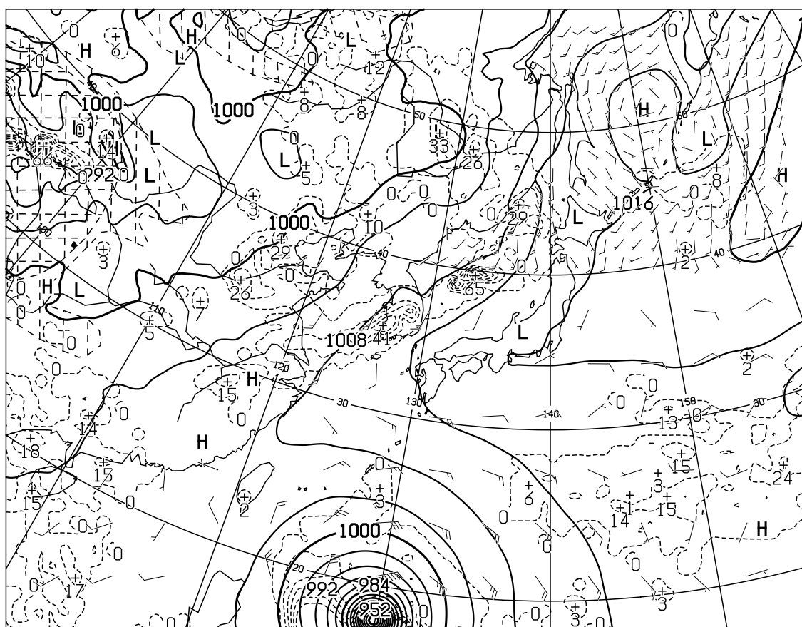
T=12 VALID 090000UTC SURFACE PRESS(hPa),PRECIP(MM) (00-12) WIND ARROW AT SURFACE
