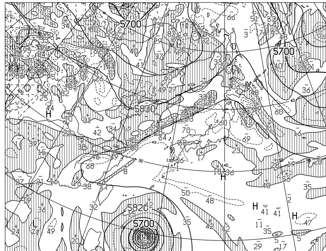
T=24 VALID 091200UTC HEIGHT(M),VORT(10 \times -6/SEC) AT 500hPa
