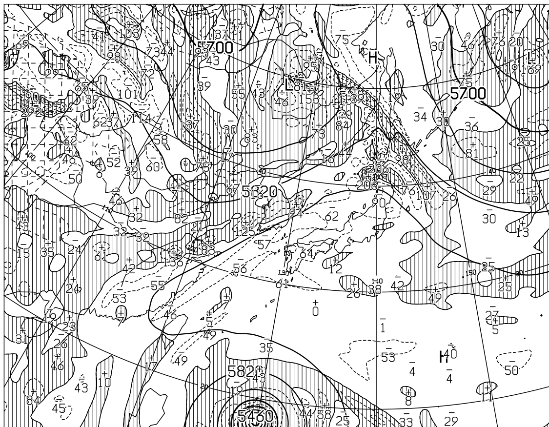
T=12 VALID 090000UTC HEIGHT(M),VORT(10 \times -6/SEC) AT 500hPa
