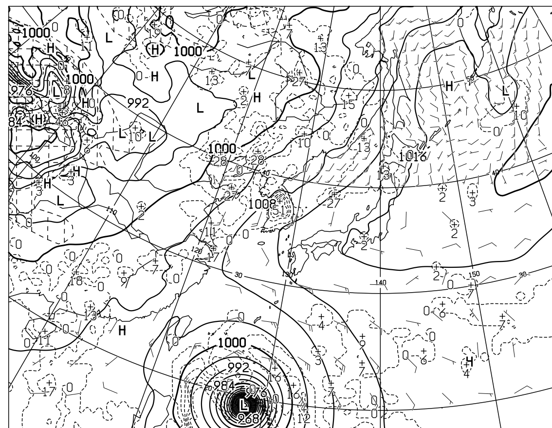
T=24 VALID 091200UTC SURFACE PRESS(hPa),PRECIP(MM) (12-24) WIND ARROW AT SURFACE
