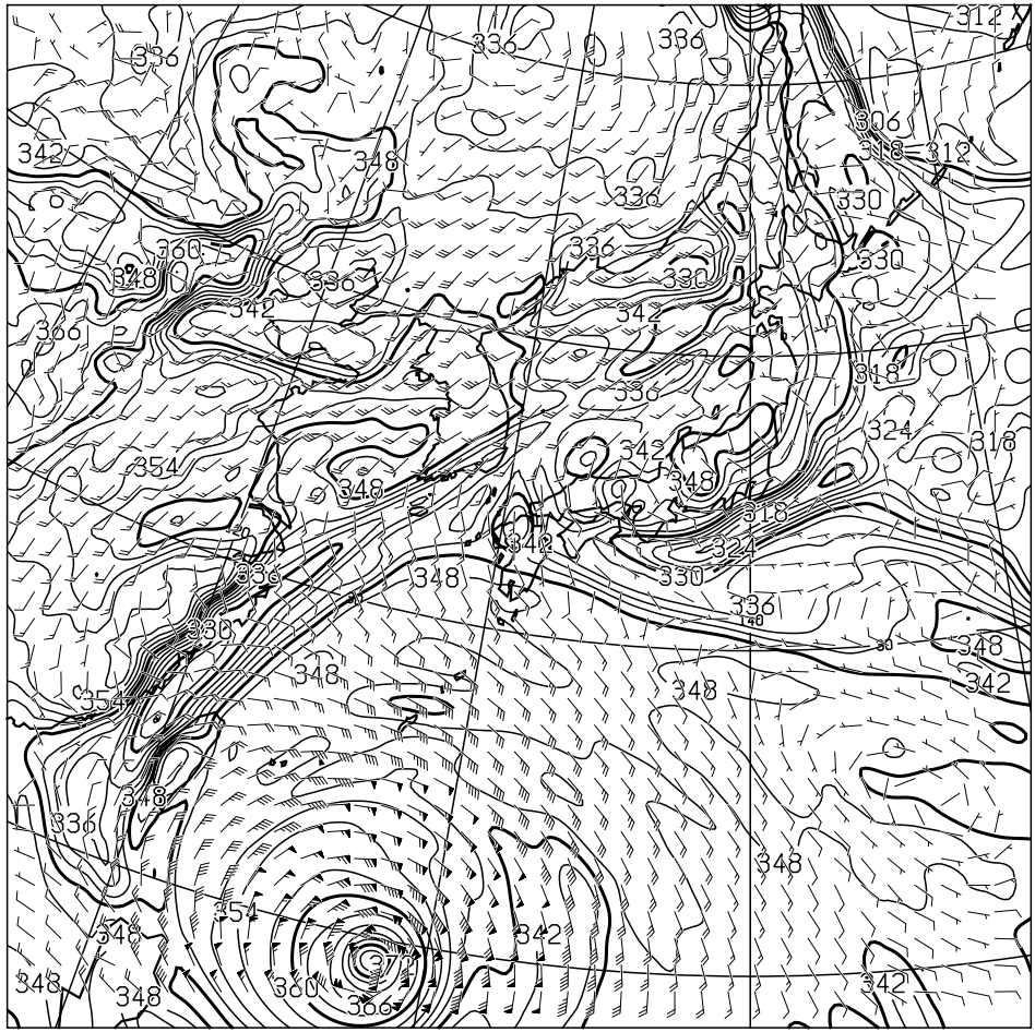
T=24 850hPa: E.P.TEMP(K),WIND(KNOTS) VALID 091200UTC
