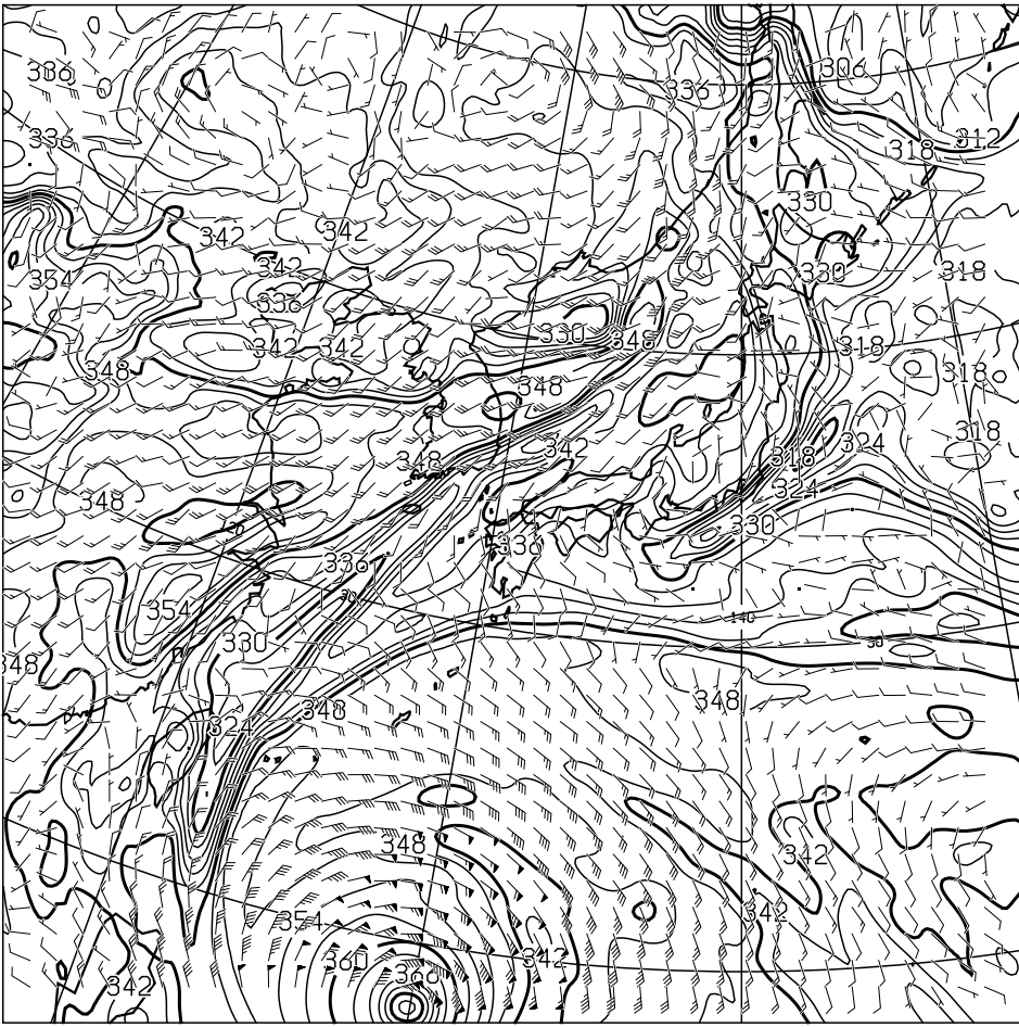
T=12 850hPa: E.P.TEMP(K),WIND(KNOTS) VALID 090000UTC
