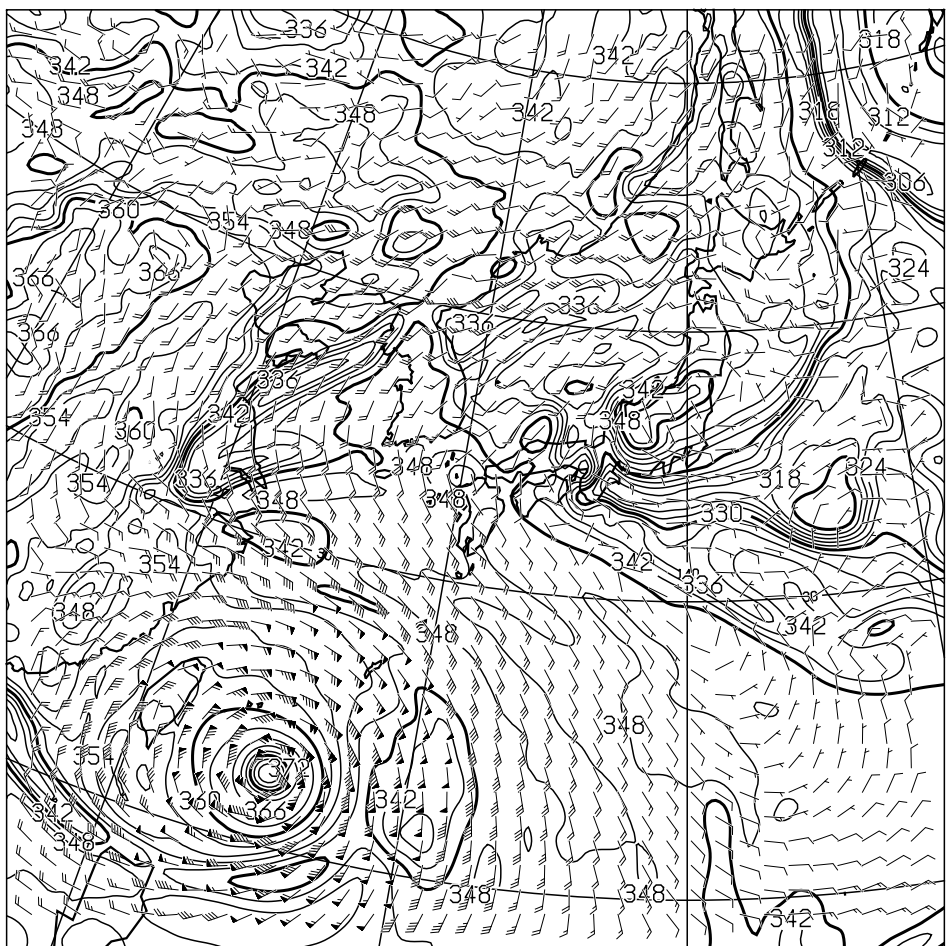
T=48 850hPa: E.P.TEMP(K),WIND(KNOTS) VALID 101200UTC
