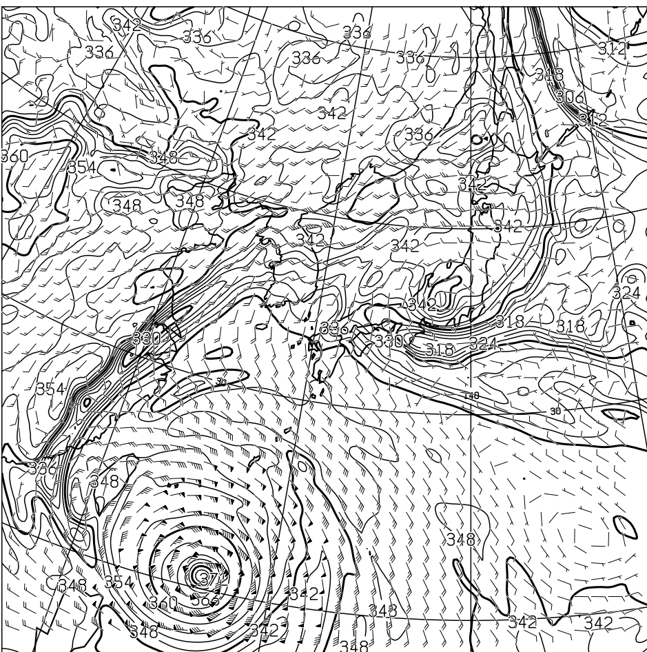
T=36 850hPa: E.P.TEMP(K),WIND(KNOTS) VALID 100000UTC
