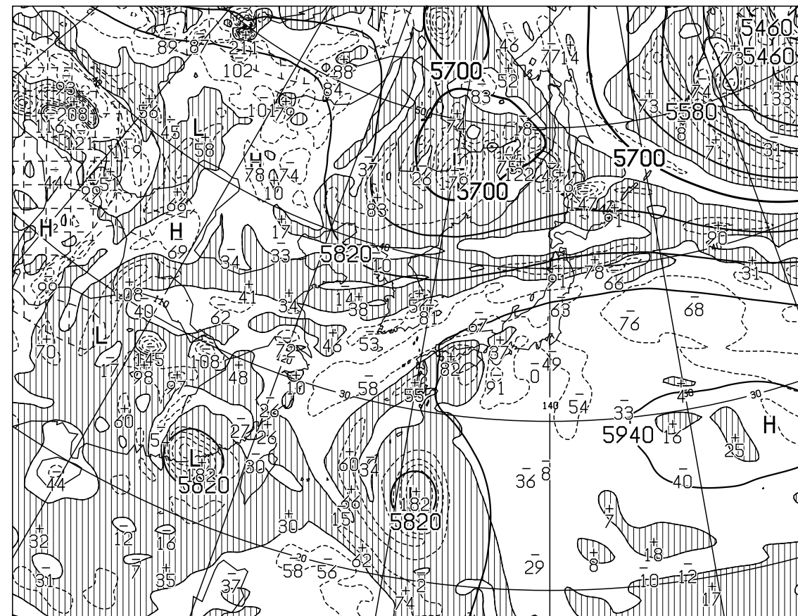
T=24 VALID 021200UTC HEIGHT(M),VORT(10 \times -6/SEC) AT 500hPa
