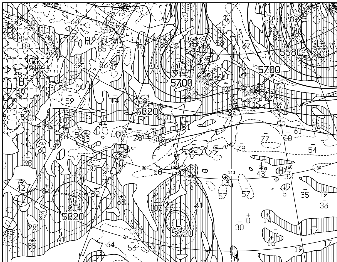
T=12 VALID 020000UTC HEIGHT(M),VORT(10 \times -6/SEC) AT 500hPa
