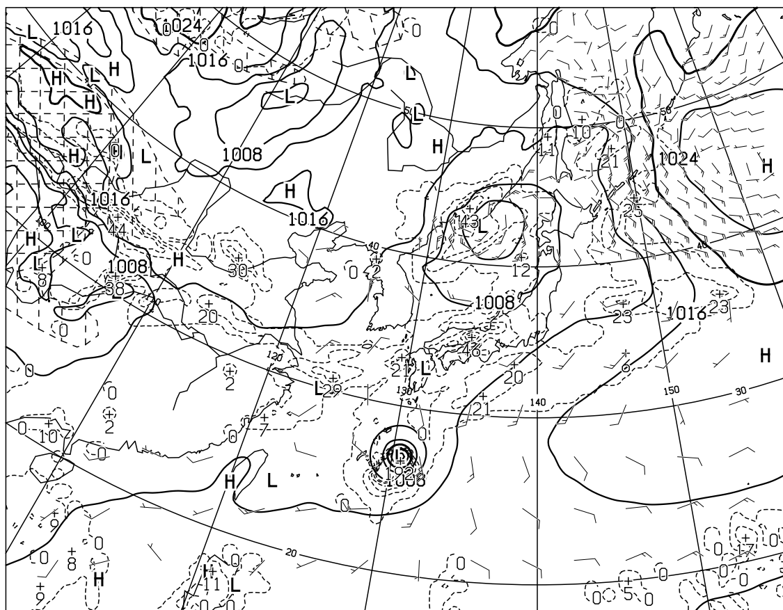
T=12 VALID 280000UTC SURFACE PRESS(hPa),PRECIP(MM) (00-12) WIND ARROW AT SURFACE
