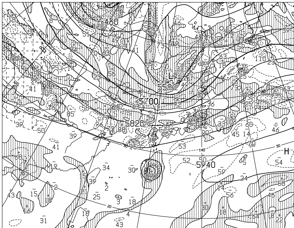
T=12 VALID 280000UTC HEIGHT(M),VORT(10 \times -6/SEC) AT 500hPa
