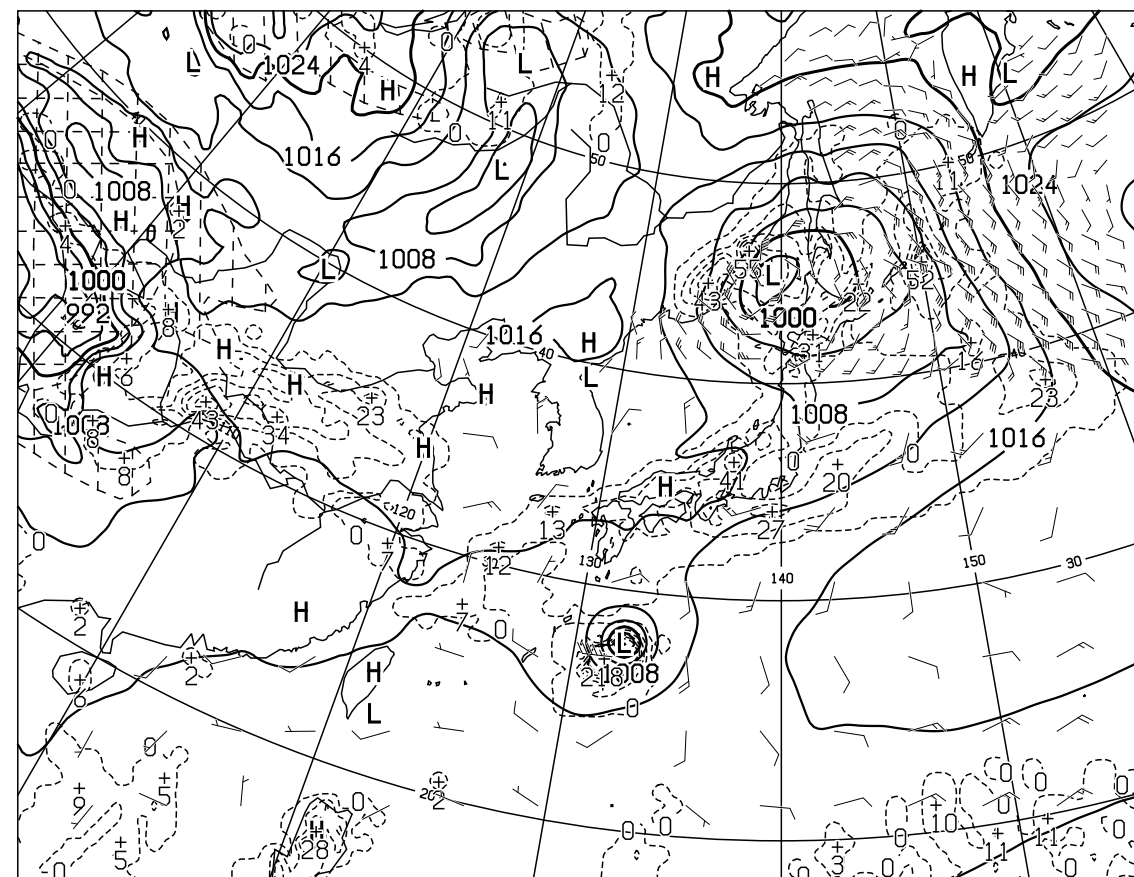
T=24 VALID 281200UTC SURFACE PRESS(hPa),PRECIP(MM) (12-24) WIND ARROW AT SURFACE
