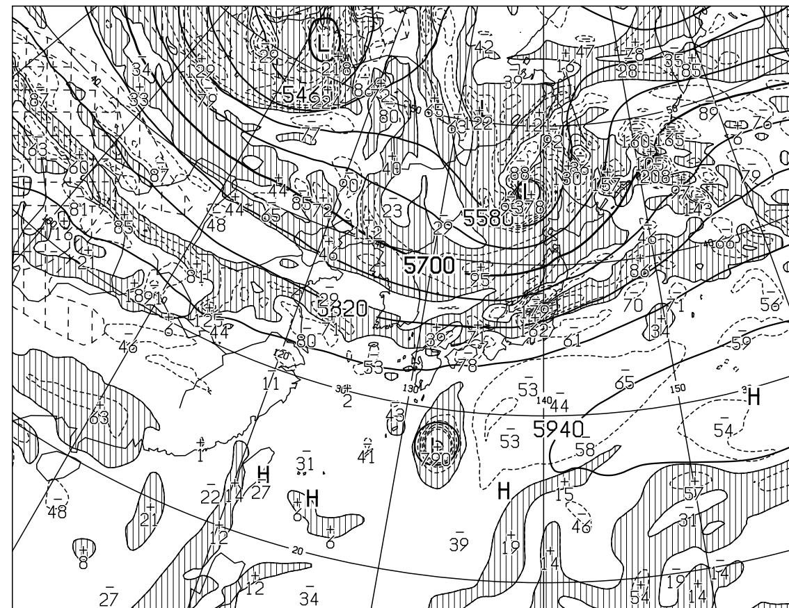
T=24 VALID 281200UTC HEIGHT(M),VORT(10 \times -6/SEC) AT 500hPa
