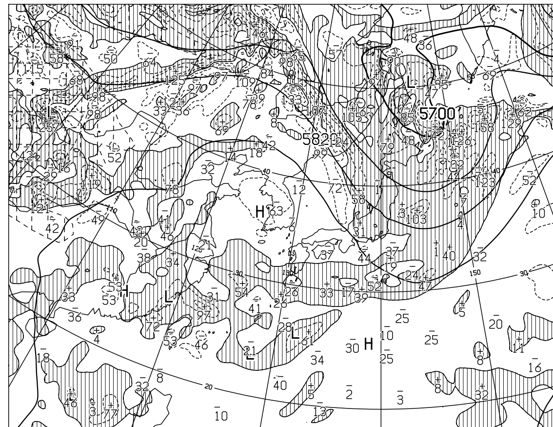
T=24 VALID 301200UTC HEIGHT(M),VORT(10 \times -6/SEC) AT 500hPa
