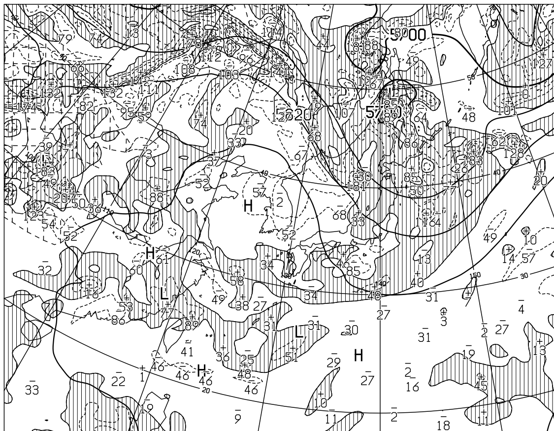
T=12 VALID 300000UTC HEIGHT(M),VORT(10 \times -6/SEC) AT 500hPa
