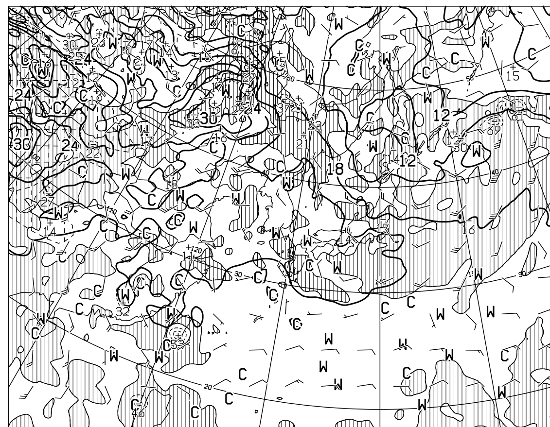
T=24 VALID 301200UTC TEMP (C), WIND ARROW AT 850hPa P-VEL (hPa/H) AT 700hPa
