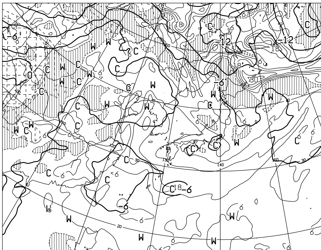
T=12 VALID 300000UTC TEMP (C) AT 500hPa T-TD (C) AT 700hPa
