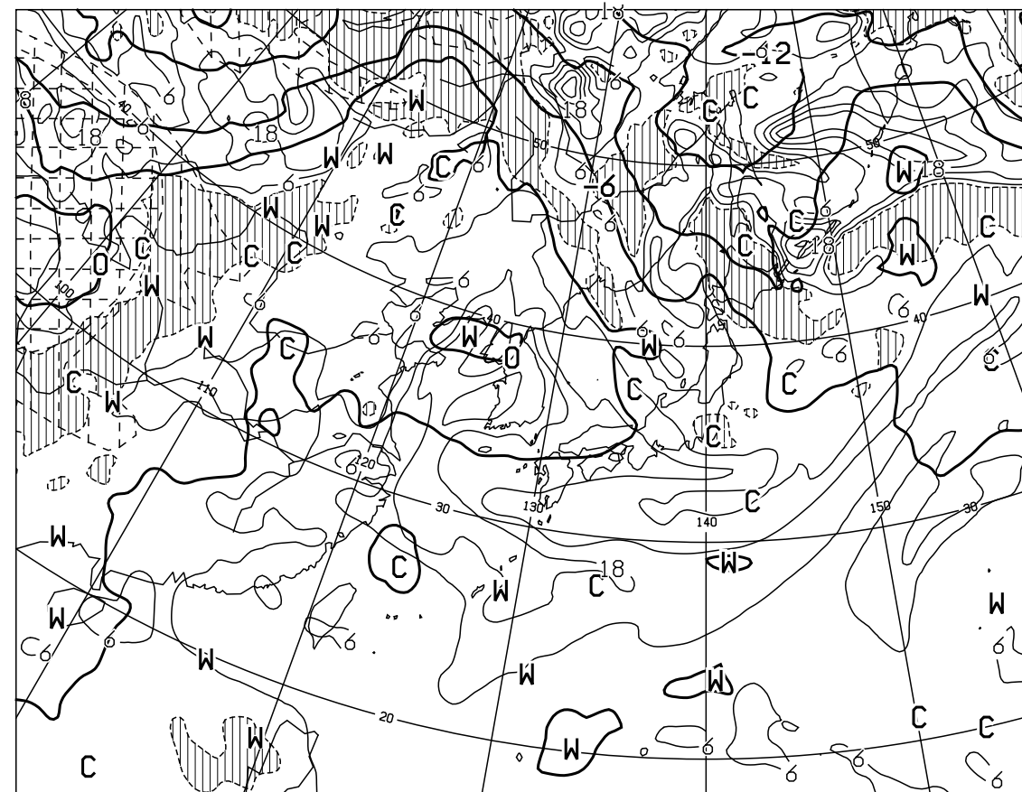
T=24 VALID 301200UTC TEMP (C) AT 500hPa T-TD (C) AT 700hPa
