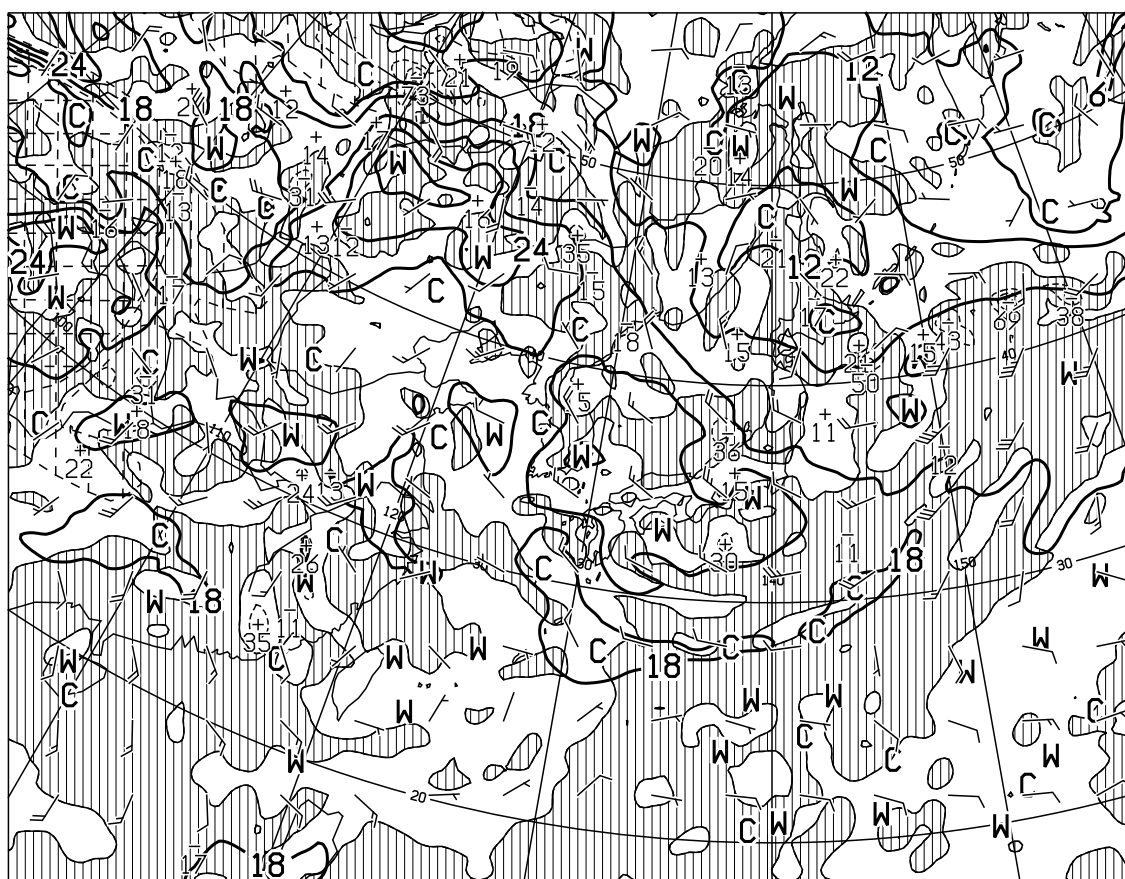
T=12 VALID 300000UTC TEMP (C), WIND ARROW AT 850hPa P-VEL (hPa/H) AT 700hPa
