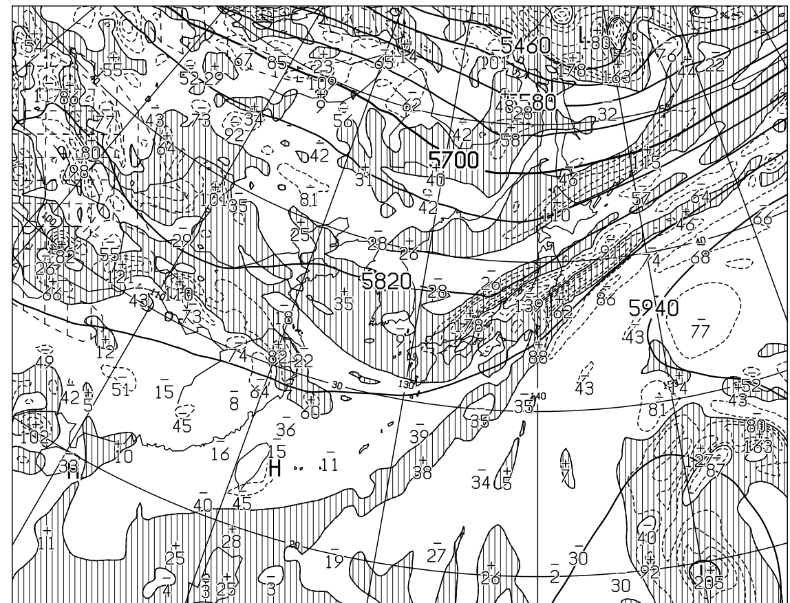
T=24 VALID 161200UTC HEIGHT(M),VORT(10 \times -6/SEC) AT 500hPa
