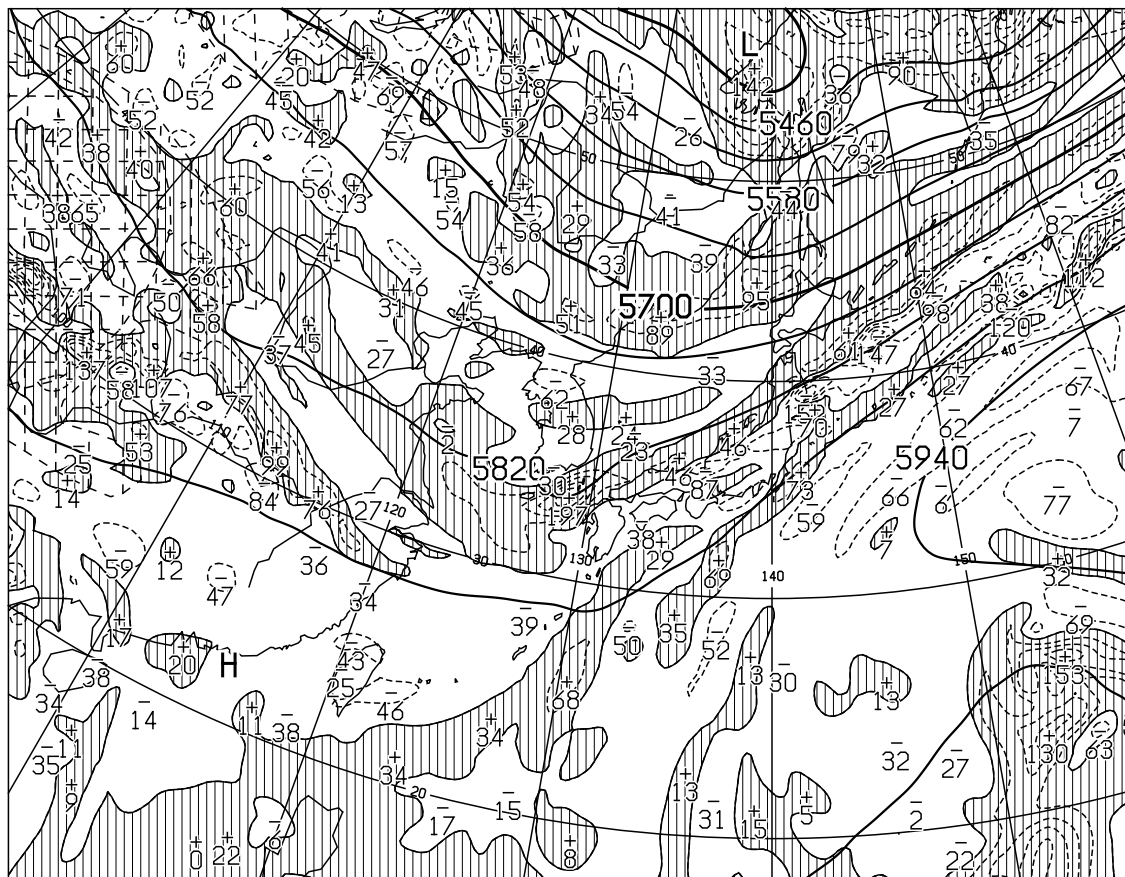
T=12 VALID 160000UTC HEIGHT(M),VORT(10 \times -6/SEC) AT 500hPa
