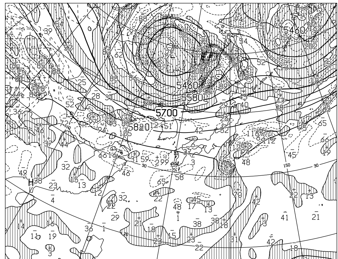
T=24 VALID 301200UTC HEIGHT(M),VORT(10**x-6/SEC) AT 500hPa
