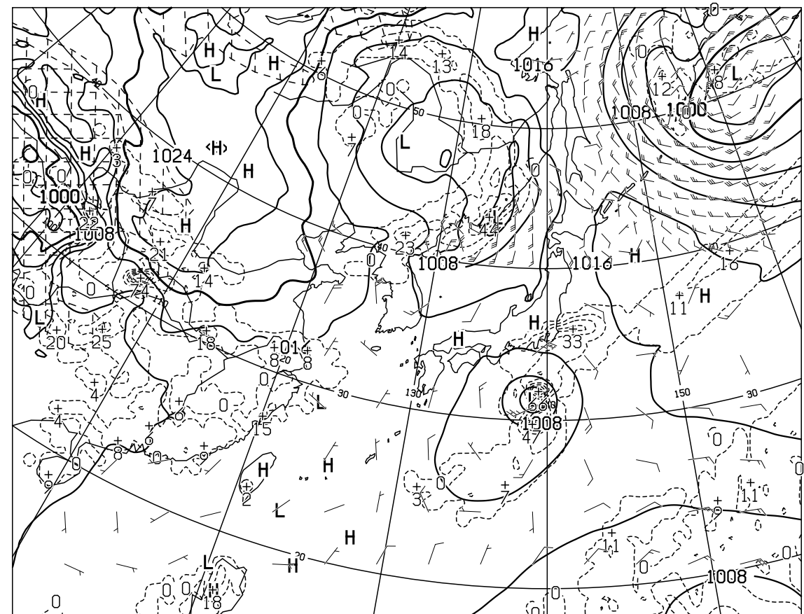
T=24 VALID 301200UTC SURFACE PRESS(hPa),PRECIP(MM) (12-24) WIND ARROW AT SURFACE
