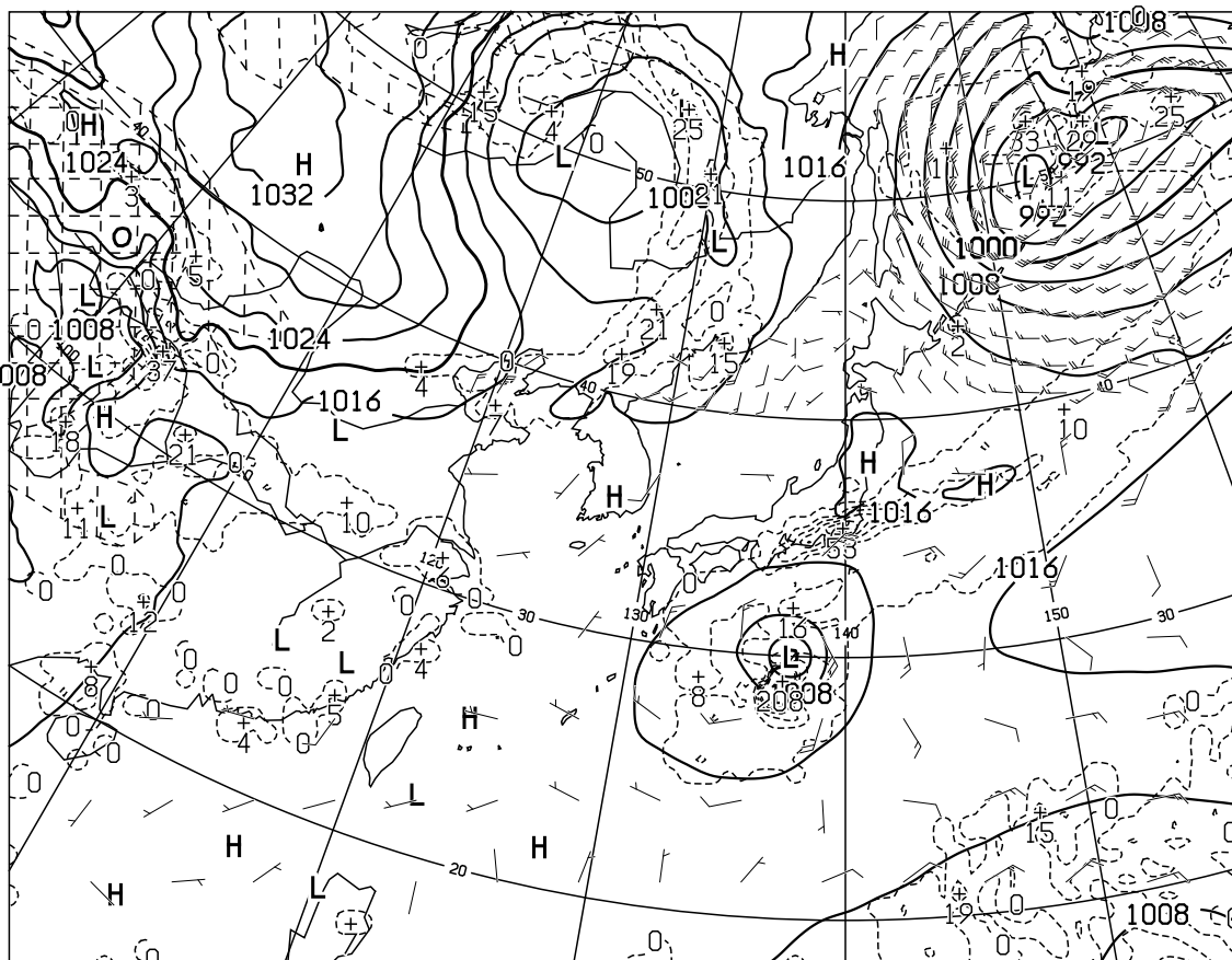
T=12 VALID 300000UTC SURFACE PRESS(hPa),PRECIP(MM) (00-12) WIND ARROW AT SURFACE
