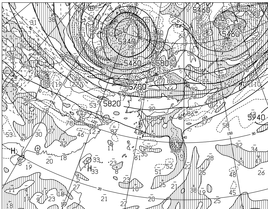
T=12 VALID 300000UTC HEIGHT(M),VORT(10**x-6/SEC) AT 500hPa
