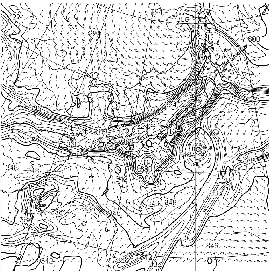
T=36 850hPa: E.P.TEMP(K),WIND(KNOTS) VALID 010000UTC
