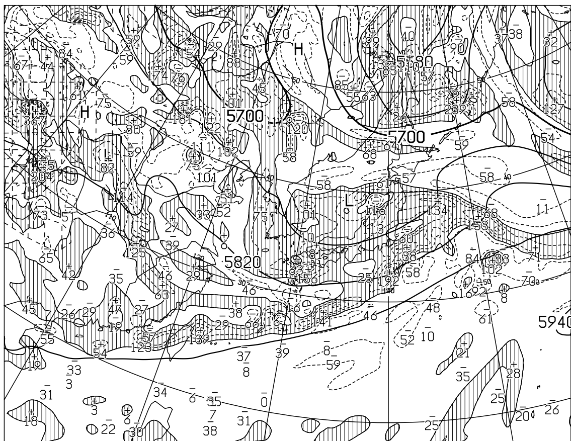
T=12 VALID 150000UTC HEIGHT(M),VORT(10 \times -6/SEC) AT 500hPa
