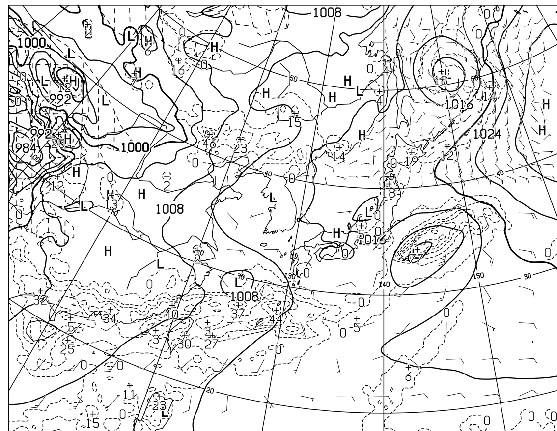
T=24 VALID 151200UTC SURFACE PRESS(hPa),PRECIP(MM) (12-24) WIND ARROW AT SURFACE
