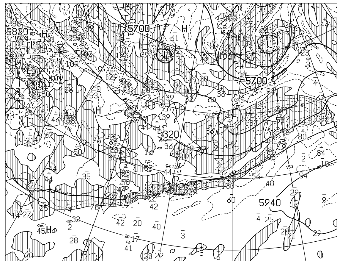
T=24 VALID 151200UTC HEIGHT(M),VORT(10 \times -6/SEC) AT 500hPa
