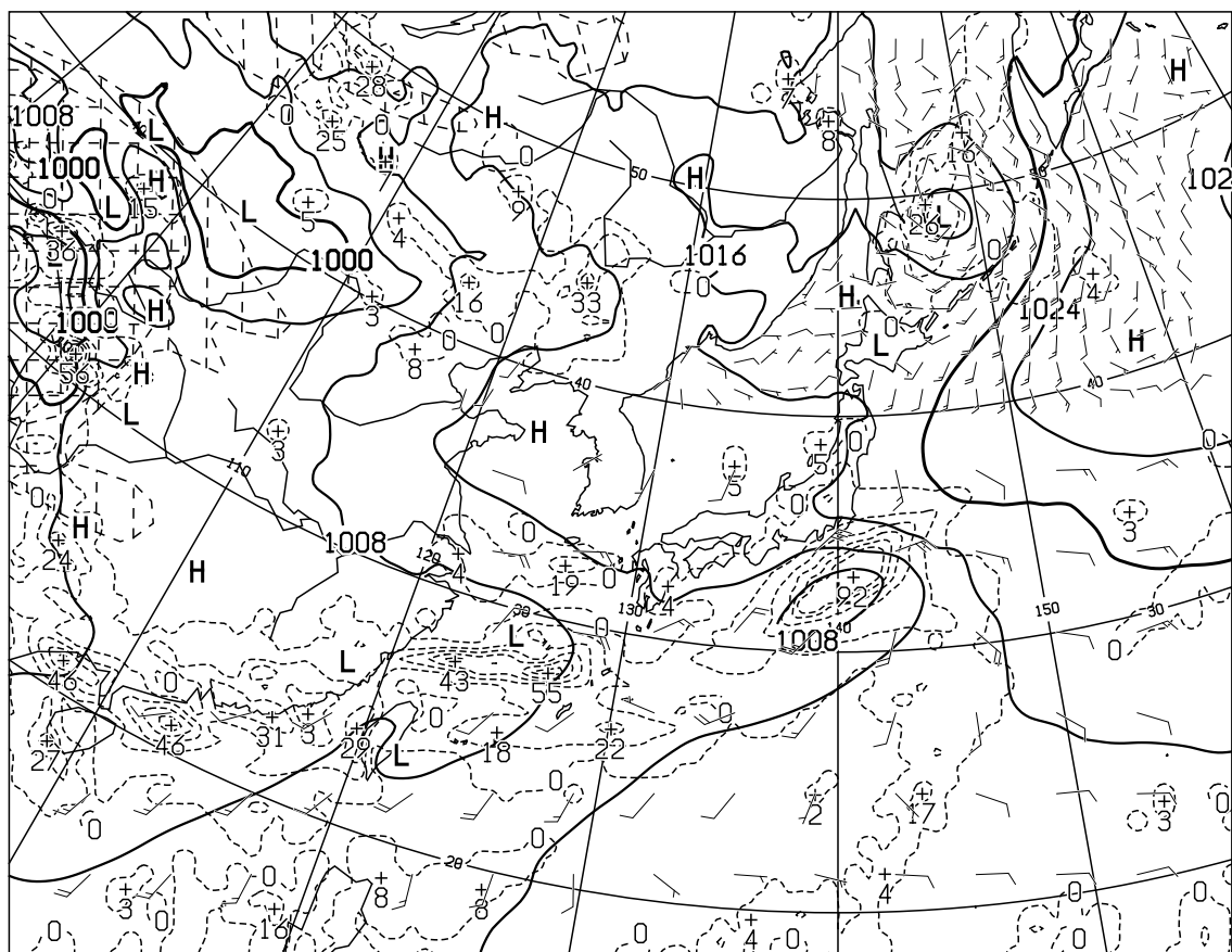
T=12 VALID 150000UTC SURFACE PRESS(hPa),PRECIP(MM) (00-12) WIND ARROW AT SURFACE
