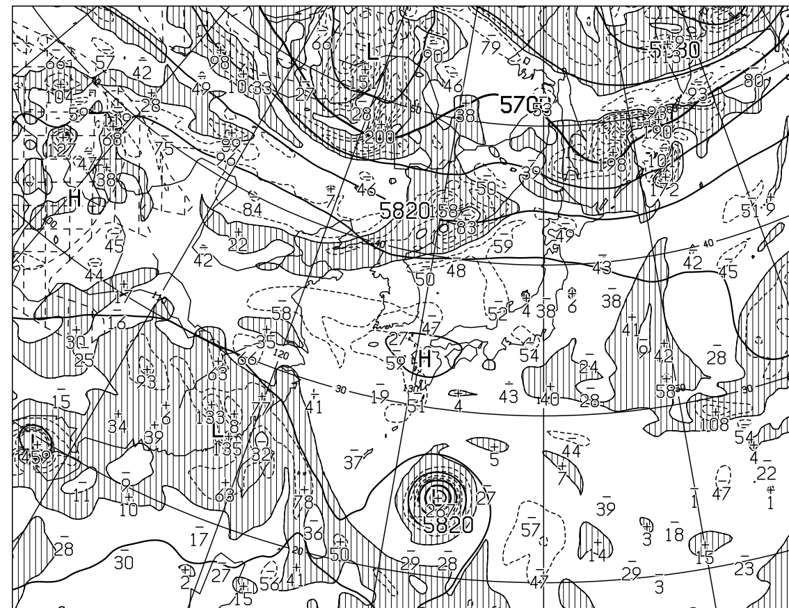
T=24 VALID 241200UTC HEIGHT(M),VORT(10 \times -6/SEC) AT 500hPa
