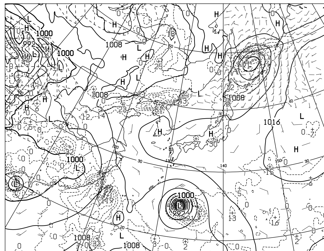
T=24 VALID 241200UTC SURFACE PRESS(hPa),PRECIP(MM) (12-24) WIND ARROW AT SURFACE
