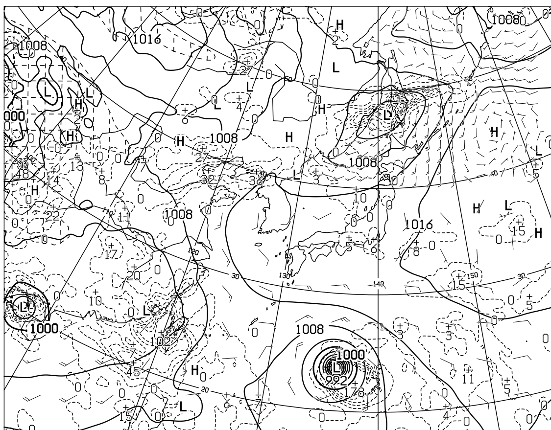
T=12 VALID 240000UTC SURFACE PRESS(hPa),PRECIP(MM) (00-12) WIND ARROW AT SURFACE
