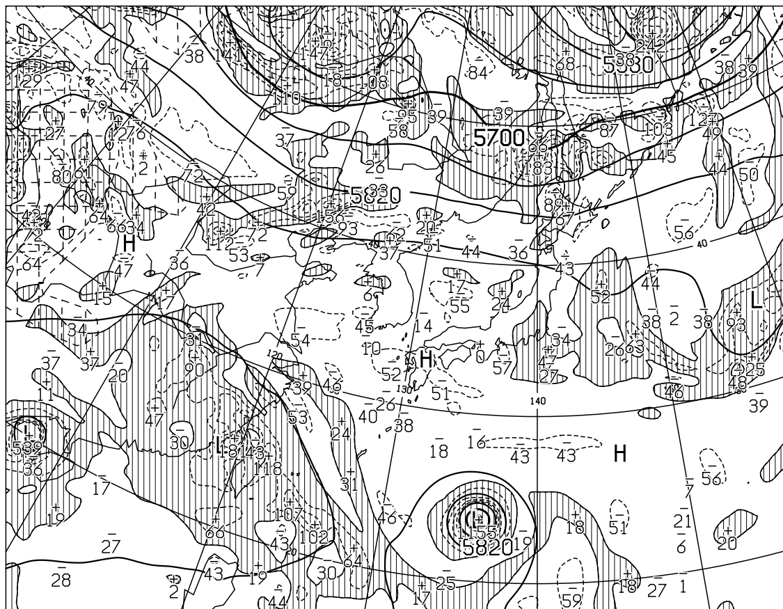
T=12 VALID 240000UTC HEIGHT(M),VORT(10 \times -6/SEC) AT 500hPa
