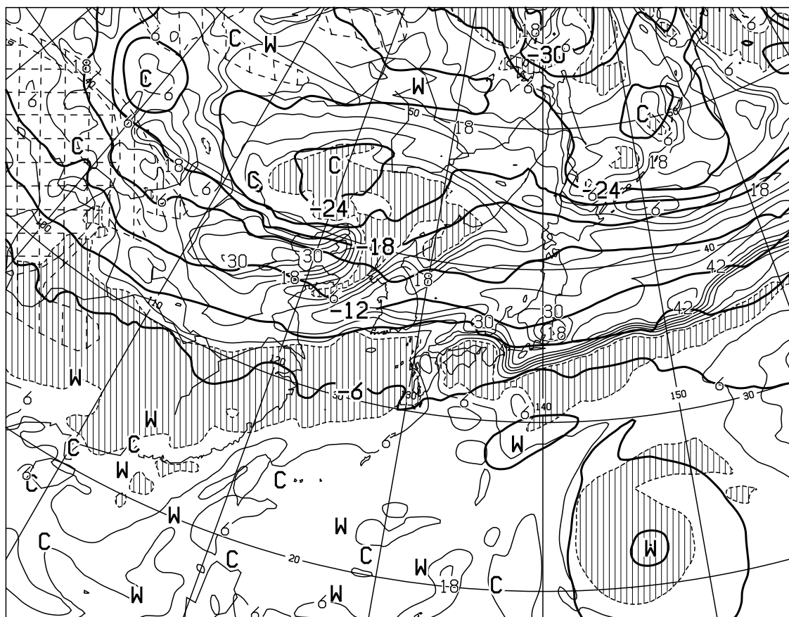
T=12 VALID 040000UTC TEMP ( C ) AT 500hPa T-TD ( C ) AT 700hPa
