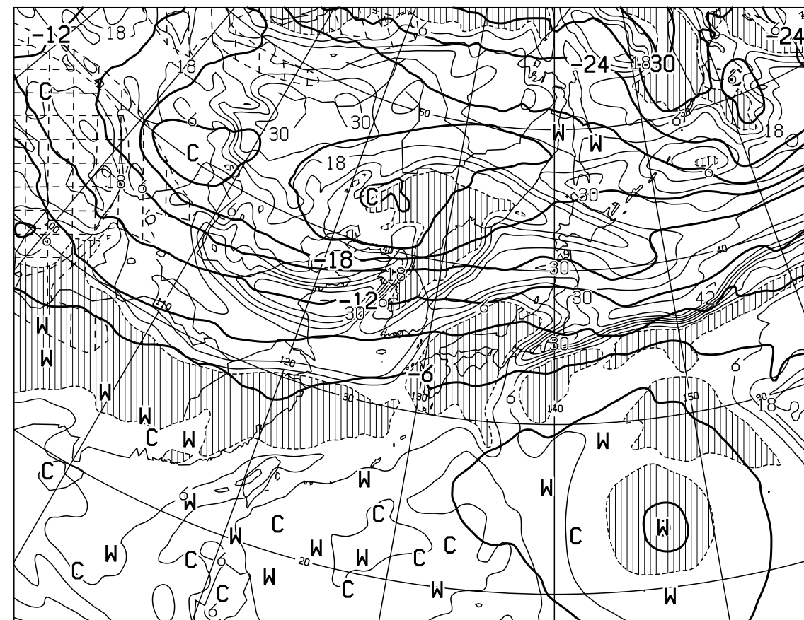
T=24 VALID 041200UTC TEMP ( C ) AT 500hPa T-TD ( C ) AT 700hPa
