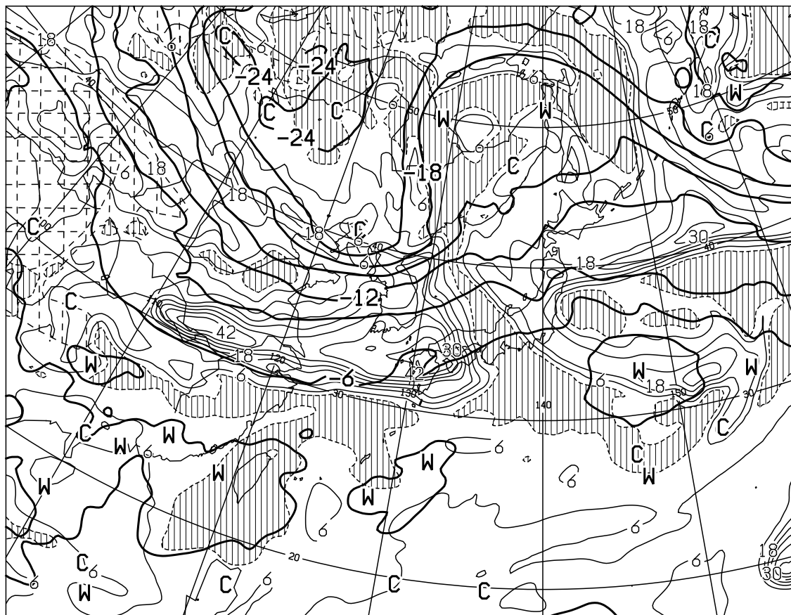
T=12 VALID 050000UTC TEMP (C) AT 500hPa T-TD (C) AT 700hPa
