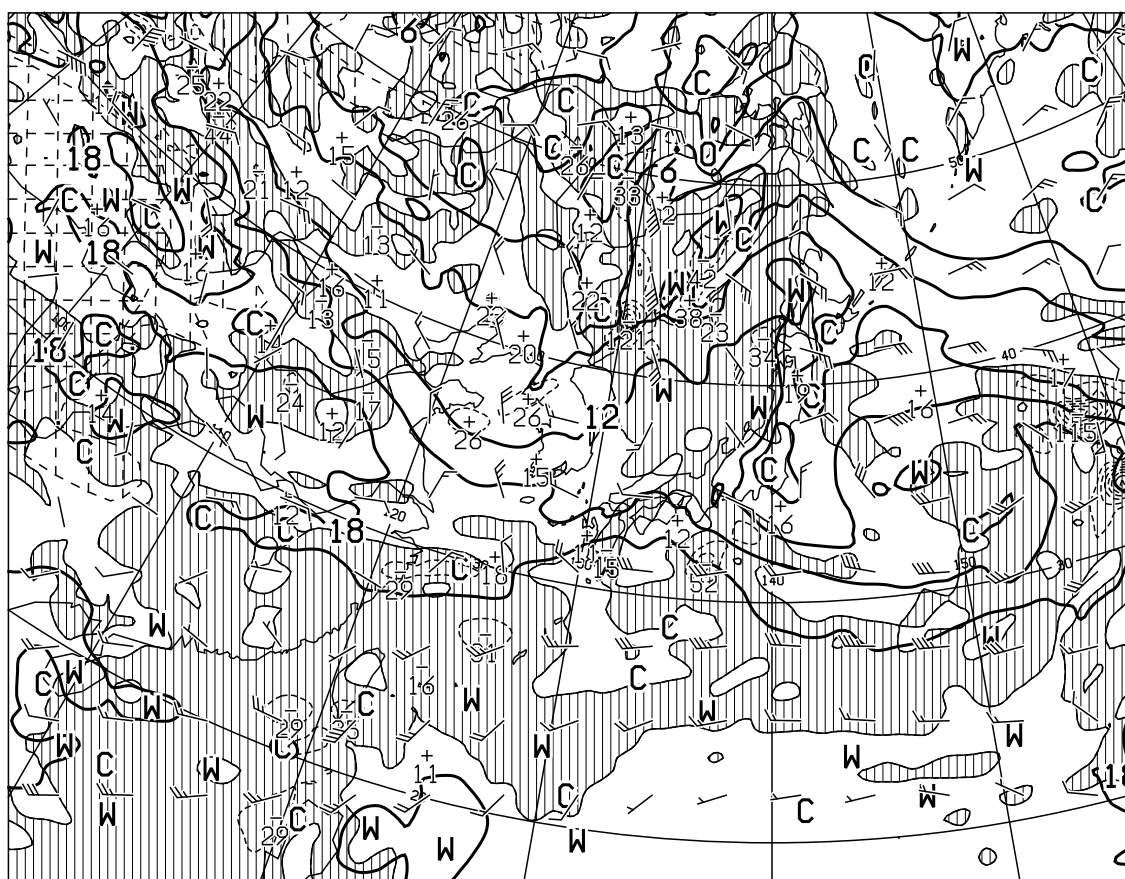
T=12 VALID 050000UTC TEMP (C), WIND ARROW AT 850hPa P-VEL (hPa/H) AT 700hPa
