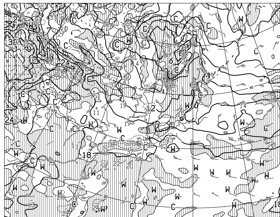
T=24 VALID 051200UTC TEMP (C), WIND ARROW AT 850hPa P-VEL (hPa/H) AT 700hPa
