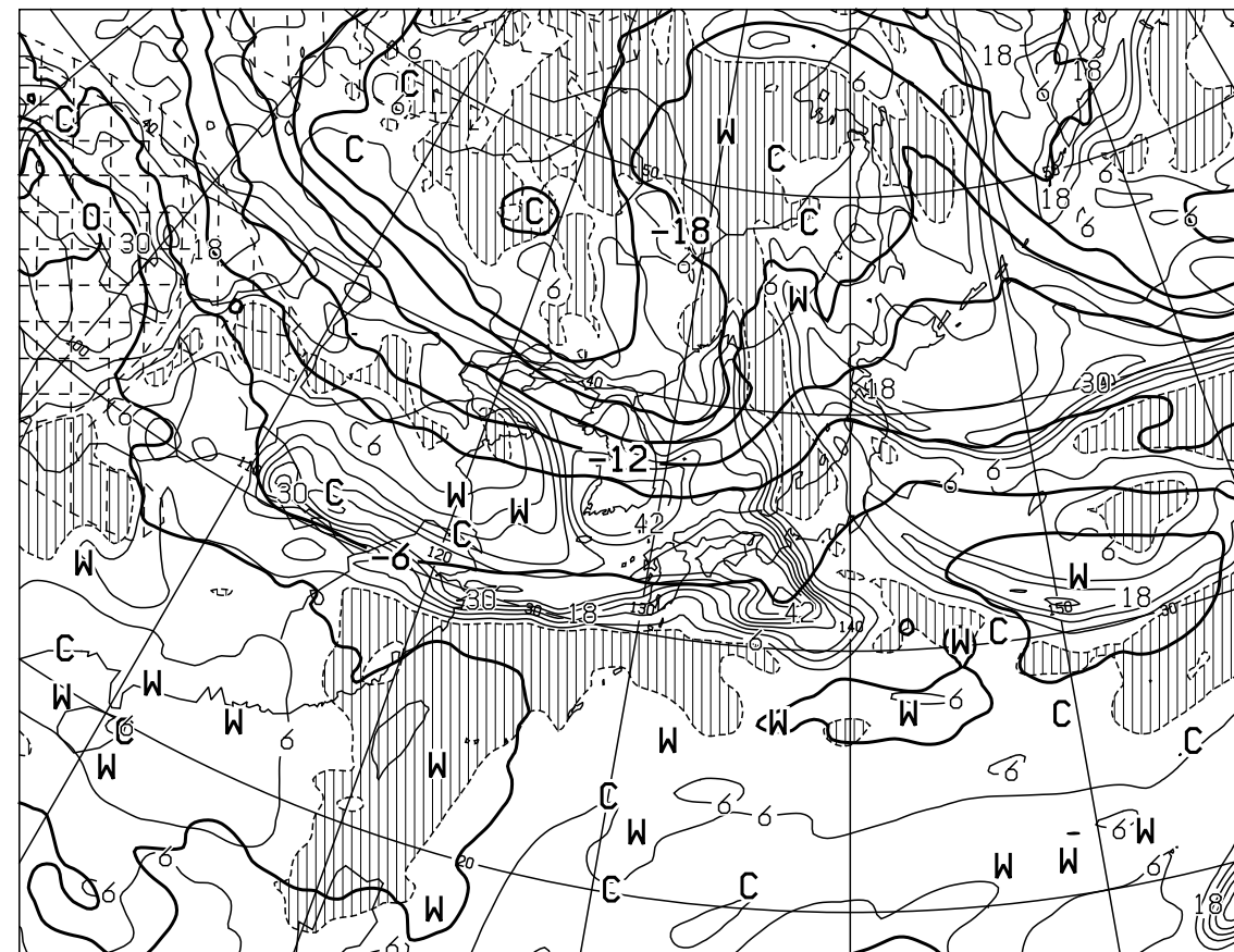
T=24 VALID 051200UTC TEMP (C) AT 500hPa T-TD (C) AT 700hPa
