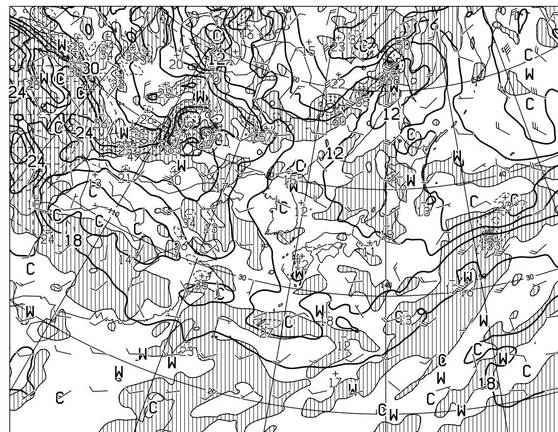
T=24 VALID 121200UTC TEMP (C), WIND ARROW AT 850hPa P-VEL (hPa/H) AT 700hPa
