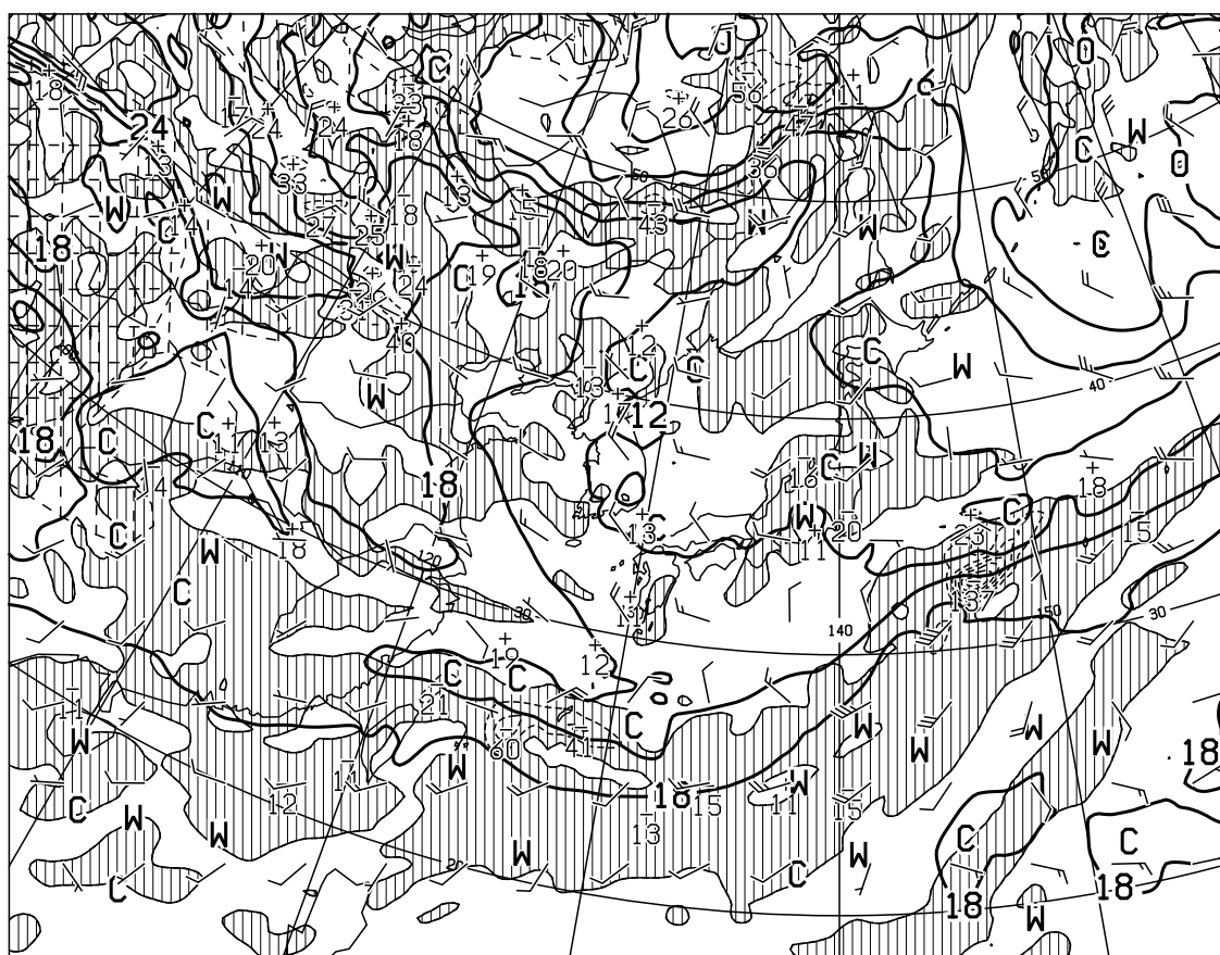
T=12 VALID 120000UTC TEMP (C), WIND ARROW AT 850hPa P-VEL (hPa/H) AT 700hPa
