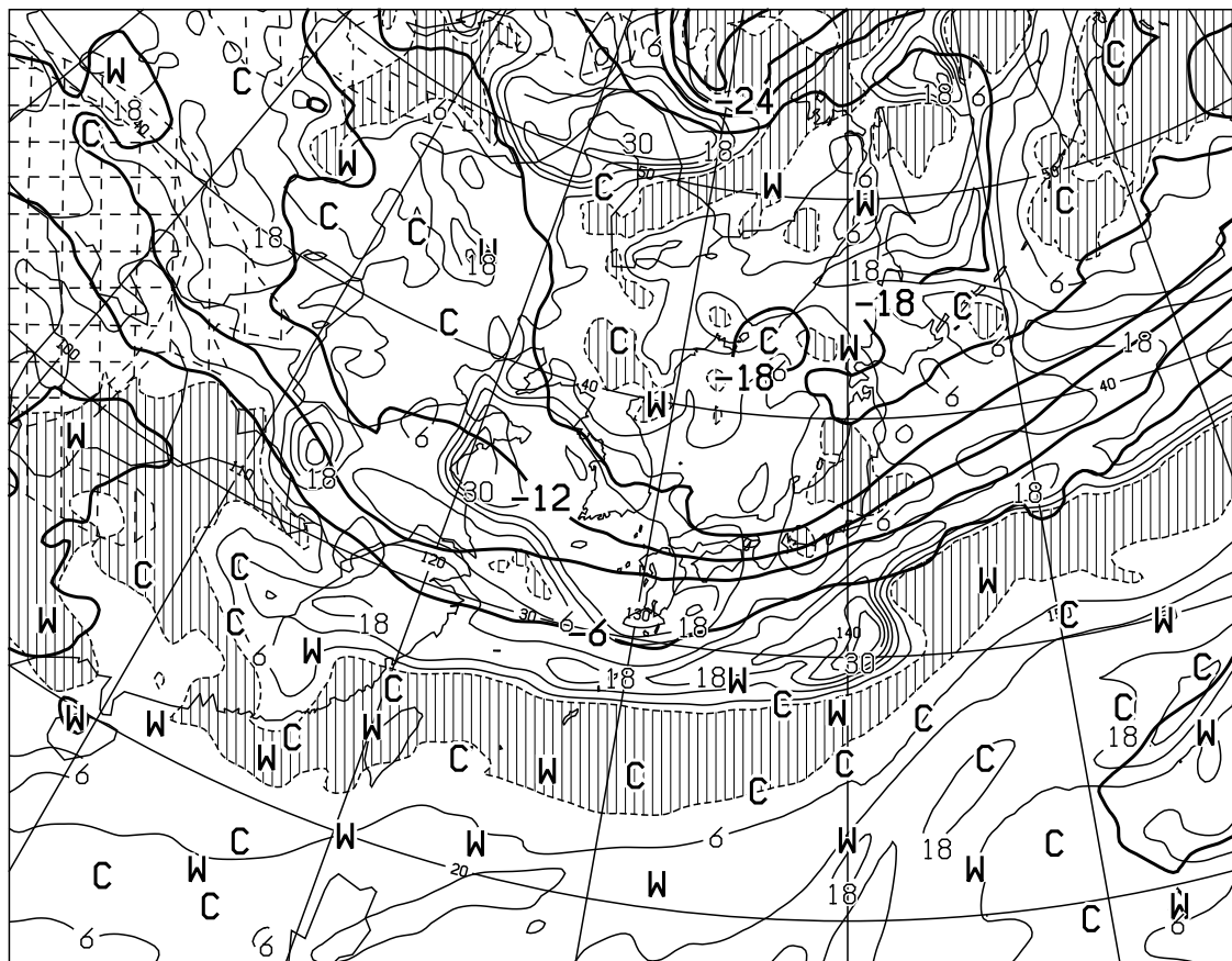
T=12 VALID 120000UTC TEMP (C) AT 500hPa T-TD (C) AT 700hPa
