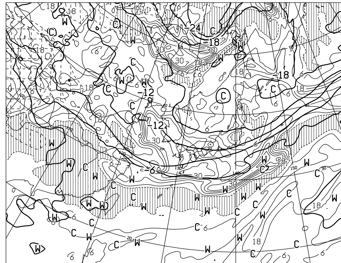
T=24 VALID 121200UTC TEMP (C) AT 500hPa T-TD (C) AT 700hPa
