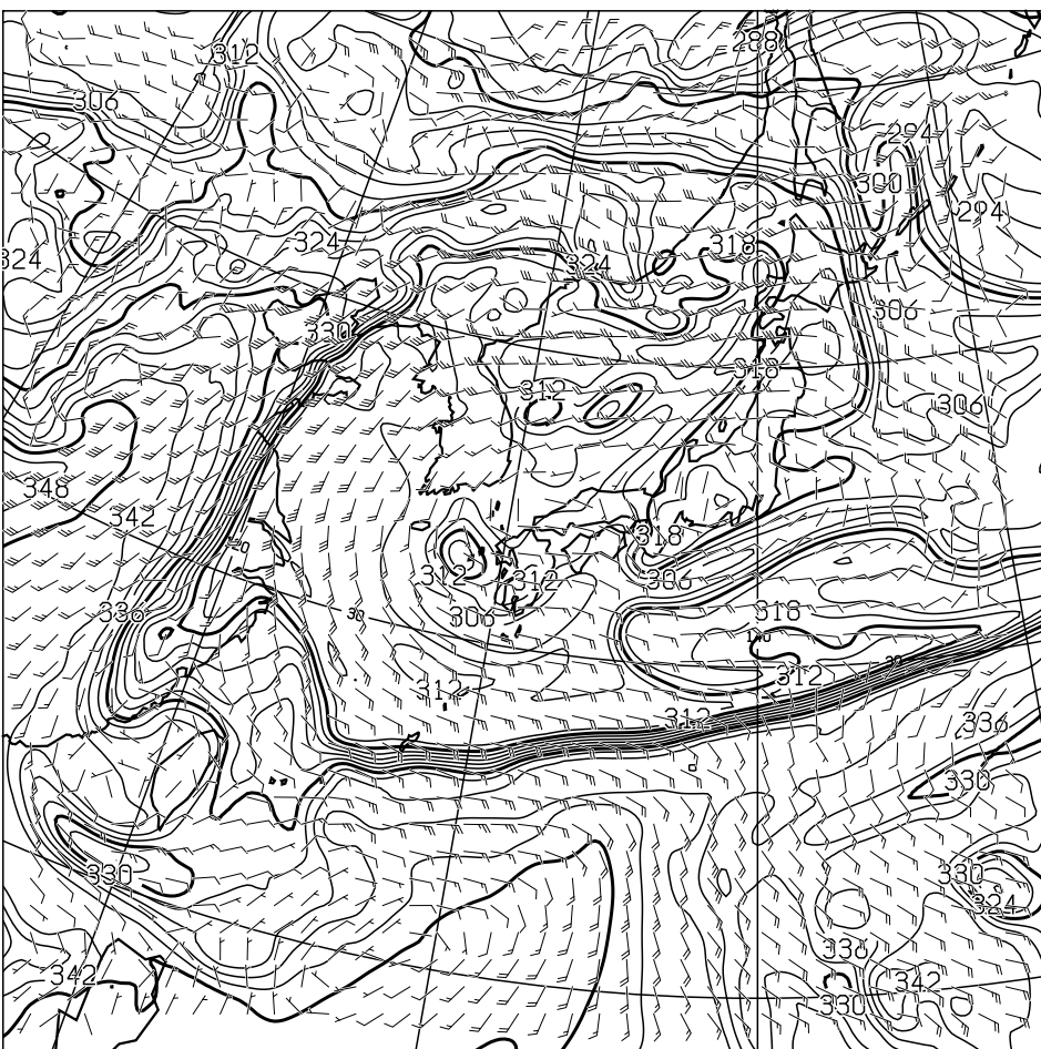
T=36 850hPa: E.P.TEMP(K),WIND(KNOTS) VALID 180000UTC
