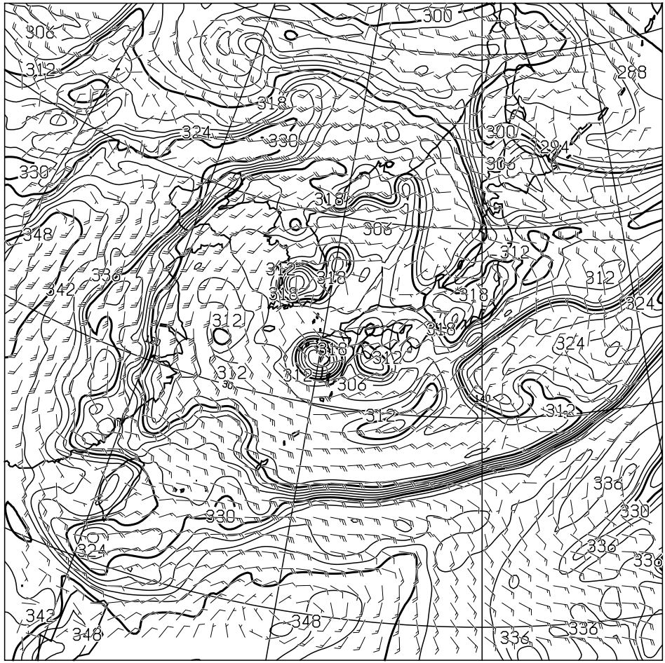
T=24 850hPa: E.P.TEMP(K),WIND(KNOTS) VALID 171200UTC
