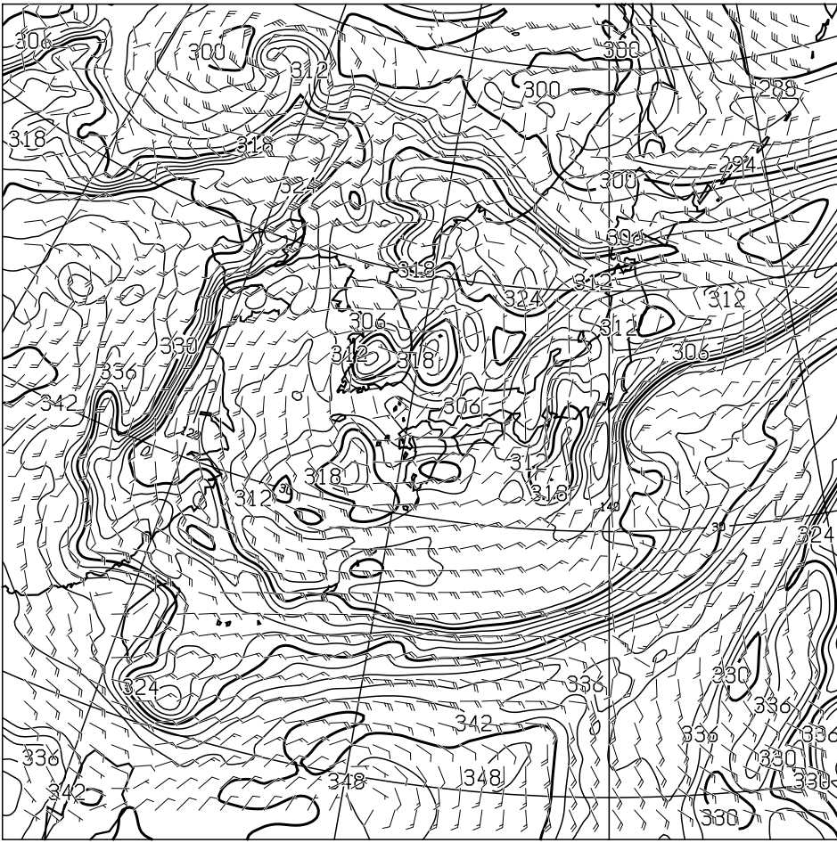
T=12 850hPa: E.P.TEMP(K),WIND(KNOTS) VALID 170000UTC
