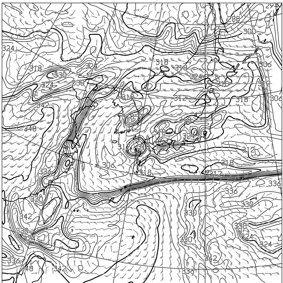
T=48 850hPa: E.P.TEMP(K),WIND(KNOTS) VALID 181200UTC
