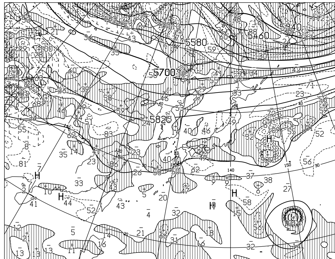
T=24 VALID 101200UTC HEIGHT(M),VORT(10**x-6/SEC) AT 500hPa
