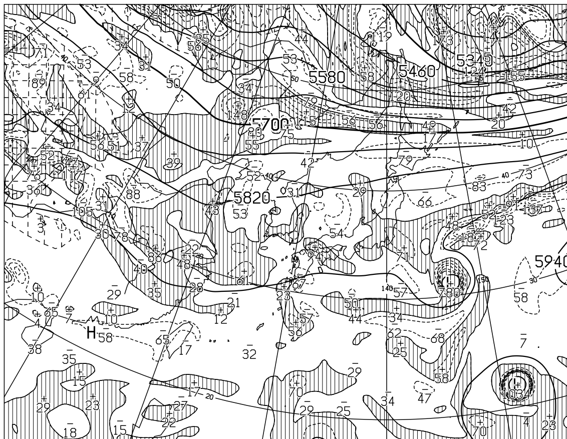
T=12 VALID 100000UTC HEIGHT(M),VORT(10**x-6/SEC) AT 500hPa
