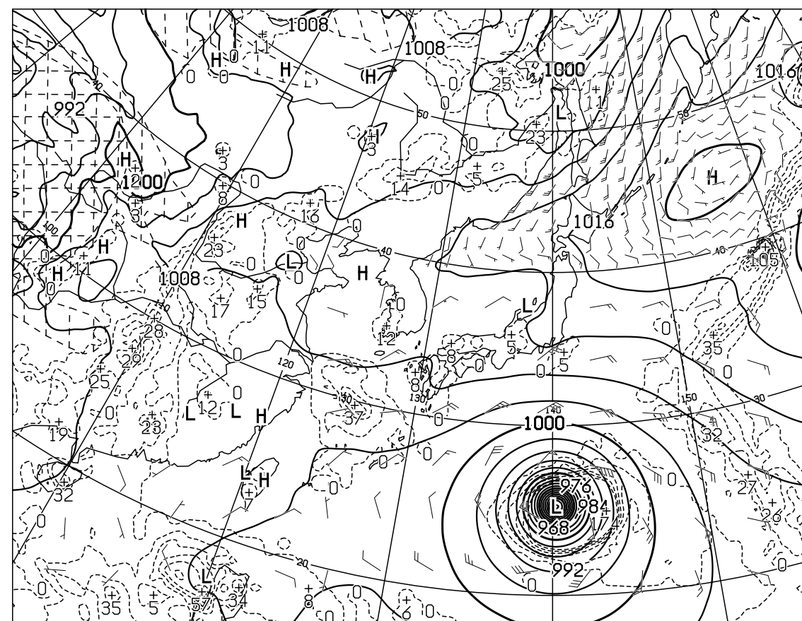
T=24 VALID 041200UTC SURFACE PRESS(hPa),PRECIP(MM) (12-24) WIND ARROW AT SURFACE
