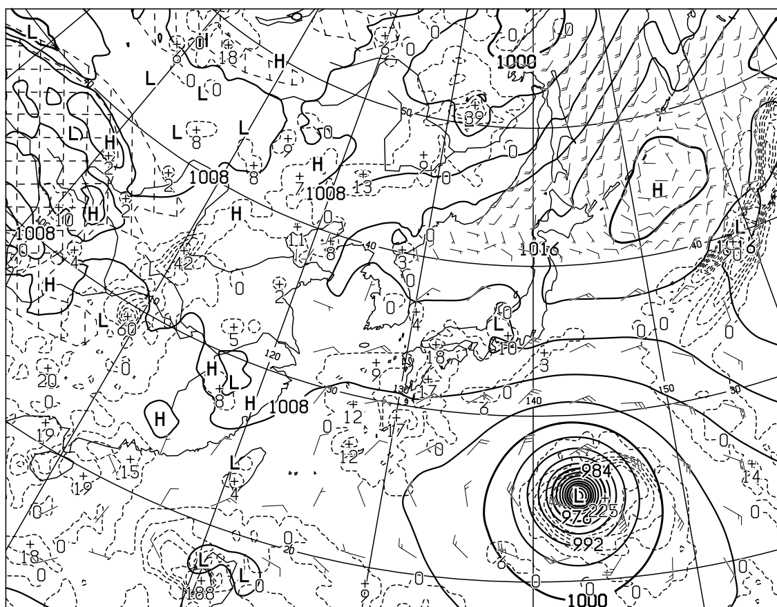
T=12 VALID 040000UTC SURFACE PRESS(hPa),PRECIP(MM) (00-12) WIND ARROW AT SURFACE
