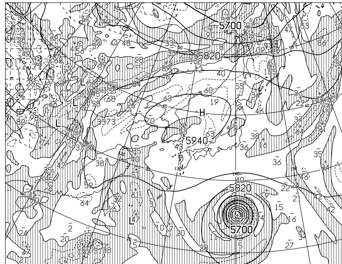
T=24 VALID 041200UTC HEIGHT(M),VORT(10 \times -6/SEC) AT 500hPa
