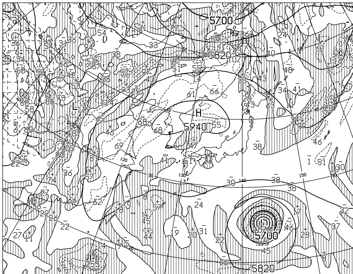
T=12 VALID 040000UTC HEIGHT(M),VORT(10 \times -6/SEC) AT 500hPa
