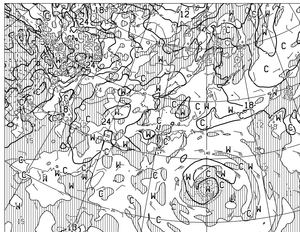
T=24 VALID 041200UTC TEMP (C), WIND ARROW AT 850hPa P-VEL (hPa/H) AT 700hPa
