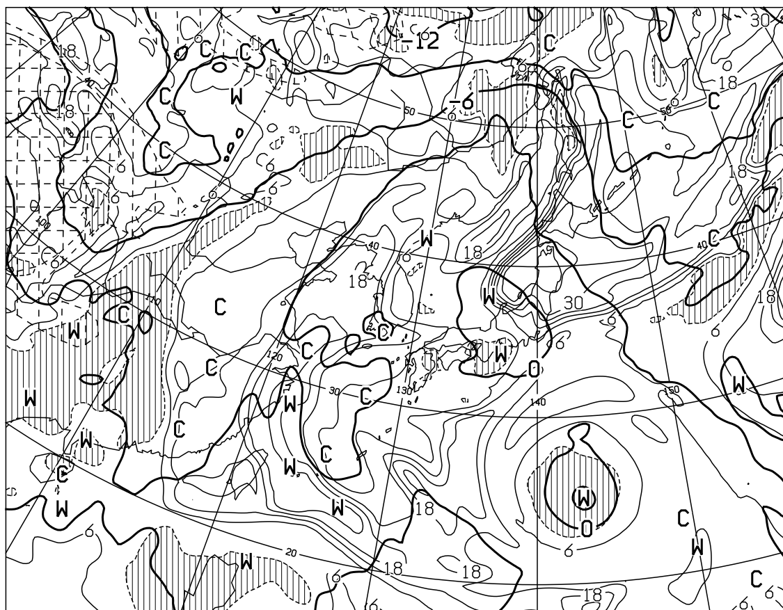
T=12 VALID 040000UTC TEMP (C) AT 500hPa T-D (C) AT 700hPa
