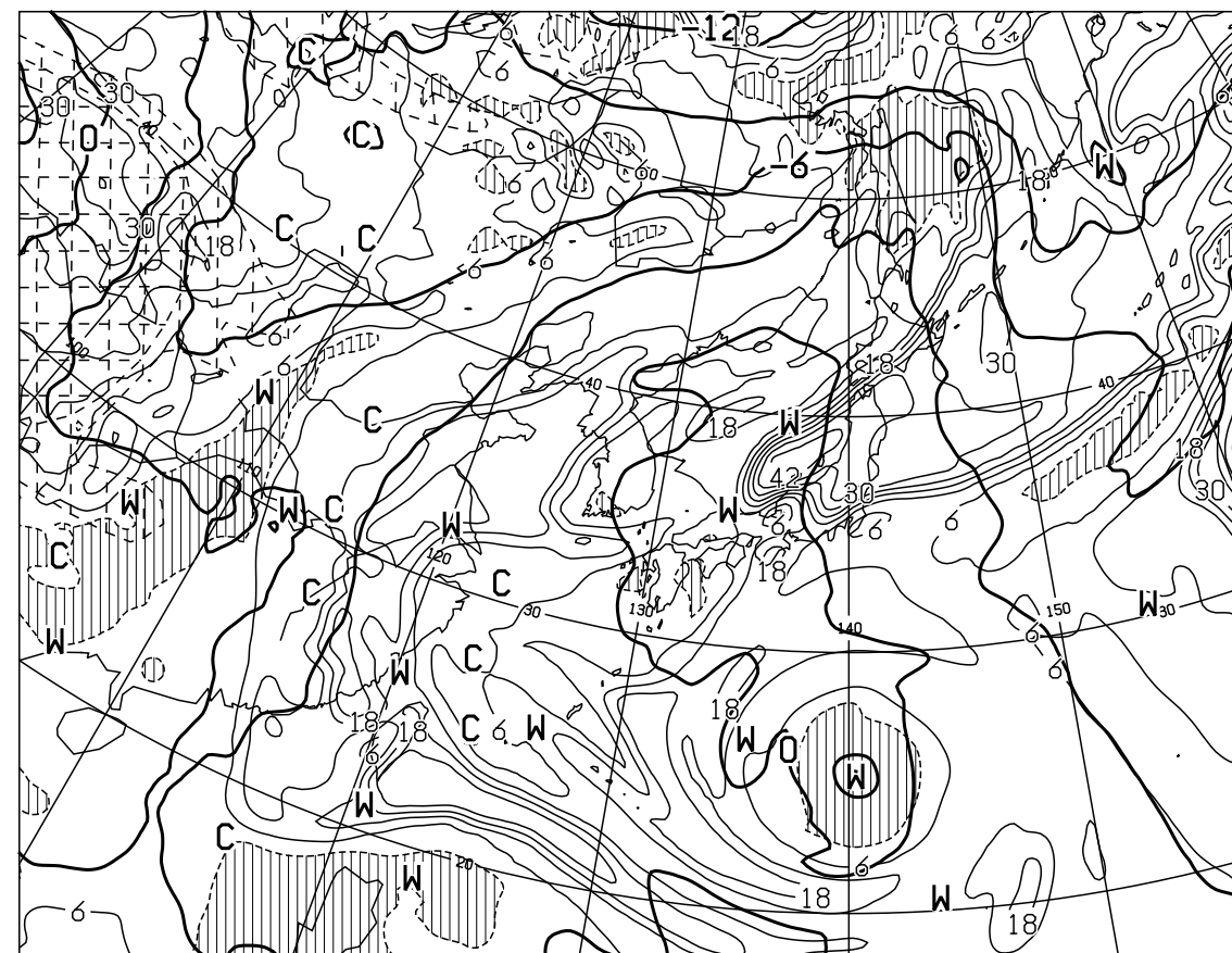
T=24 VALID 041200UTC TEMP (C) AT 500hPa T-D (C) AT 700hPa
