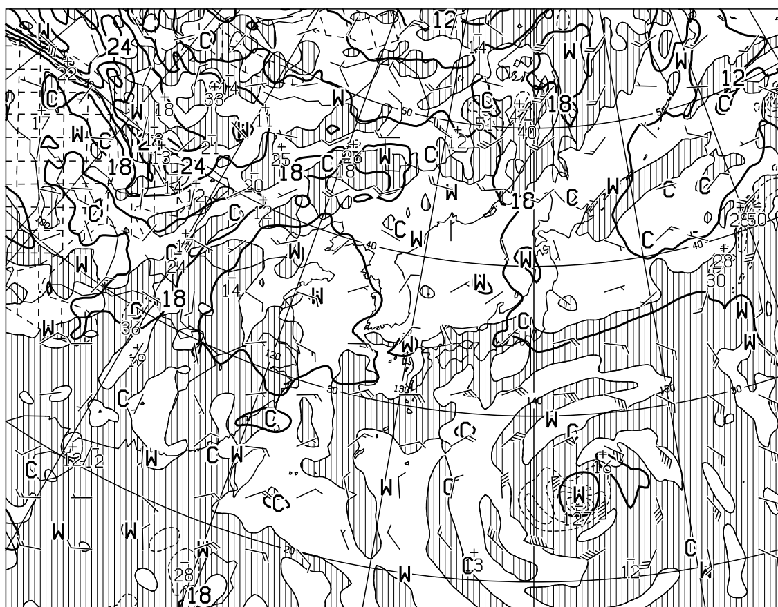
T=12 VALID 040000UTC TEMP (C), WIND ARROW AT 850hPa P-VEL (hPa/H) AT 700hPa
