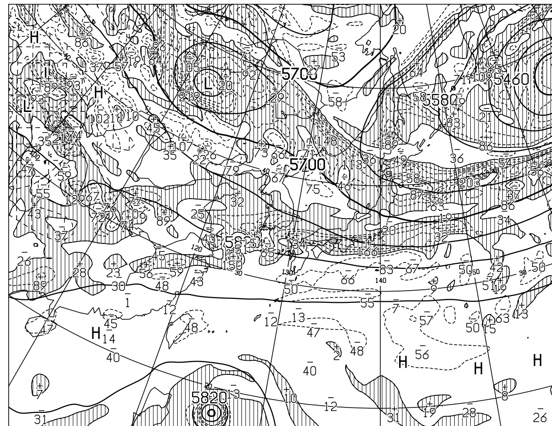
T=24 VALID 221200UTC HEIGHT(M),VORT(10 \times -6/SEC) AT 500hPa
