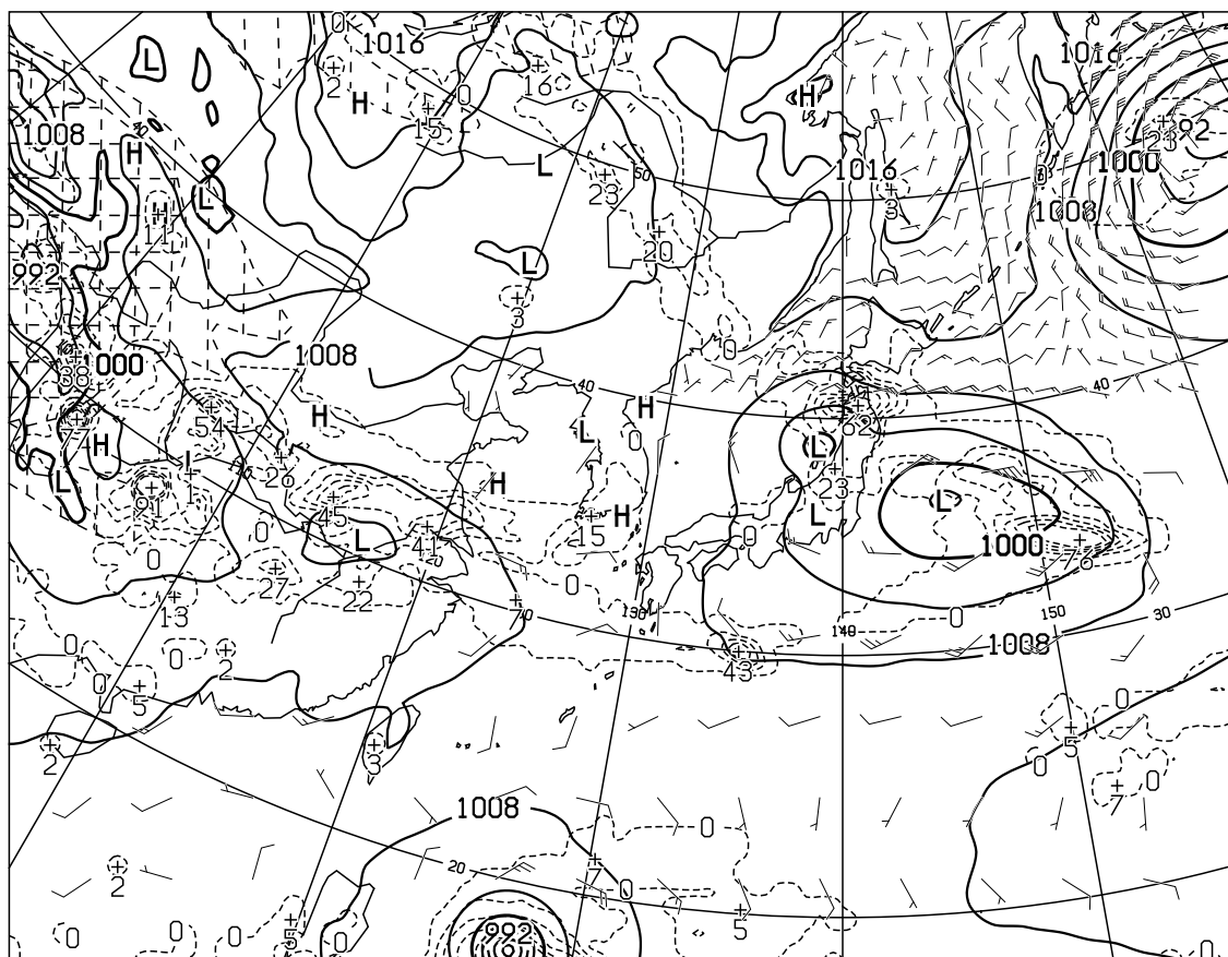
T=12 VALID 220000UTC SURFACE PRESS(hPa),PRECIP(MM) (00-12) WIND ARROW AT SURFACE
