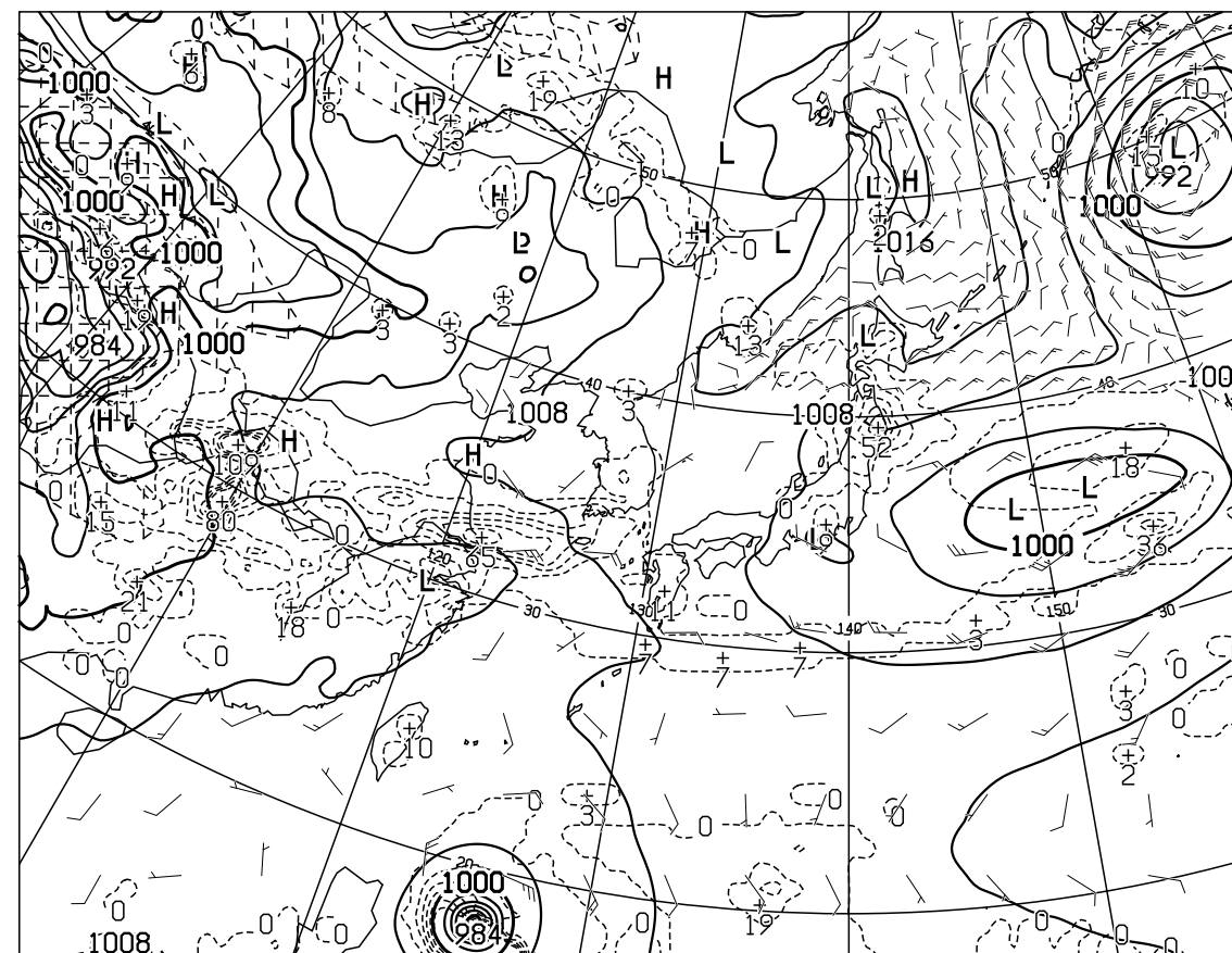
T=24 VALID 221200UTC SURFACE PRESS(hPa),PRECIP(MM) (12-24) WIND ARROW AT SURFACE
