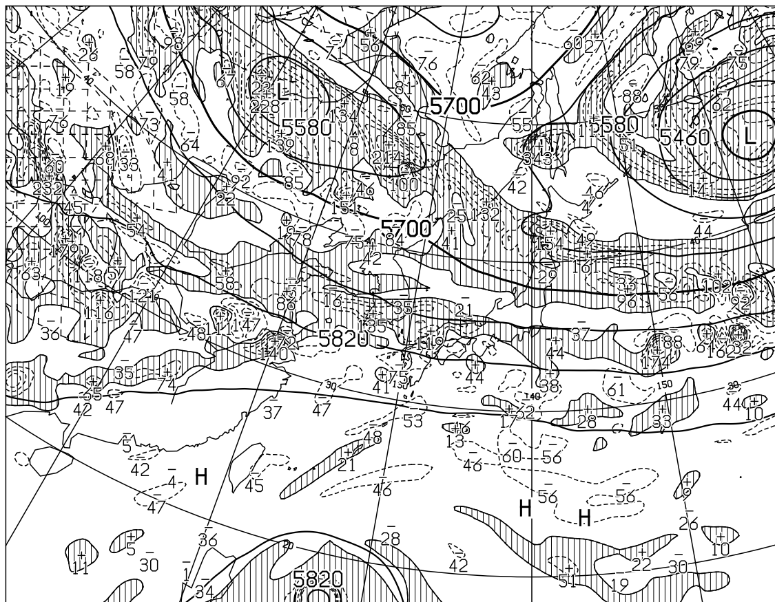
T=12 VALID 220000UTC HEIGHT(M),VORT(10 \times -6/SEC) AT 500hPa
