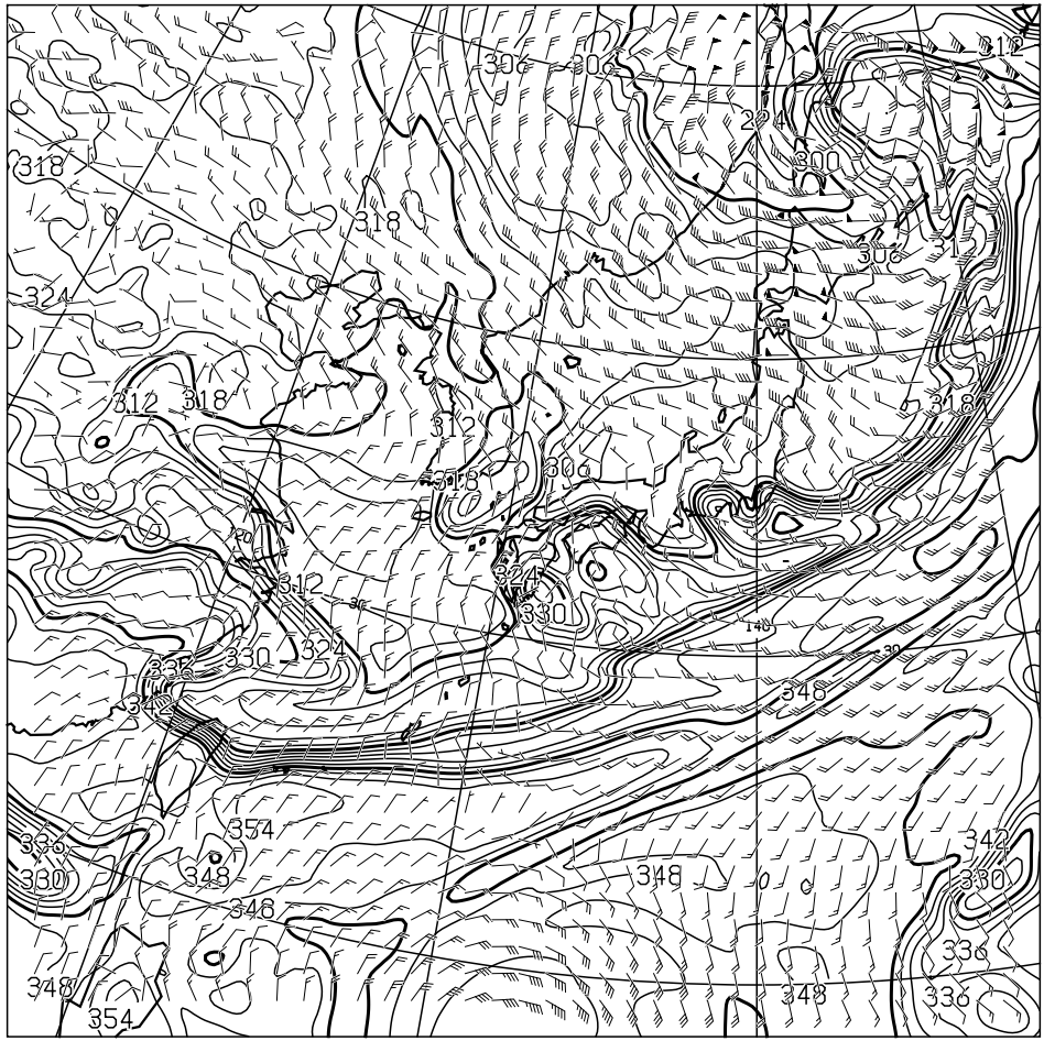
T=24 850hPa: E.P.TEMP(K),WIND(KNOTS) VALID 291200UTC
