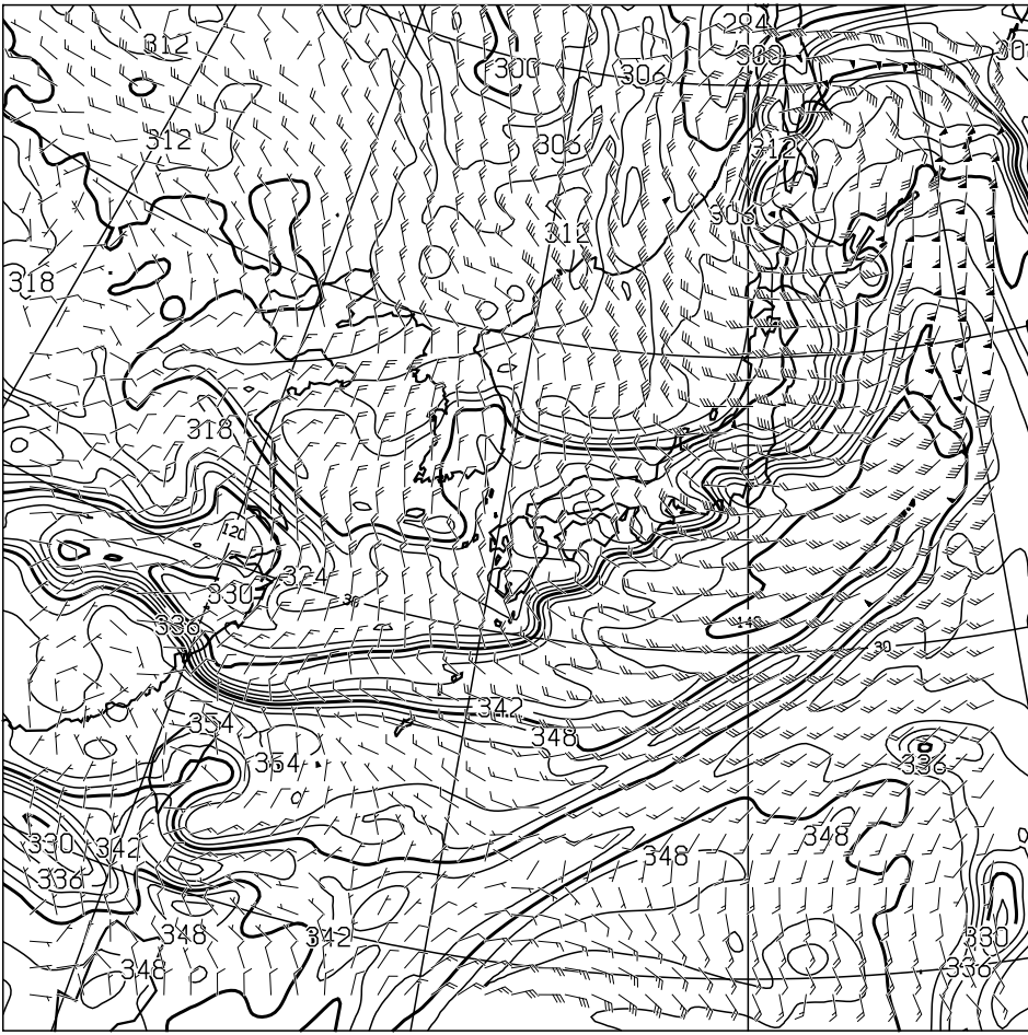
T=12 850hPa: E.P.TEMP(K),WIND(KNOTS) VALID 290000UTC
