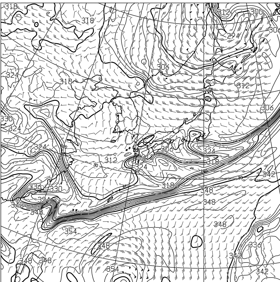
T=36 850hPa: E.P.TEMP(K),WIND(KNOTS) VALID 300000UTC
