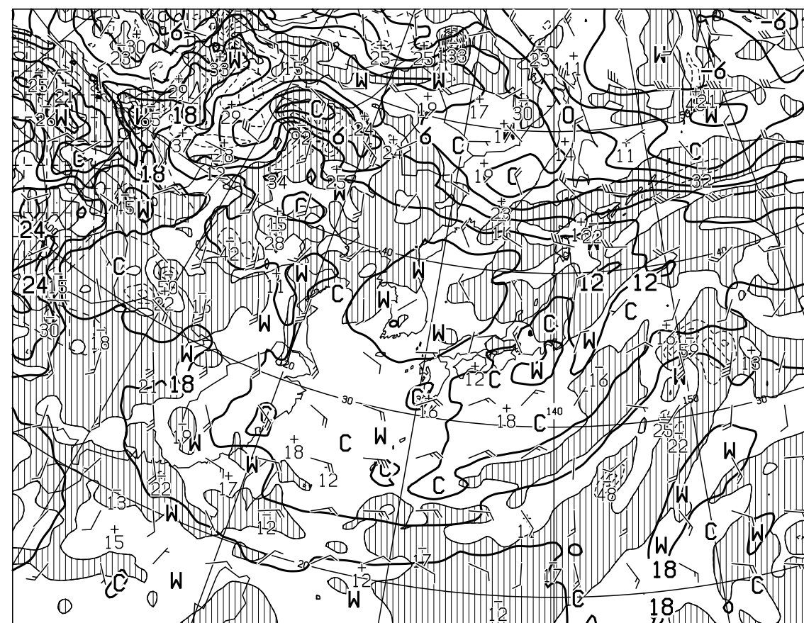
T=24 VALID 161200UTC TEMP (C), WIND ARROW AT 850hPa P-VEL (hPa/H) AT 700hPa
