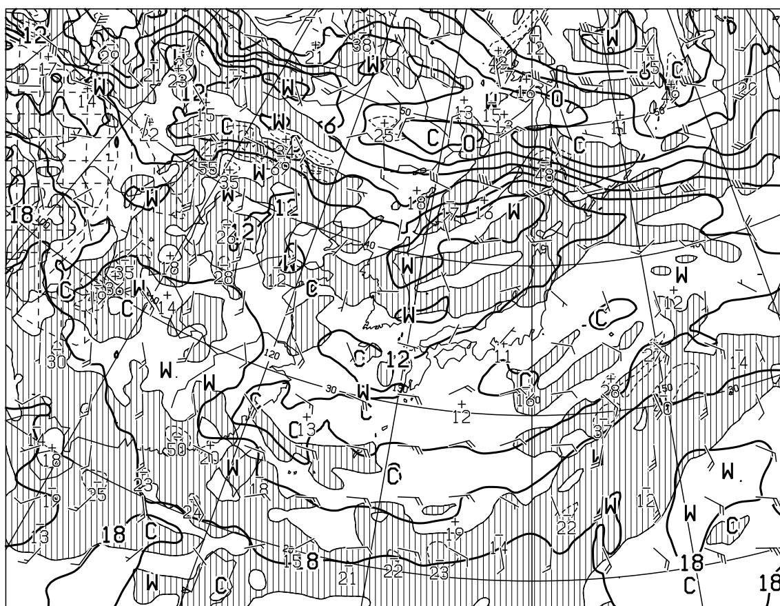
T=12 VALID 160000UTC TEMP (C), WIND ARROW AT 850hPa P-VEL (hPa/H) AT 700hPa
