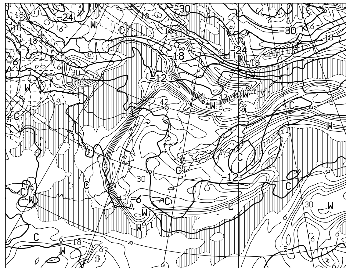
T=24 VALID 161200UTC TEMP (C) AT 500hPa T-TD (C) AT 700hPa
