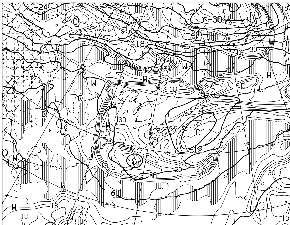
T=12 VALID 160000UTC TEMP (C) AT 500hPa T-TD (C) AT 700hPa
