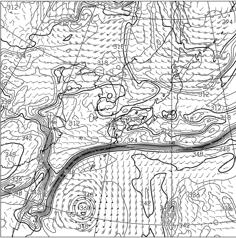
T=12 850hPa: E.P.TEMP(K),WIND(KNOTS) VALID 310000UTC
