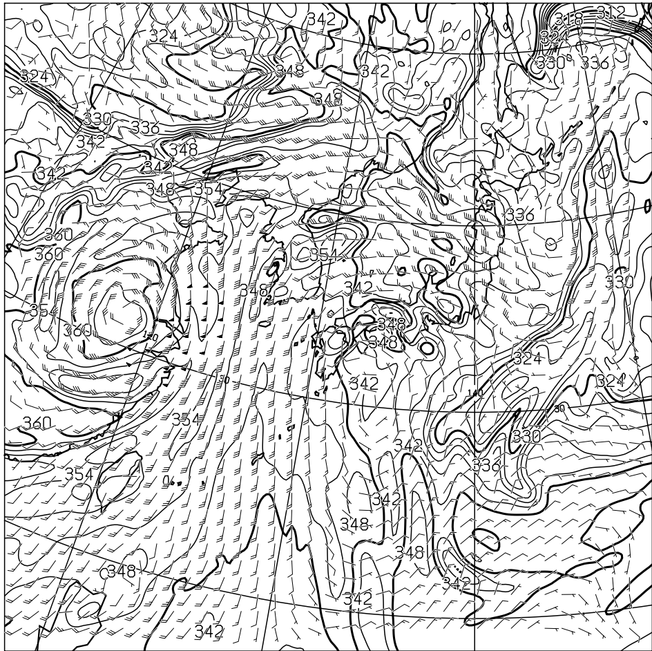
T=24 850hPa: E.P.TEMP(K),WIND(KNOTS) VALID 121200UTC
