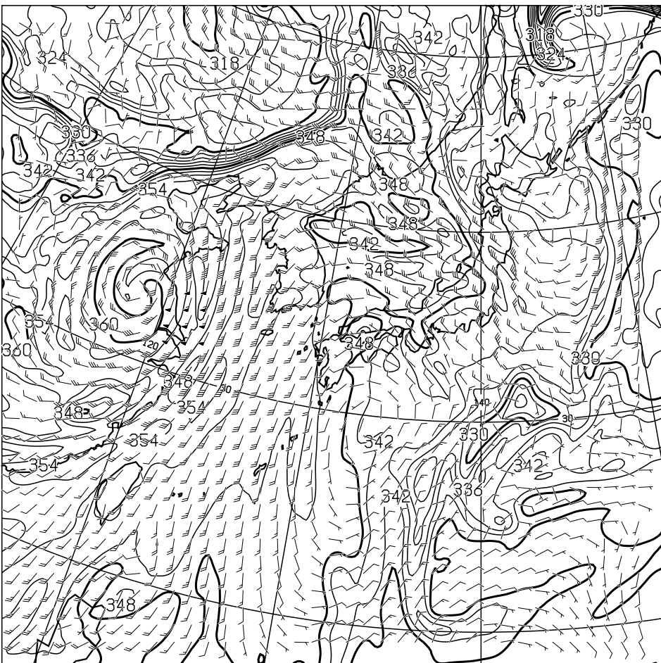
T=36 850hPa: E.P.TEMP(K),WIND(KNOTS) VALID 130000UTC
