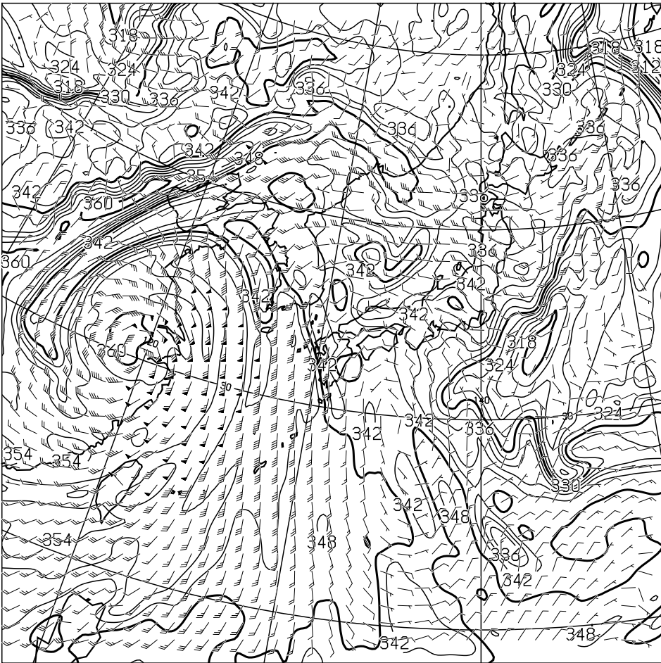
T=12 850hPa: E.P.TEMP(K),WIND(KNOTS) VALID 120000UTC
