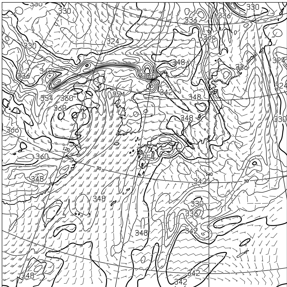
T=48 850hPa: E.P.TEMP(K),WIND(KNOTS) VALID 131200UTC
