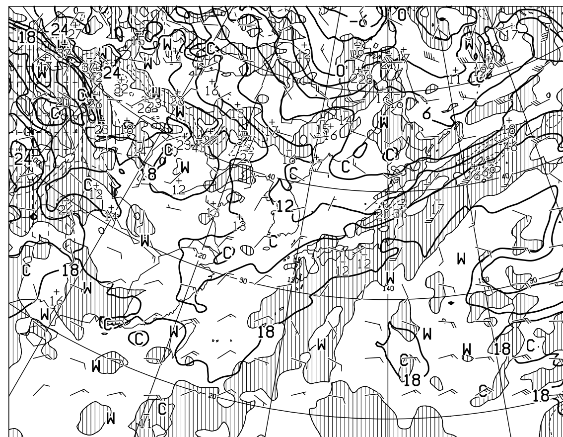
T=24 VALID 151200UTC TEMP (C), WIND ARROW AT 850hPa P-VEL (hPa/h) AT 700hPa
