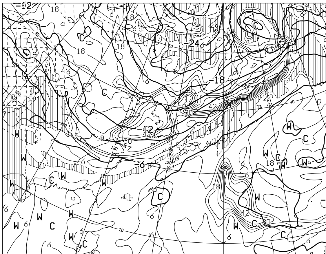
T=12 VALID 150000UTC TEMP (C) AT 500hPa T-TD (C) AT 700hPa
