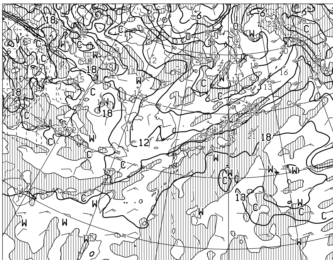
T=12 VALID 150000UTC TEMP (C), WIND ARROW AT 850hPa P-VEL (hPa/h) AT 700hPa
