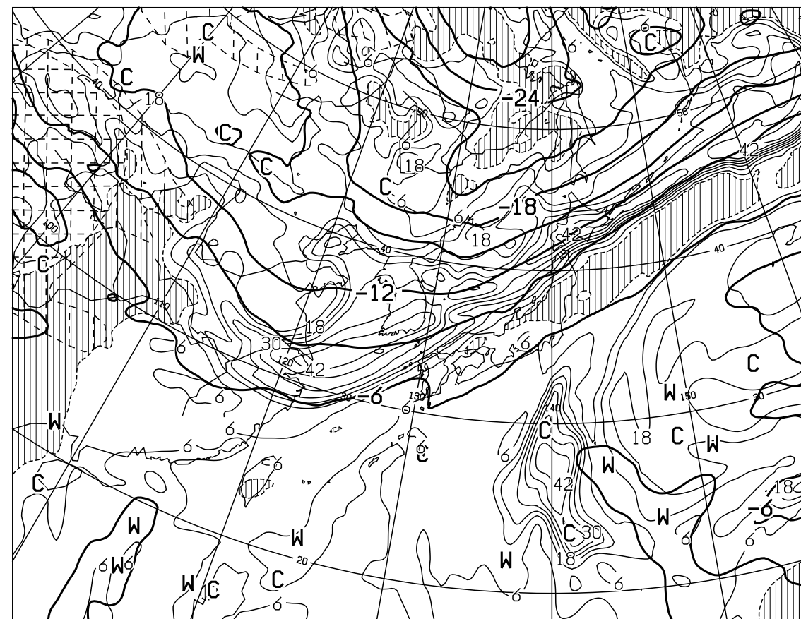
T=24 VALID 151200UTC TEMP (C) AT 500hPa T-TD (C) AT 700hPa
