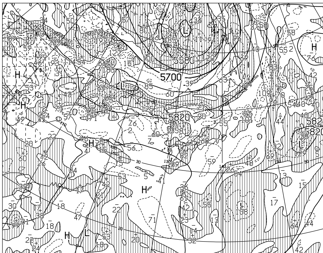
T=12 VALID 170000UTC HEIGHT(M),VORT(10** \times -6/SEC) AT 500hPa
