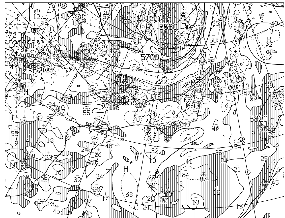
T=24 VALID 171200UTC HEIGHT(M),VORT(10** \times -6/SEC) AT 500hPa
