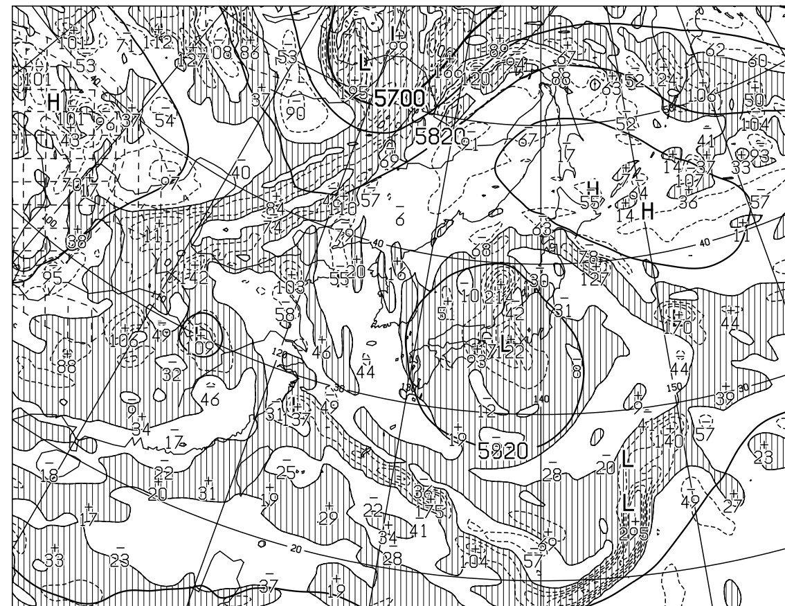
T=24 VALID 121200UTC HEIGHT(M),VORT(10 \times -6/SEC) AT 500hPa
