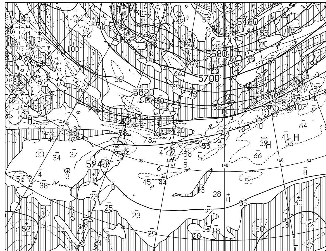
T=24 VALID 111200UTC HEIGHT(M),VORT(10 \times -6/SEC) AT 500hPa
