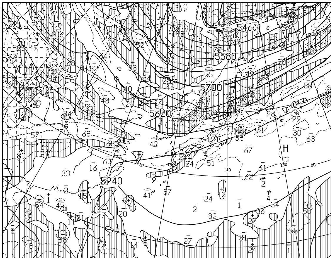
T=12 VALID 110000UTC HEIGHT(M),VORT(10 \times -6/SEC) AT 500hPa
