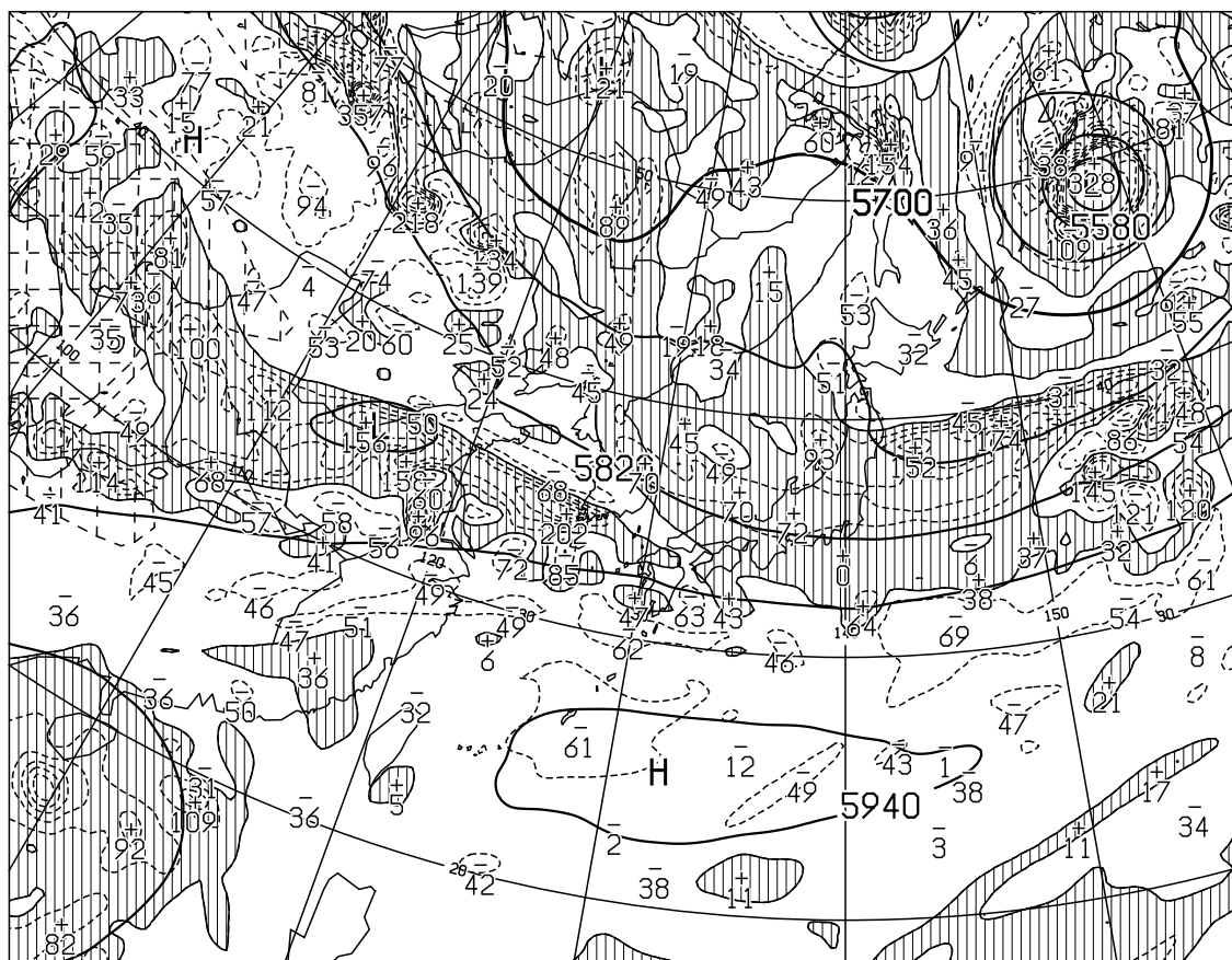
T=12 VALID 030000UTC HEIGHT(M),VORT(10××-6/SEC) AT 500hPa
