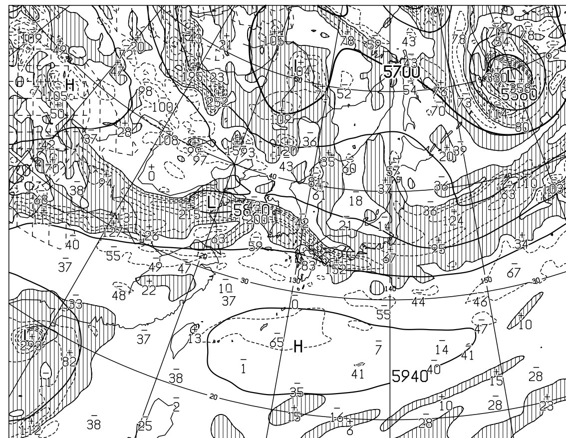
T=24 VALID 031200UTC HEIGHT(M),VORT(10××-6/SEC) AT 500hPa
