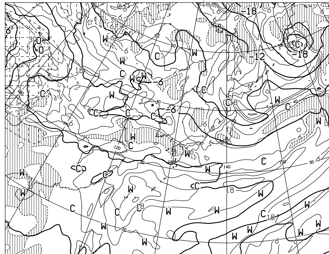
T=24 VALID 031200UTC TEMP (C) AT 500hPa T-TD (C) AT 700hPa
