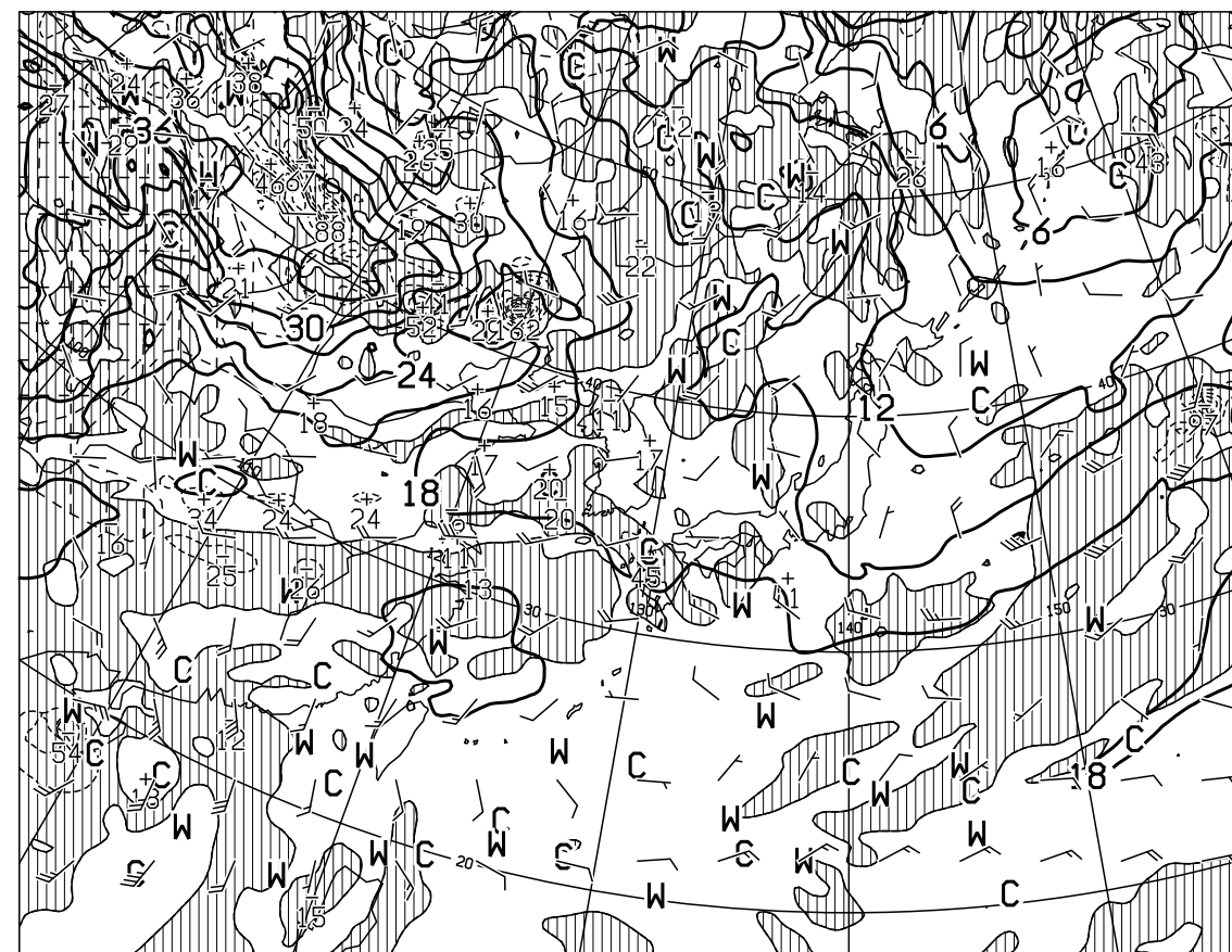
T=24 VALID 031200UTC TEMP (C), WIND ARROW AT 850hPa P-VEL (hPa/H) AT 700hPa
