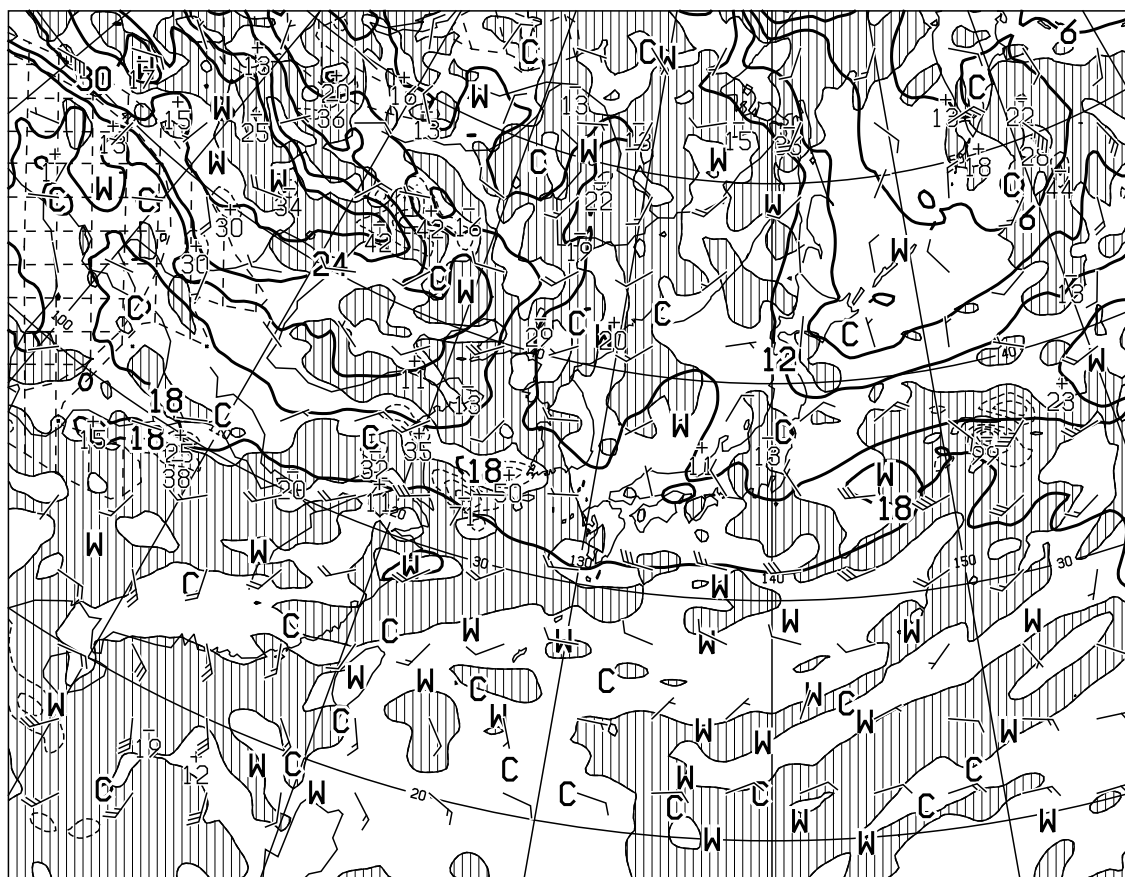
T=12 VALID 030000UTC TEMP (C), WIND ARROW AT 850hPa P-VEL (hPa/H) AT 700hPa
