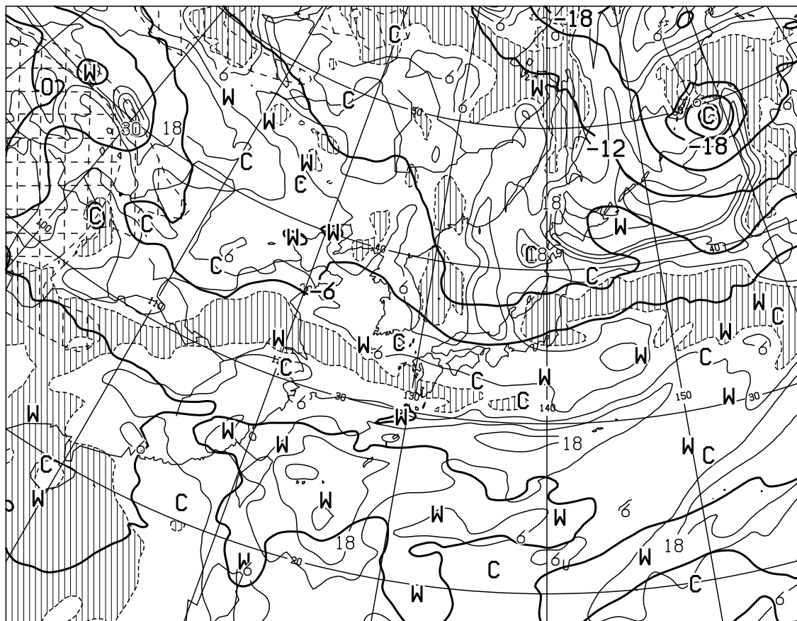
T=12 VALID 030000UTC TEMP (C) AT 500hPa T-TD (C) AT 700hPa
