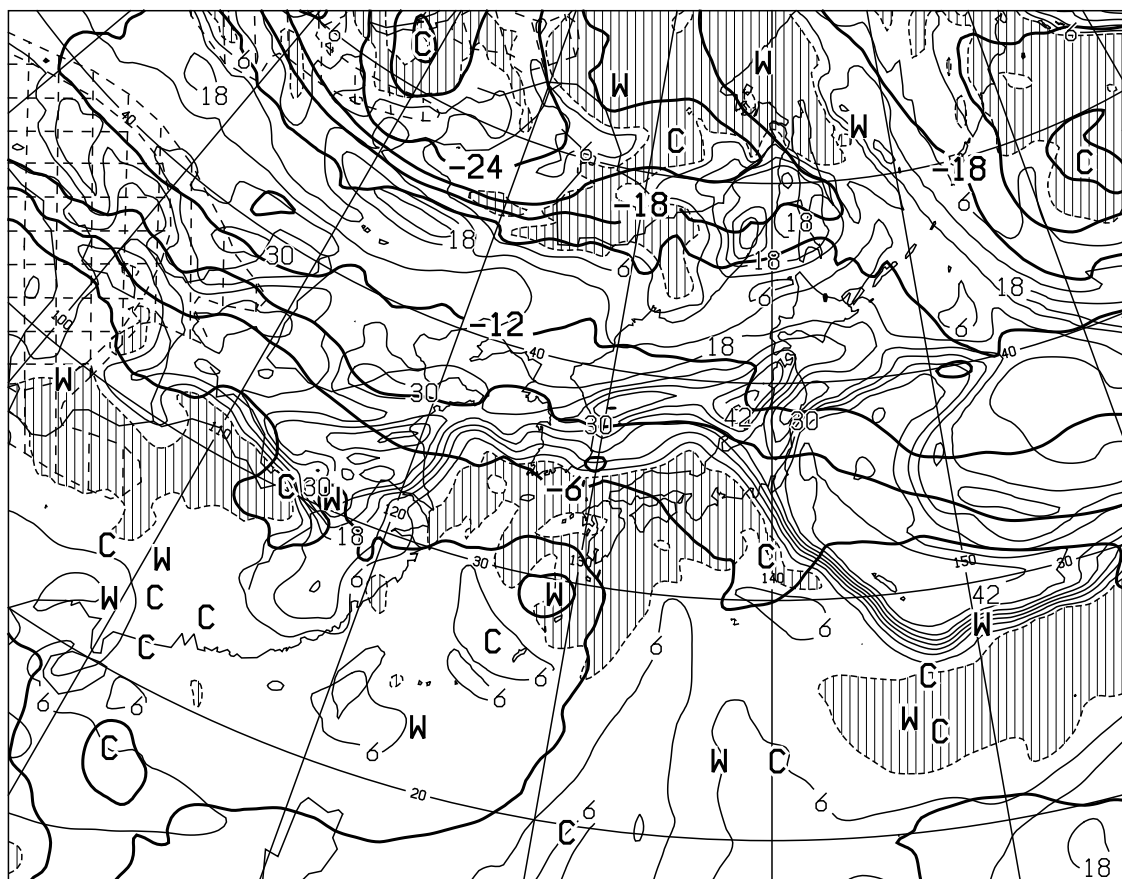
T=12 VALID 020000UTC TEMP (C) AT 500hPa T-TD (C) AT 700hPa
