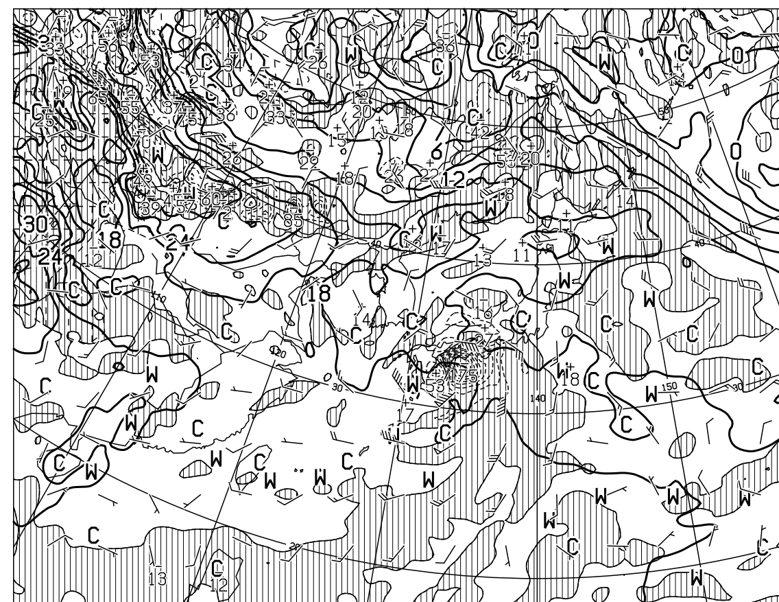
T=24 VALID 021200UTC TEMP (C), WIND ARROW AT 850hPa P-VEL (hPa/H) AT 700hPa
