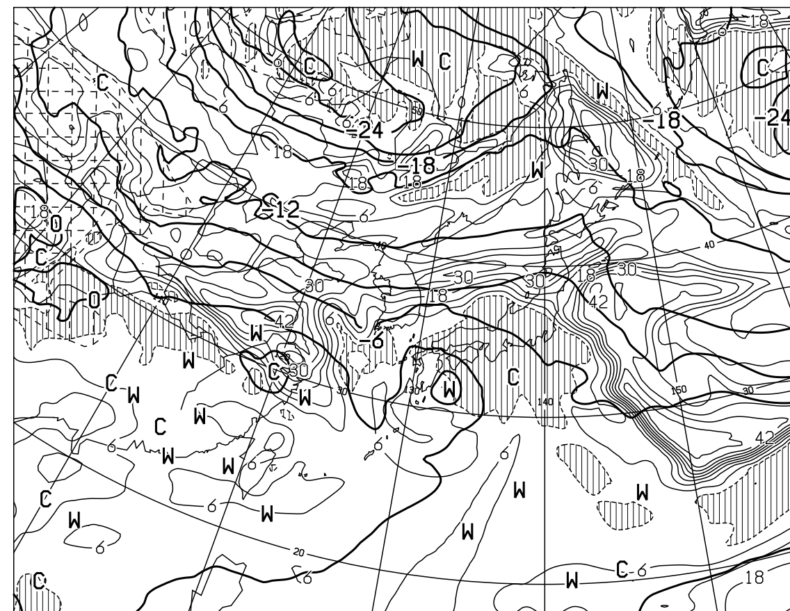
T=24 VALID 021200UTC TEMP (C) AT 500hPa T-TD (C) AT 700hPa
