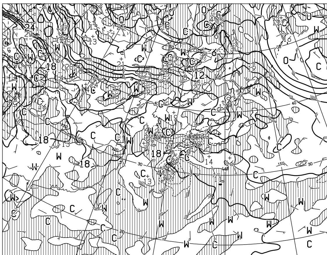
T=12 VALID 020000UTC TEMP (C), WIND ARROW AT 850hPa P-VEL (hPa/H) AT 700hPa
