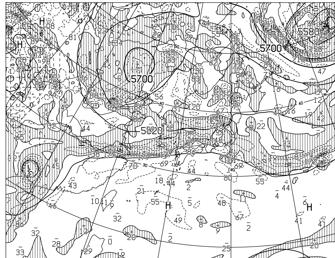
T=24 VALID 051200UTC HEIGHT(M),VORT(10××-6/SEC) AT 500hPa
