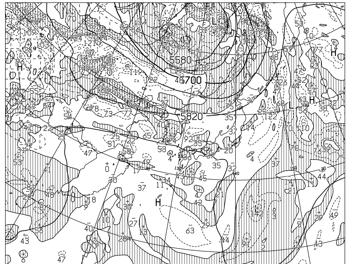
T=24 VALID 161200UTC HEIGHT(M),VORT(10**6/SEC) AT 500hPa
