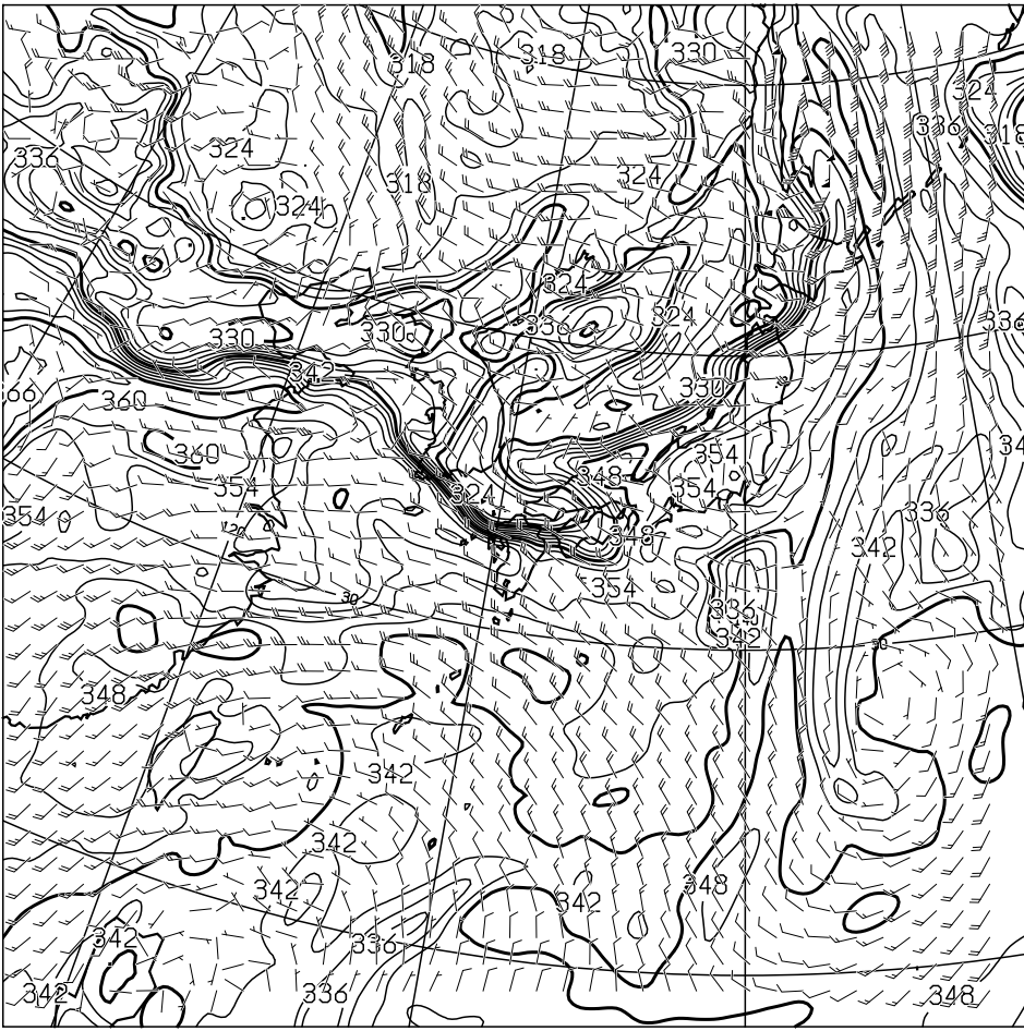
T=12 850hPa: E.P.TEMP(K),WIND(KNOTS) VALID 160000UTC
