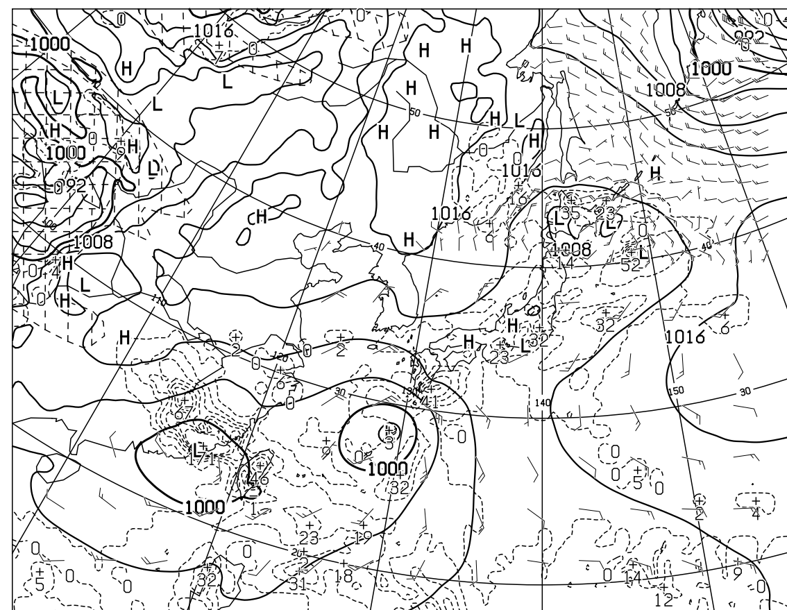
T=24 VALID 031200UTC SURFACE PRESS(hPa),PRECIP(MM) (12-24) WIND ARROW AT SURFACE
