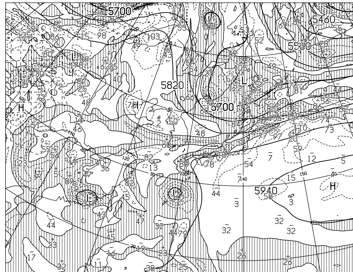
T=24 VALID 031200UTC HEIGHT(M),VORT(10** \times -6/SEC) AT 500hPa
