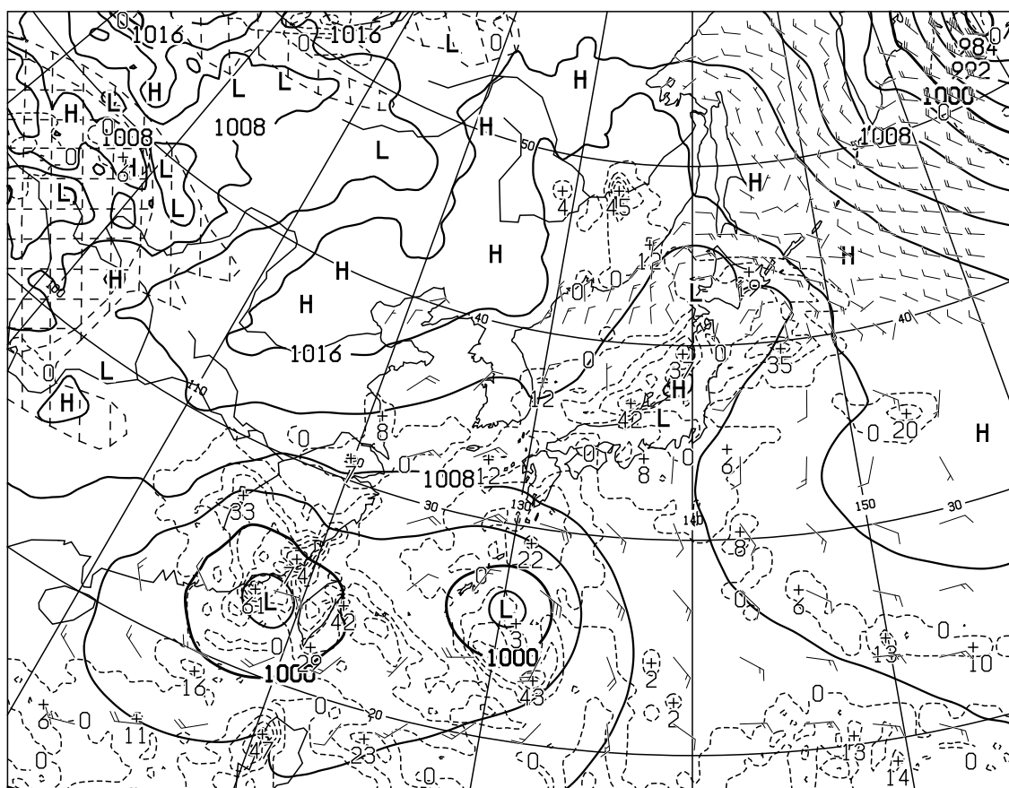
T=12 VALID 030000UTC SURFACE PRESS(hPa),PRECIP(MM) (00-12) WIND ARROW AT SURFACE
