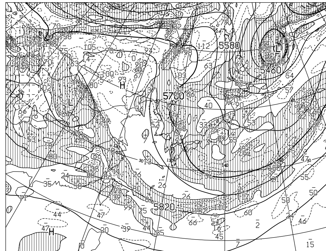
T=24 VALID 131200UTC HEIGHT(M),VORT(10 \times -6/SEC) AT 500hPa
