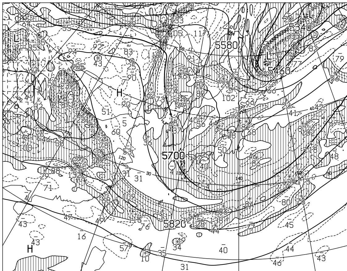
T=12 VALID 130000UTC HEIGHT(M),VORT(10 \times -6/SEC) AT 500hPa
