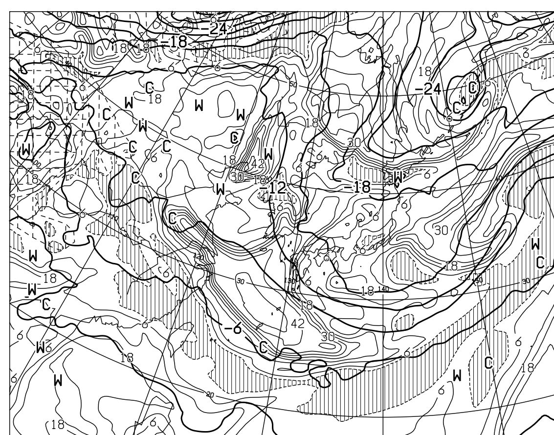
T=24 VALID 131200UTC TEMP (C) AT 500hPa T-TD (C) AT 700hPa
