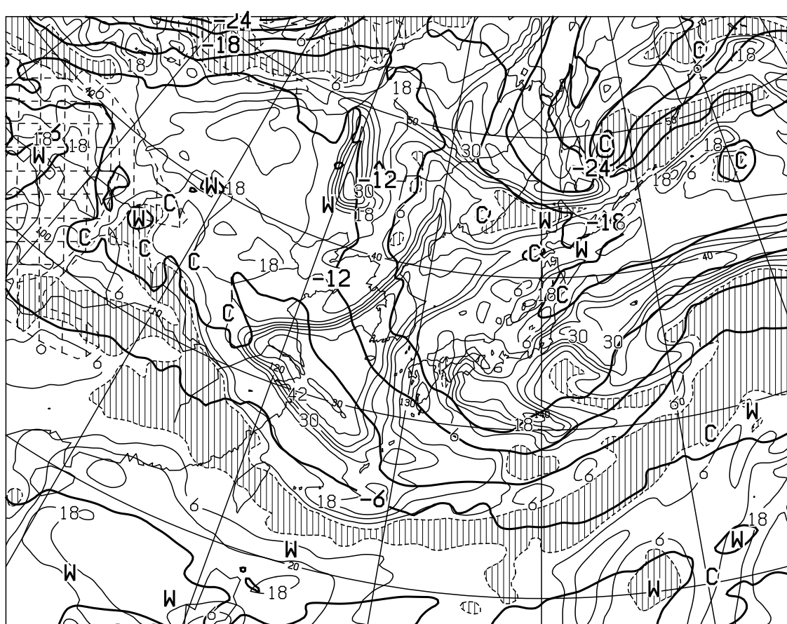
T=12 VALID 130000UTC TEMP (C) AT 500hPa T-TD (C) AT 700hPa
