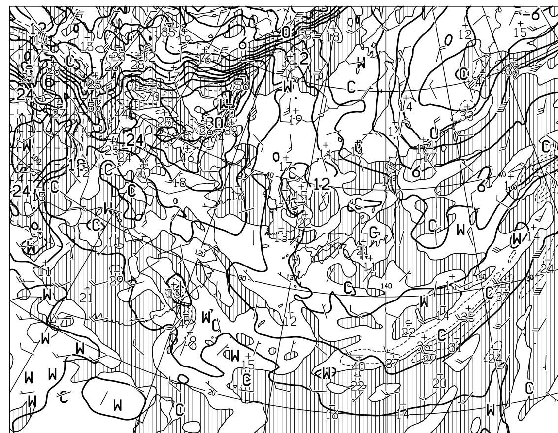
T=24 VALID 131200UTC TEMP (C), WIND ARROW AT 850hPa P-VEL (hPa/H) AT 700hPa
