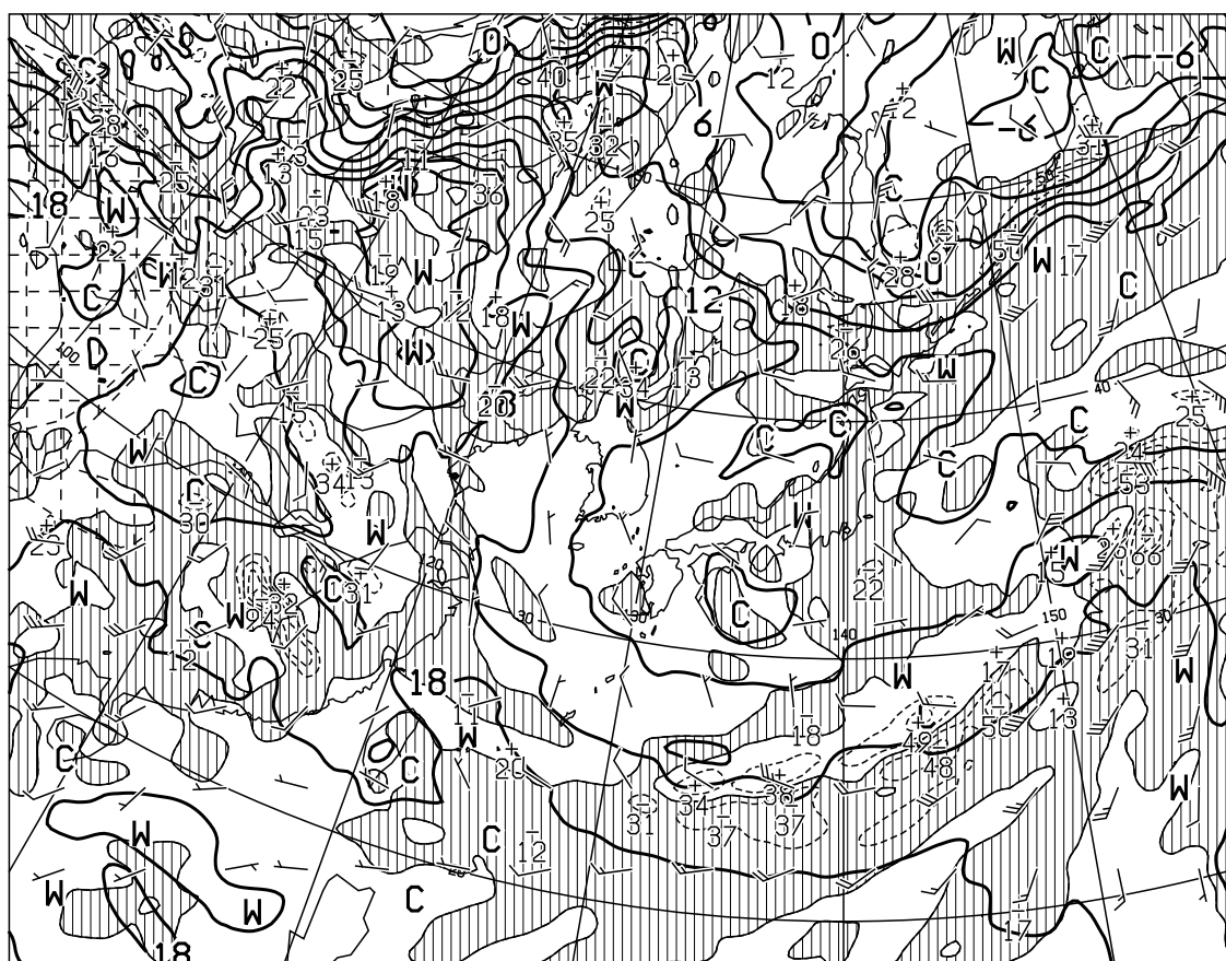
T=12 VALID 130000UTC TEMP (C), WIND ARROW AT 850hPa P-VEL (hPa/H) AT 700hPa
