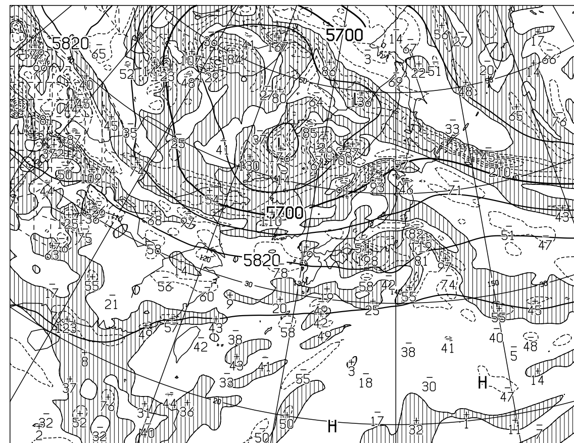
T=24 VALID 071200UTC HEIGHT(M),VORT(10 -6 /SEC) AT 500hPa
