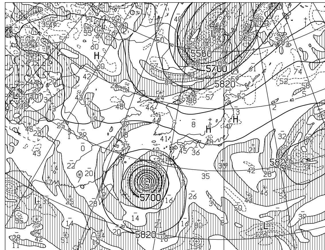
T=24 VALID 071200UTC HEIGHT(M),VORT(10 \times -6/SEC) AT 500hPa
