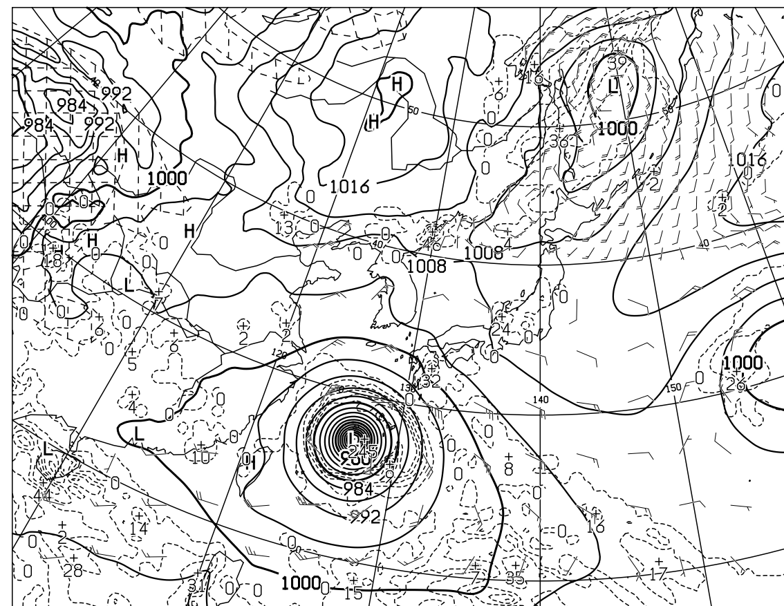
T=24 VALID 071200UTC SURFACE PRESS(hPa),PRECIP(MM) (12-24) WIND ARROW AT SURFACE
