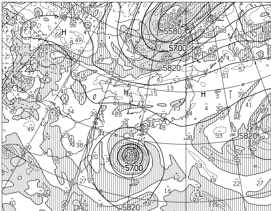
T=12 VALID 070000UTC HEIGHT(M),VORT(10 \times -6/SEC) AT 500hPa
