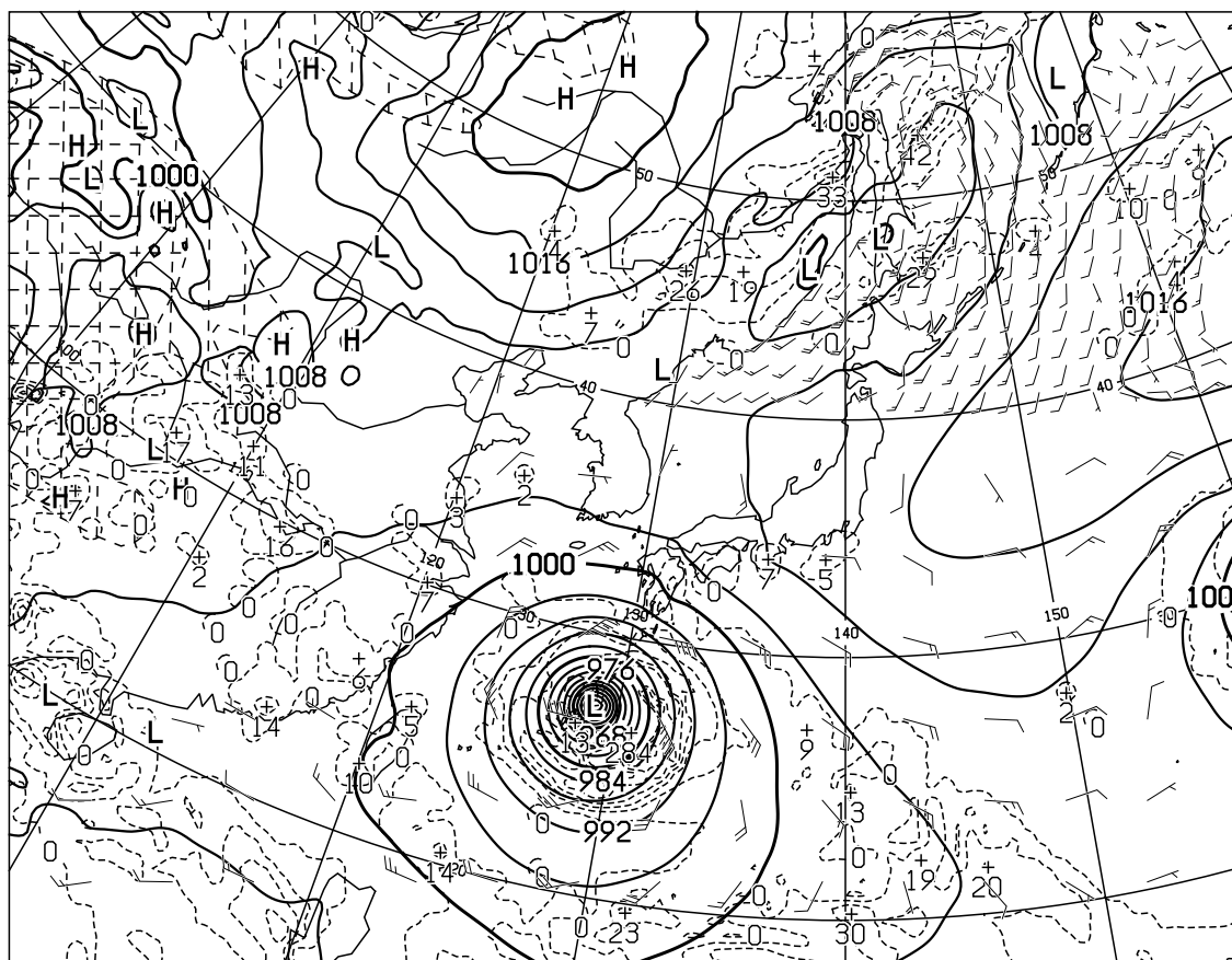
T=12 VALID 070000UTC SURFACE PRESS(hPa),PRECIP(MM) (00-12) WIND ARROW AT SURFACE
