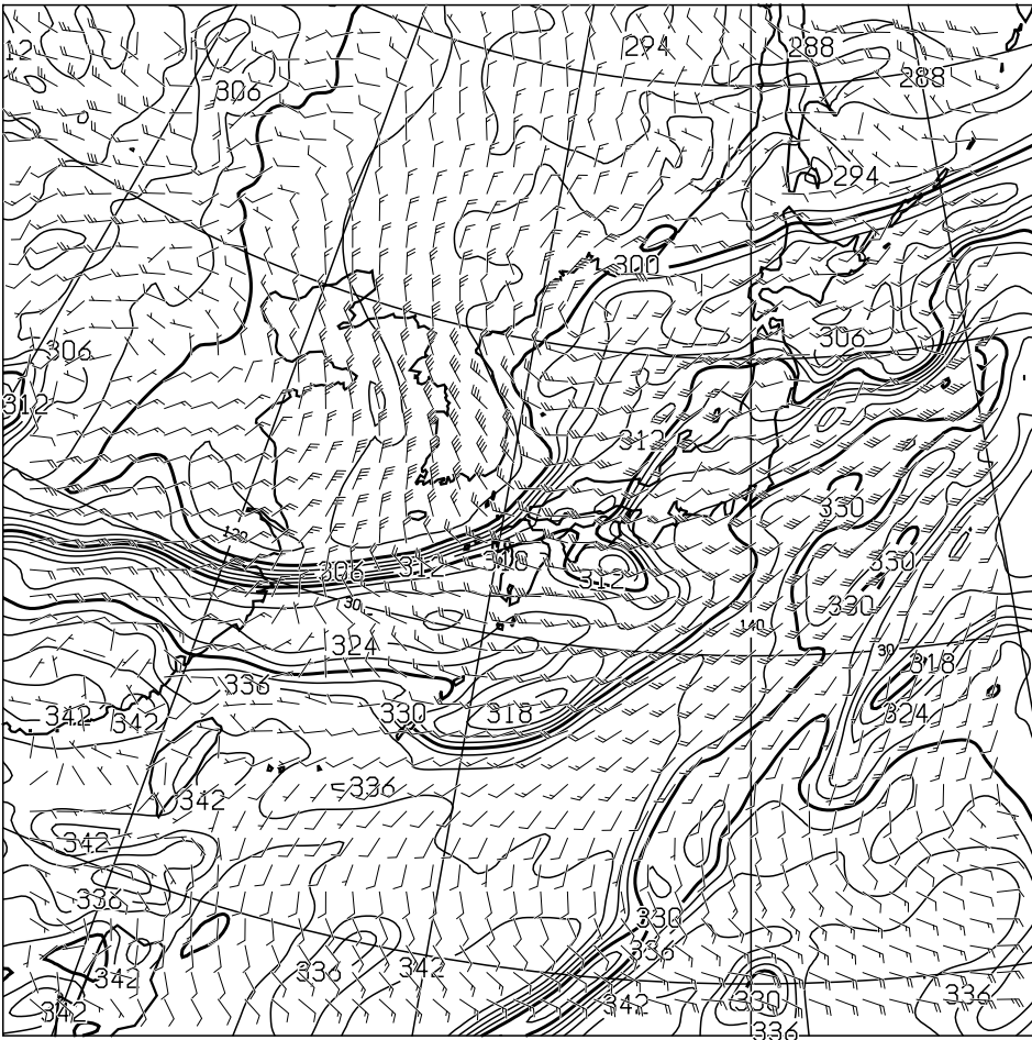
T=12 850hPa: E.P.TEMP(K),WIND(KNOTS) VALID 080000UTC
