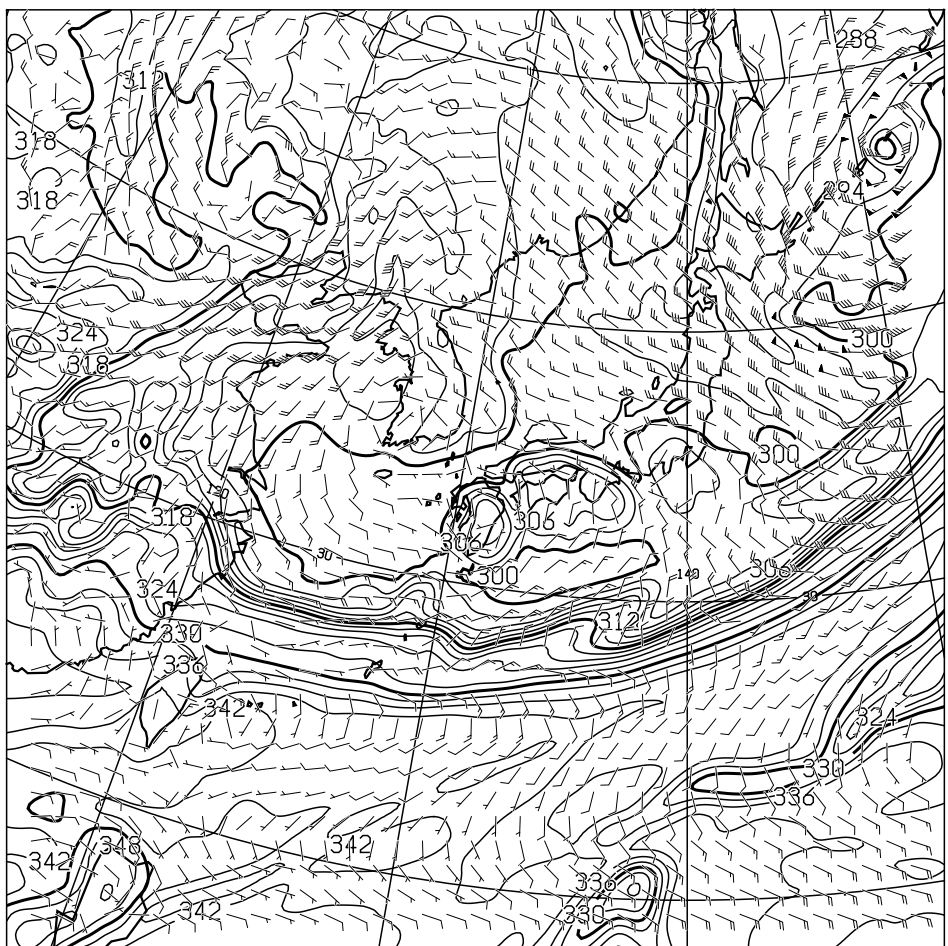
T=48 850hPa: E.P.TEMP(K),WIND(KNOTS) VALID 091200UTC
