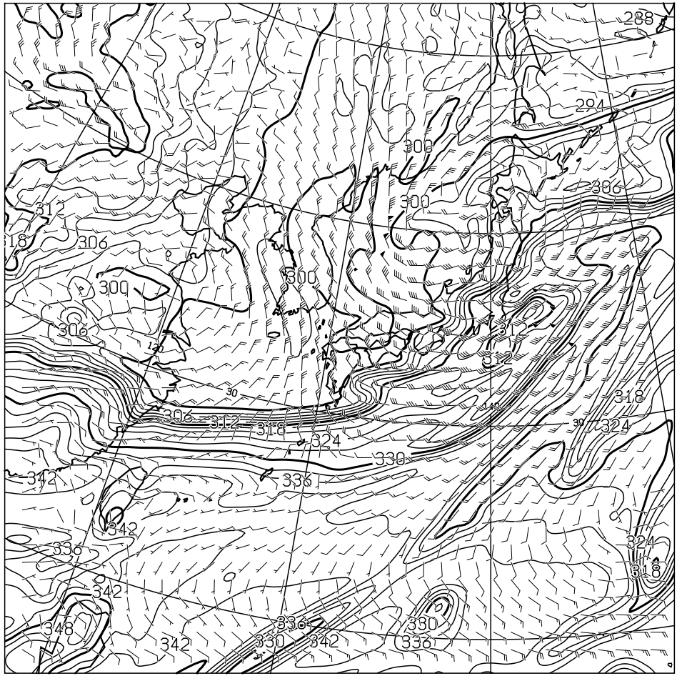
T=24 850hPa: E.P.TEMP(K),WIND(KNOTS) VALID 081200UTC
