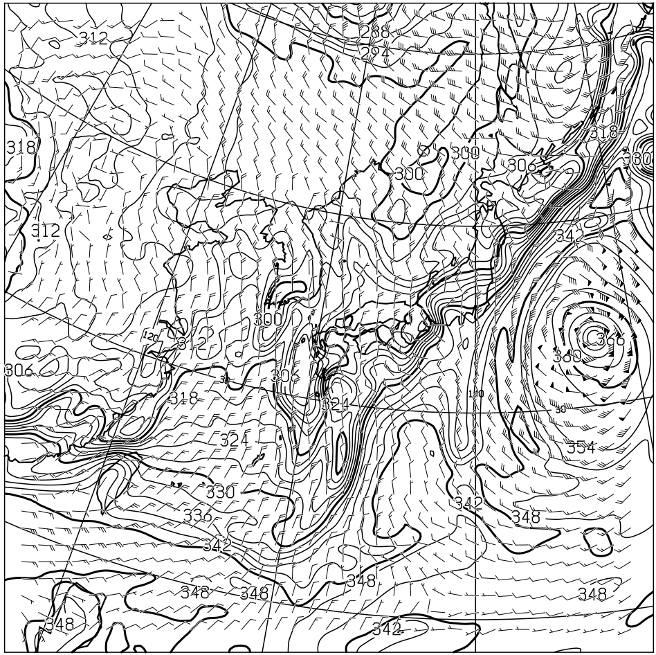
T=24 850hPa: E.P.TEMP(K),WIND(KNOTS) VALID 061200UTC
