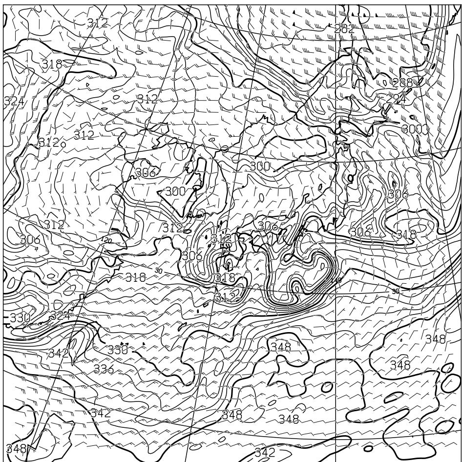
T=48 850hPa: E.P.TEMP(K),WIND(KNOTS) VALID 071200UTC
