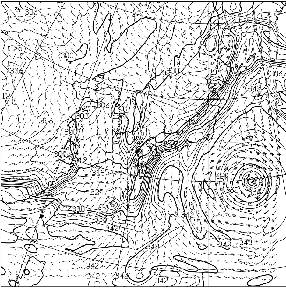
T=12 850hPa: E.P.TEMP(K),WIND(KNOTS) VALID 060000UTC
