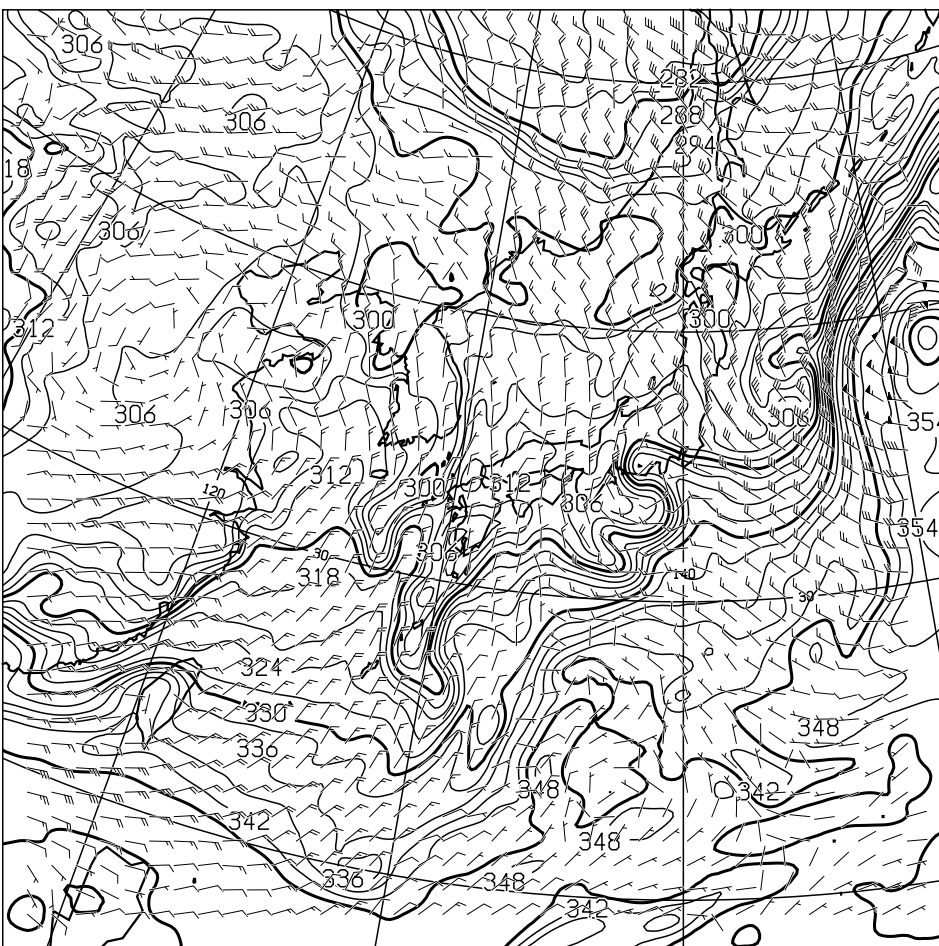
T=36 850hPa: E.P.TEMP(K),WIND(KNOTS) VALID 070000UTC
