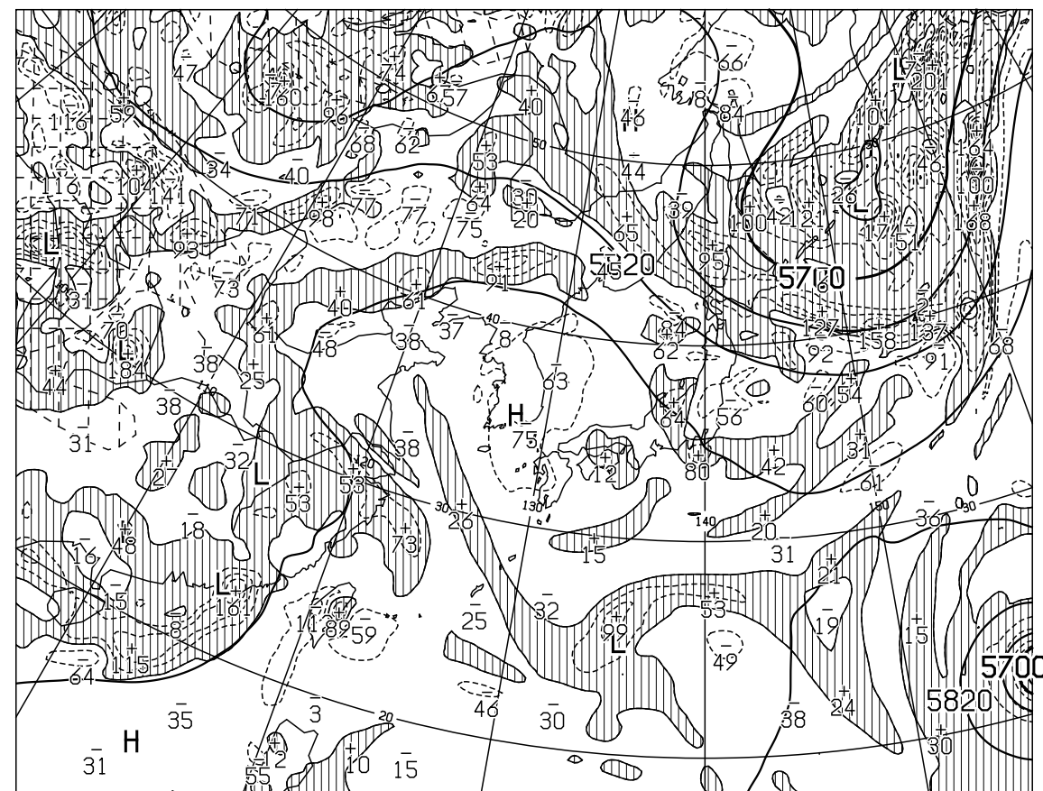
T=24 VALID 011200UTC HEIGHT(M),VORT(10 \times -6/SEC) AT 500hPa
