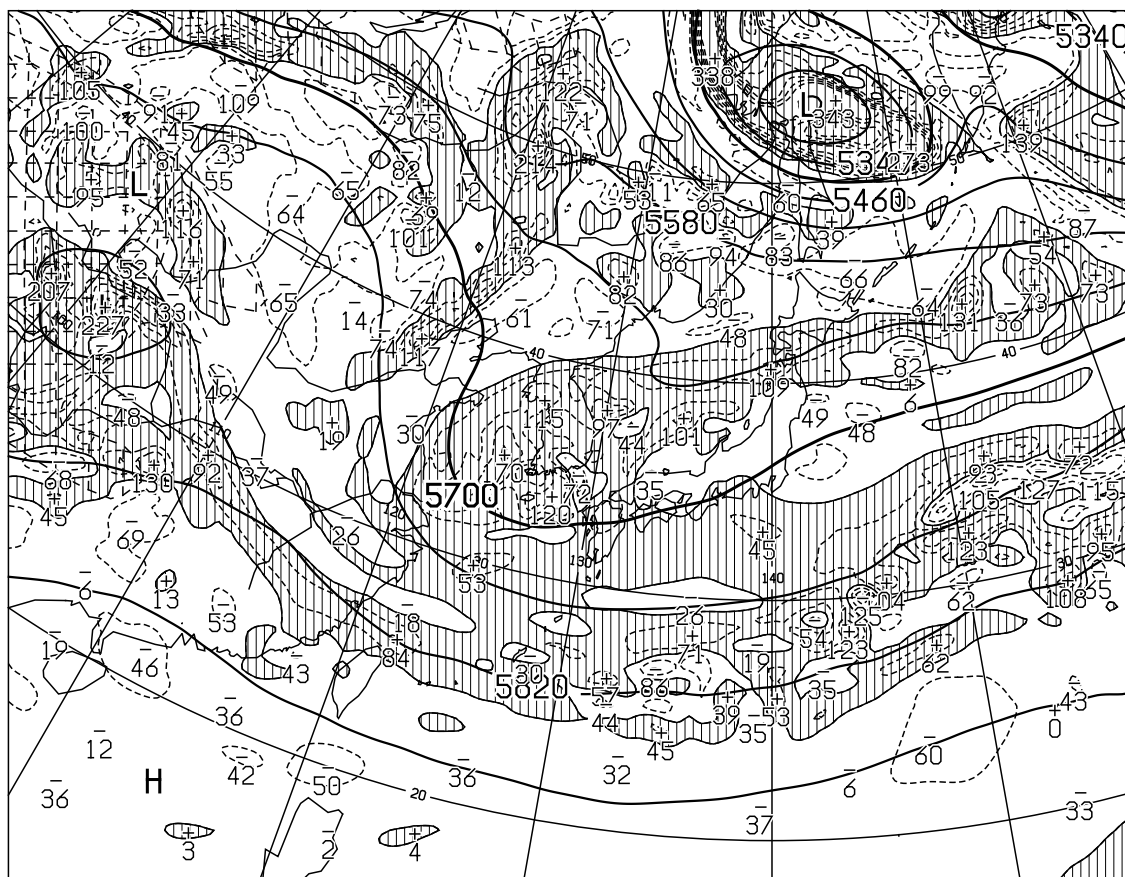
T=12 VALID 120000UTC HEIGHT(M),VORT(10××-6/SEC) AT 500hPa
