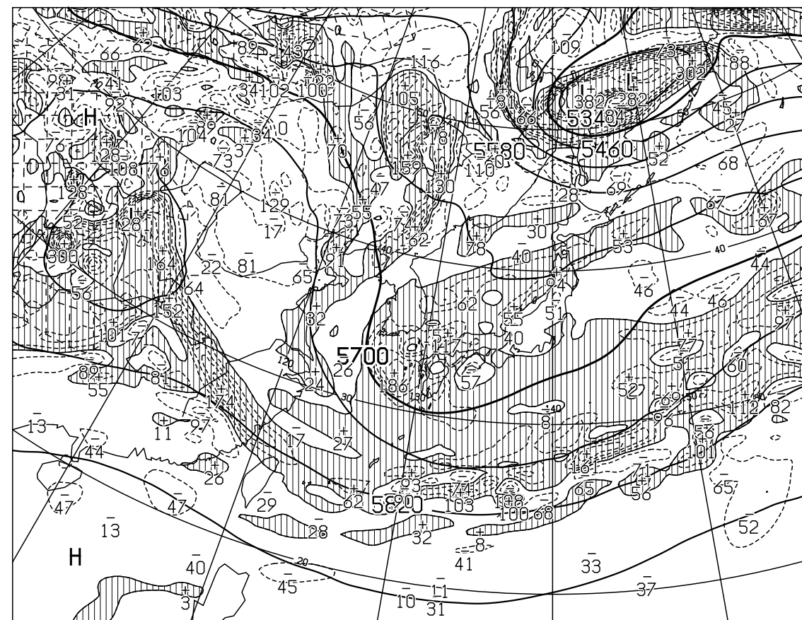
T=24 VALID 121200UTC HEIGHT(M),VORT(10××-6/SEC) AT 500hPa
