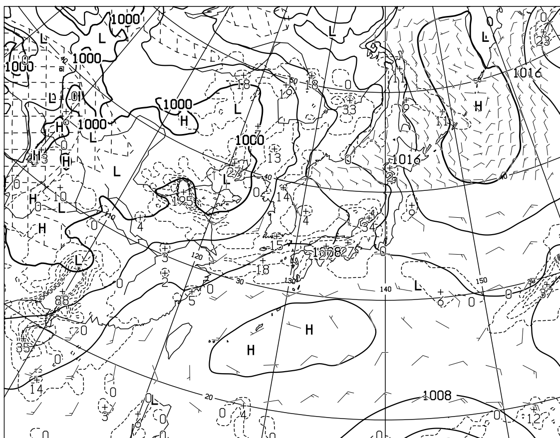
T=12 VALID 060000UTC SURFACE PRESS(hPa),PRECIP(MM) (00-12) WIND ARROW AT SURFACE
