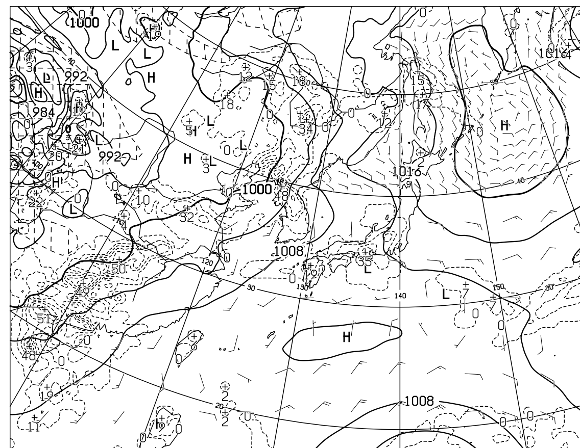
T=24 VALID 061200UTC SURFACE PRESS(hPa),PRECIP(MM) (12-24) WIND ARROW AT SURFACE
