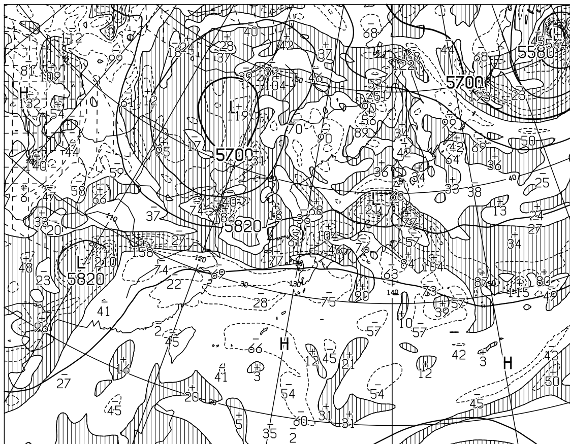
T=12 VALID 060000UTC HEIGHT(M),VORT(10 \times -6/SEC) AT 500hPa
