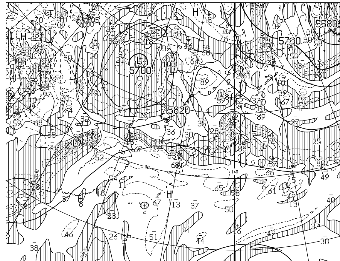
T=24 VALID 061200UTC HEIGHT(M),VORT(10 \times -6/SEC) AT 500hPa
