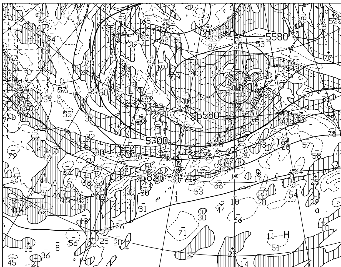
T=12 VALID 090000UTC HEIGHT(M),VORT(10×-6/SEC) AT 500hPa
