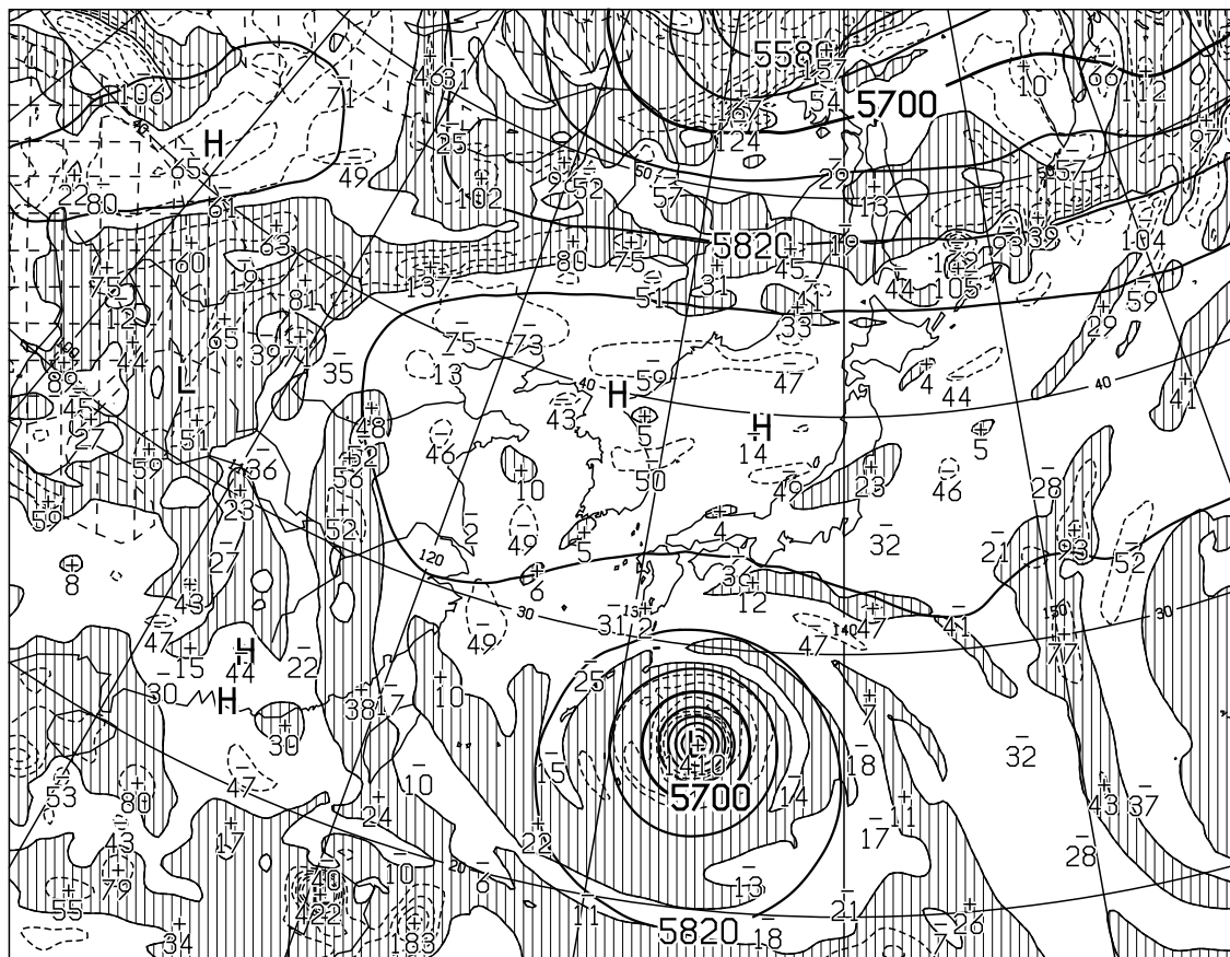
T=12 VALID 060000UTC HEIGHT(M),VORT(10**x-6/SEC) AT 500hPa
