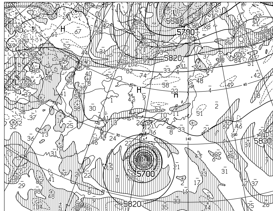
T=24 VALID 061200UTC HEIGHT(M),VORT(10**x-6/SEC) AT 500hPa
