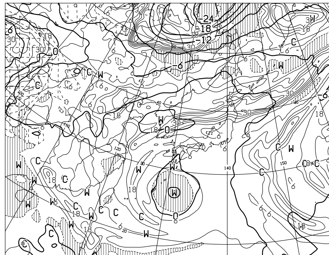
T=24 VALID 061200UTC TEMP (C) AT 500hPa T-TD (C) AT 700hPa
