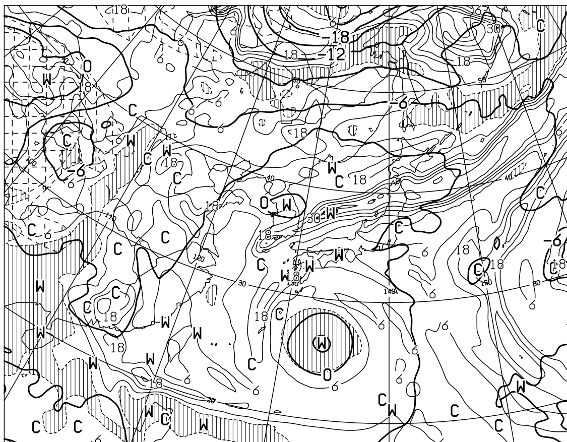
T=12 VALID 060000UTC TEMP (C) AT 500hPa T-TD (C) AT 700hPa
