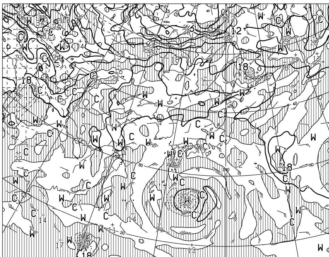
T=12 VALID 060000UTC TEMP (C), WIND ARROW AT 850hPa P-VEL (hPa/H) AT 700hPa
