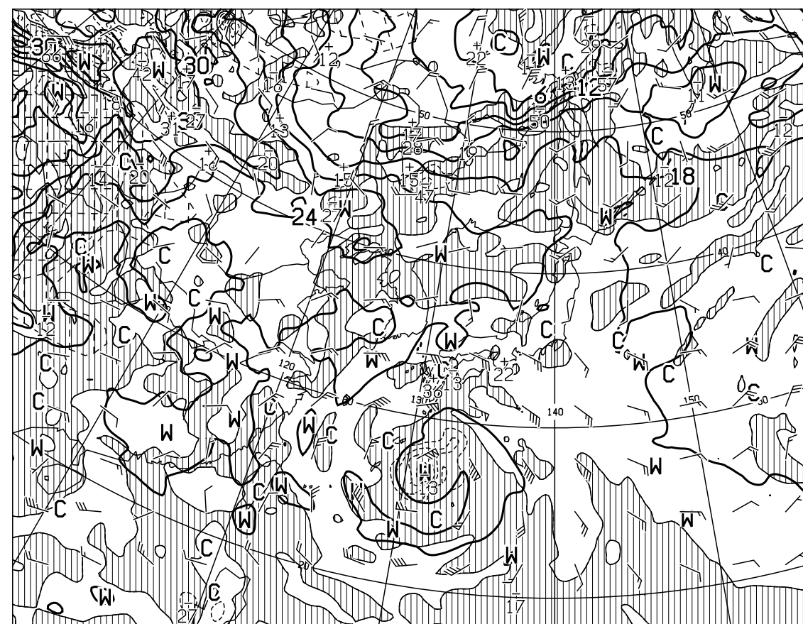
T=24 VALID 061200UTC TEMP (C), WIND ARROW AT 850hPa P-VEL (hPa/H) AT 700hPa
