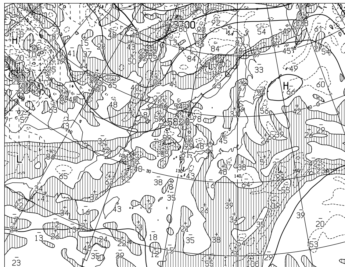
T=24 VALID 151200UTC HEIGHT(M),VORT(10**x-6/SEC) AT 500hPa
