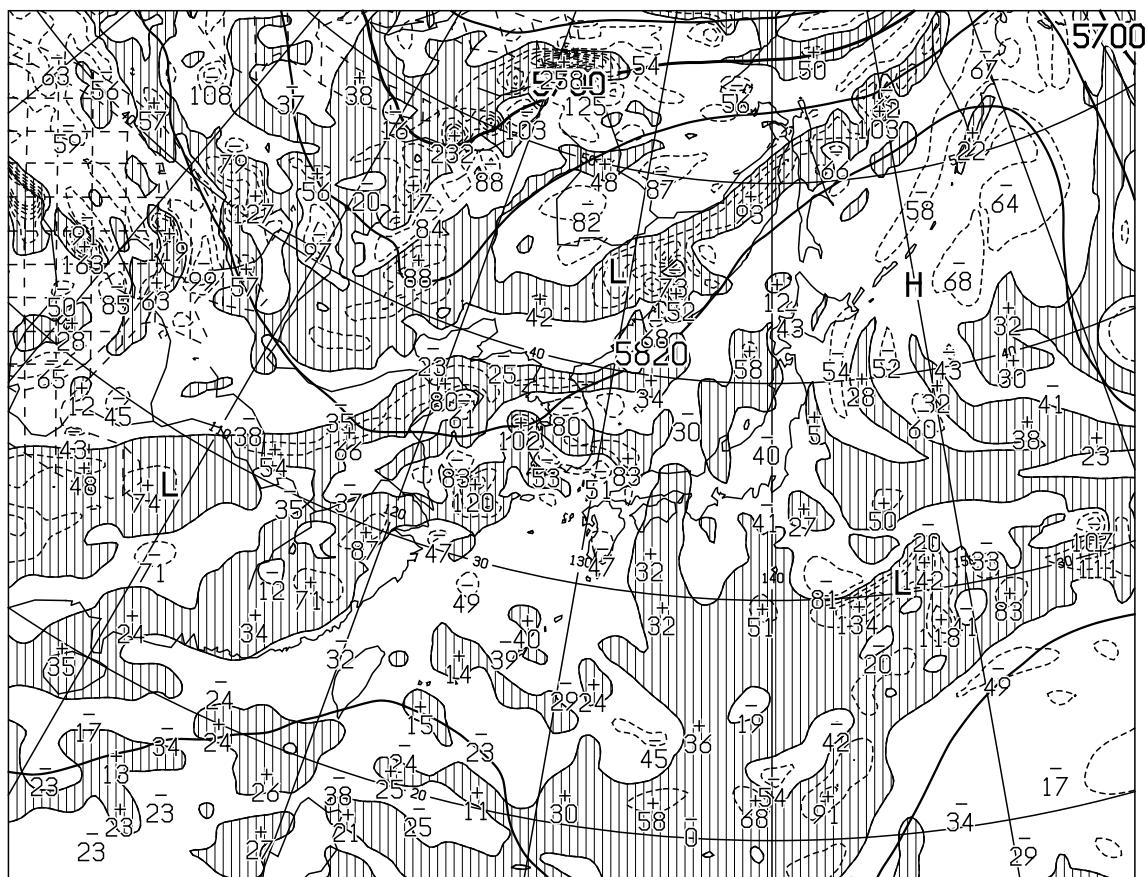
T=12 VALID 150000UTC HEIGHT(M),VORT(10**x-6/SEC) AT 500hPa
