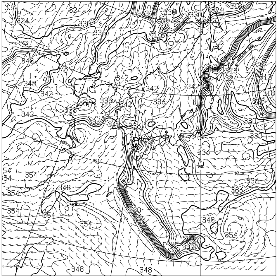
T=24 850hPa: E.P.TEMP(K),WIND(KNOTS) VALID 151200UTC
