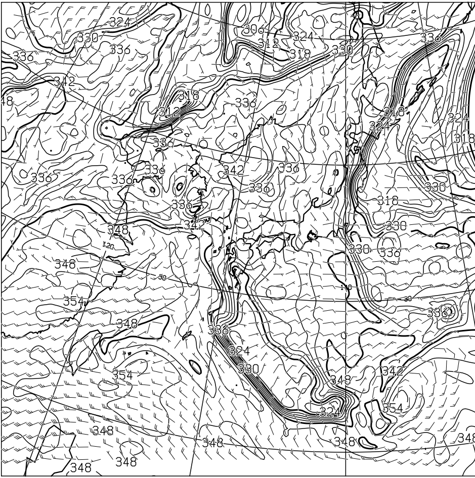
T=12 850hPa: E.P.TEMP(K),WIND(KNOTS) VALID 150000UTC
