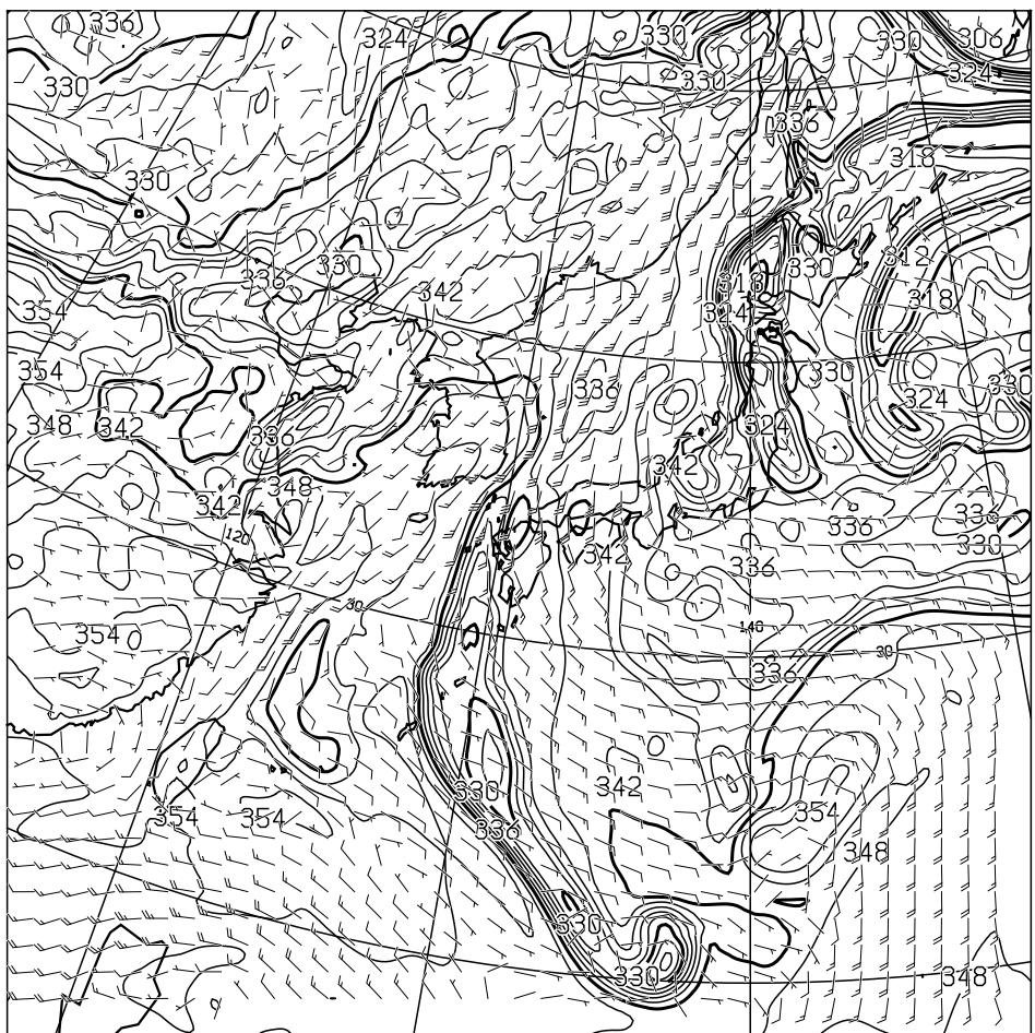
T=48 850hPa: E.P.TEMP(K),WIND(KNOTS) VALID 161200UTC
