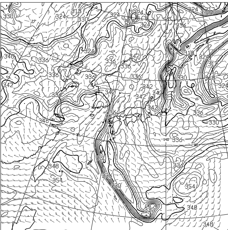
T=36 850hPa: E.P.TEMP(K),WIND(KNOTS) VALID 160000UTC
