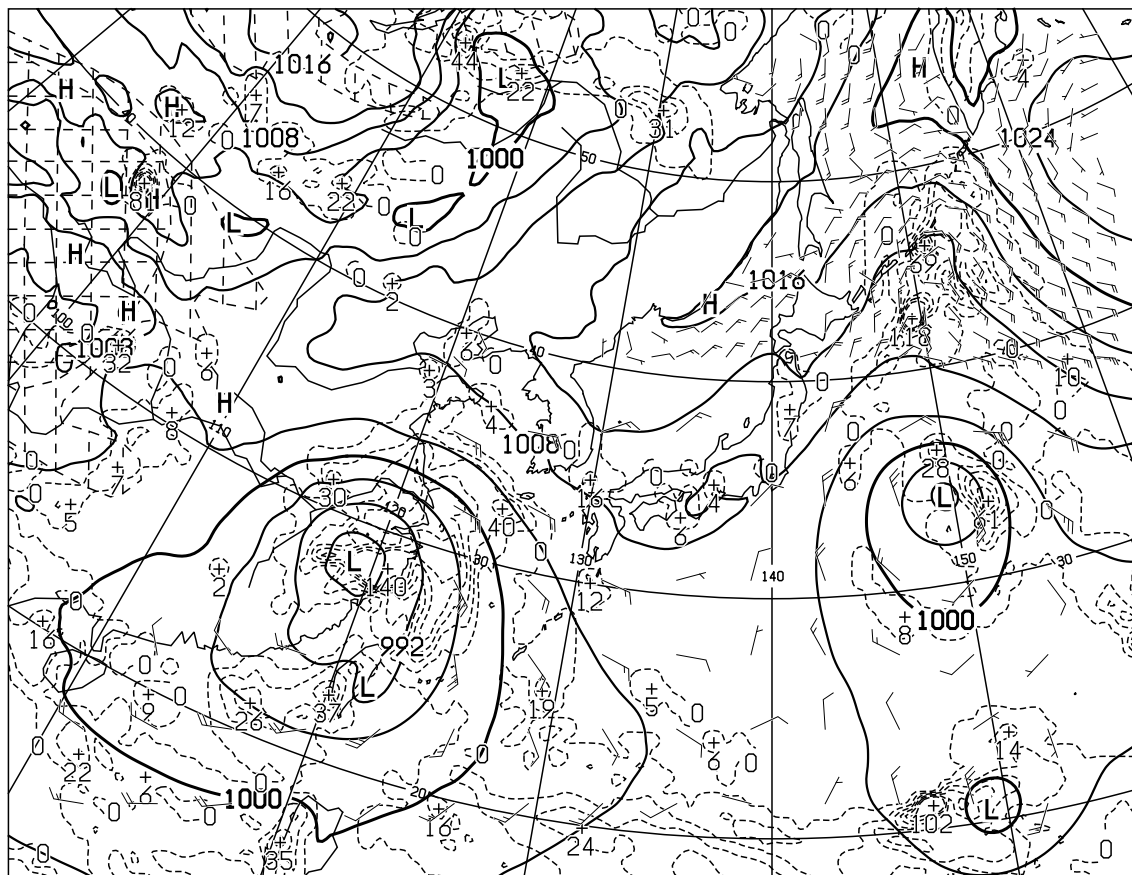
T=12 VALID 100000UTC SURFACE PRESS(hPa), PRECIP(MM) (00-12) WIND ARROW AT SURFACE
