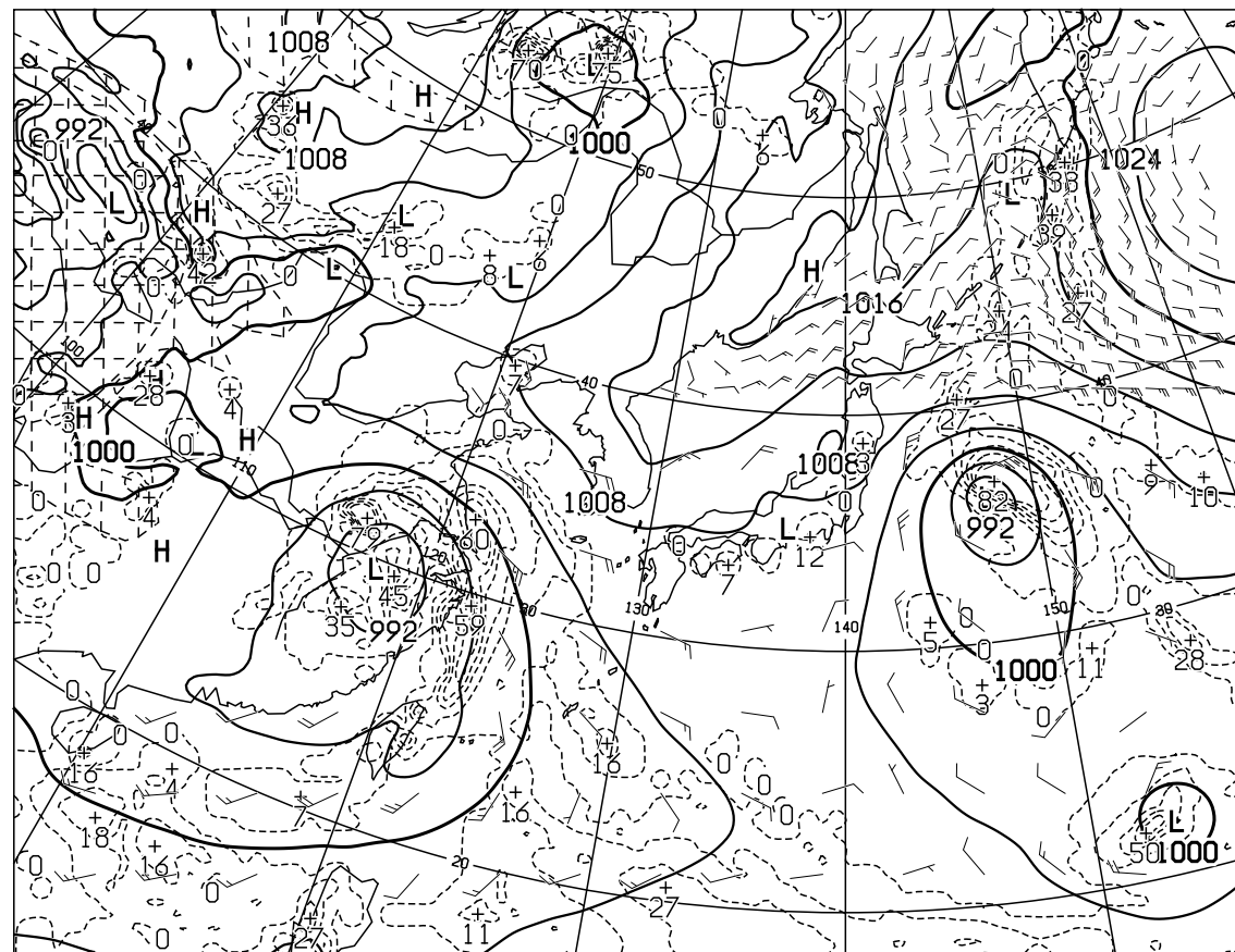
T=24 VALID 101200UTC SURFACE PRESS(hPa), PRECIP(MM) (12-24) WIND ARROW AT SURFACE
