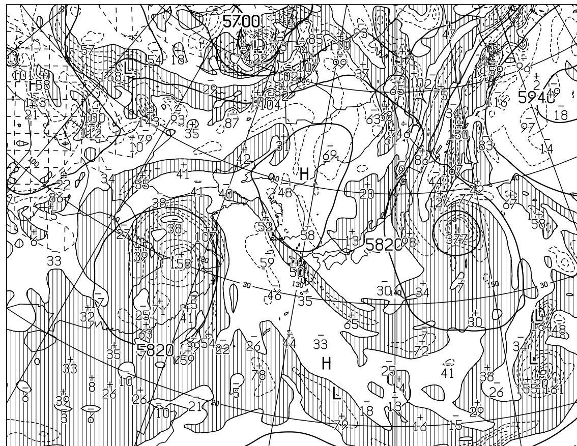
T=24 VALID 101200UTC HEIGHT(M), VORT(10 -6 /SEC) AT 500hPa
