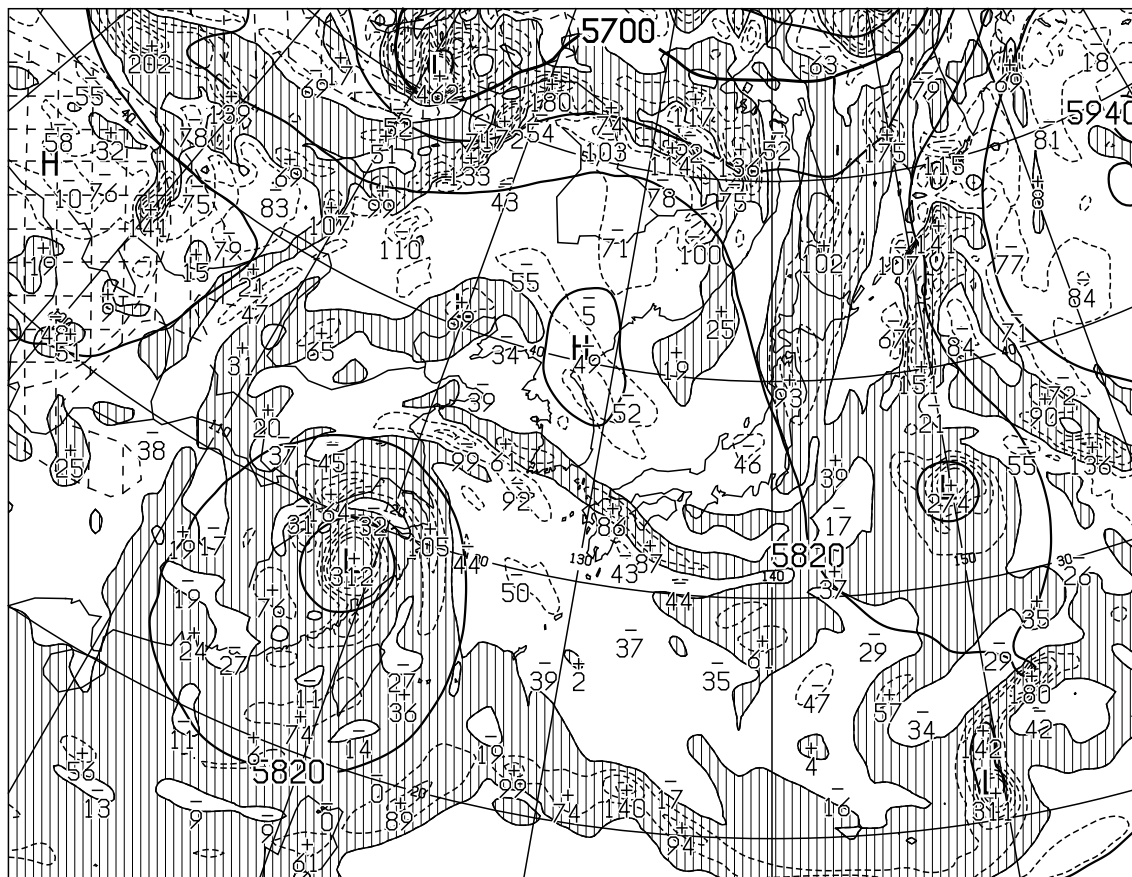
T=12 VALID 100000UTC HEIGHT(M), VORT(10 -6 /SEC) AT 500hPa
