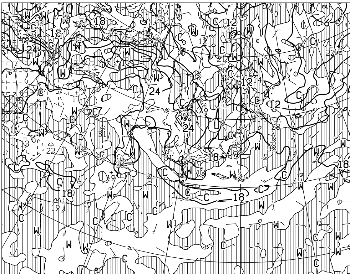
T=12 VALID 290000UTC TEMP( C), WIND ARROW AT 850hPa P-VEL(hPa/H) AT 700hPa
