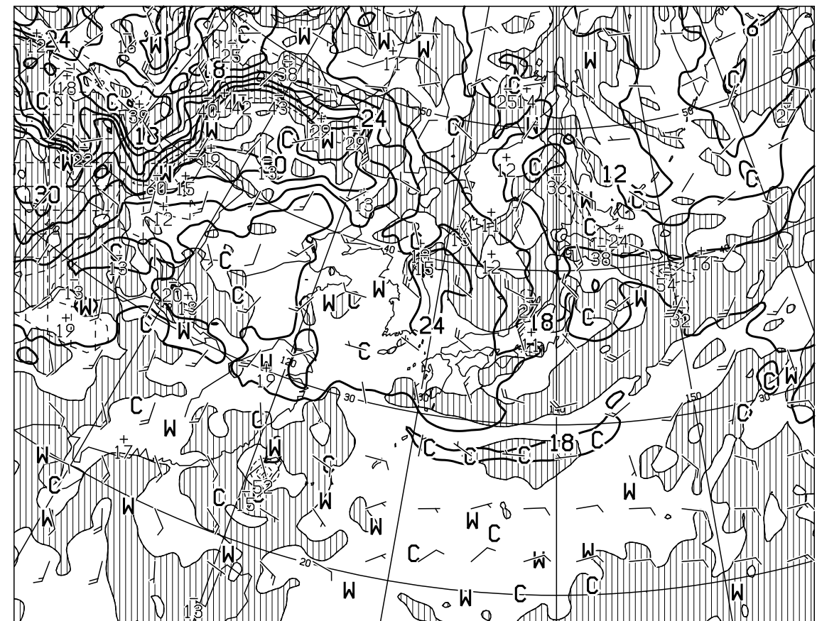
T=24 VALID 291200UTC TEMP( C), WIND ARROW AT 850hPa P-VEL(hPa/H) AT 700hPa
