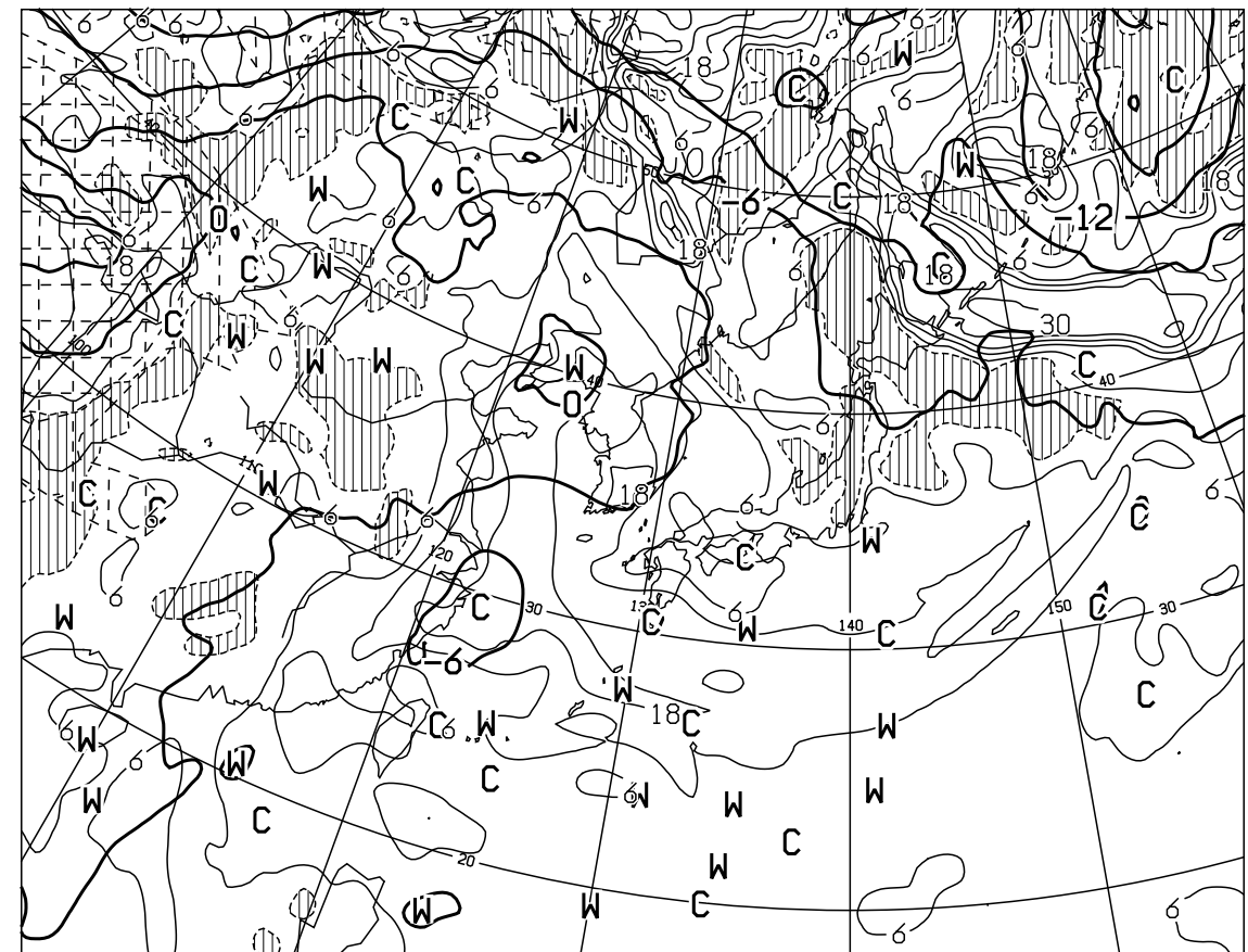
T=24 VALID 291200UTC TEMP( C) AT 500hPa T-TD( C) AT 700hPa
