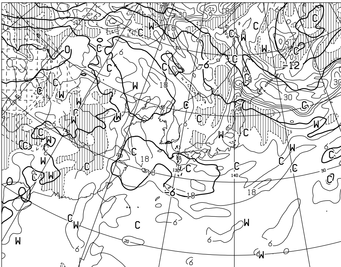
T=12 VALID 290000UTC TEMP( C) AT 500hPa T-TD( C) AT 700hPa
